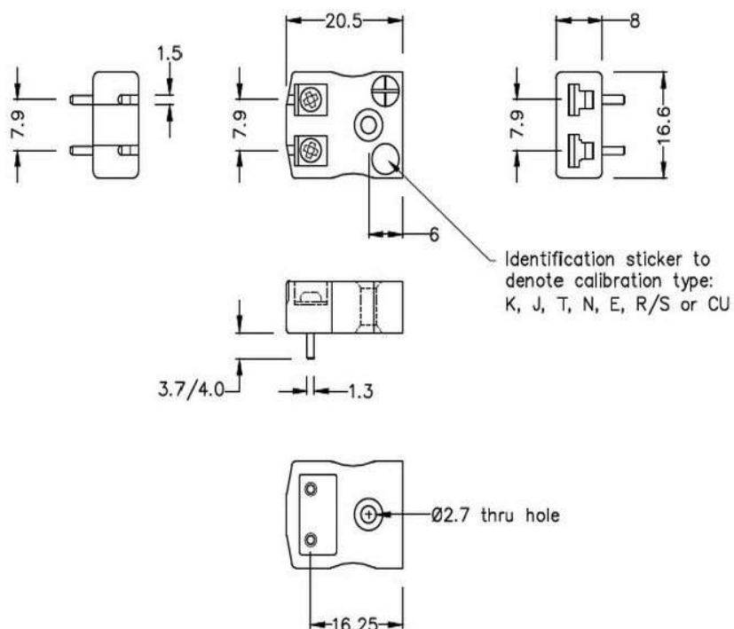
Miniature PCB Socket (dimensions in mm)
