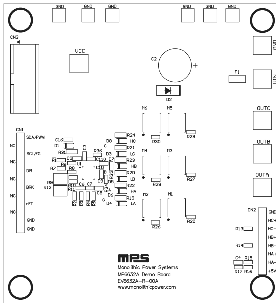
Figure 11: Top Silk
