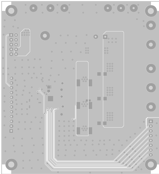
Figure 13: Bottom Layer
