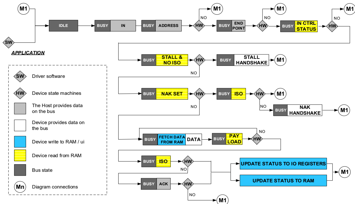
Figure 28-6. IN Transaction
