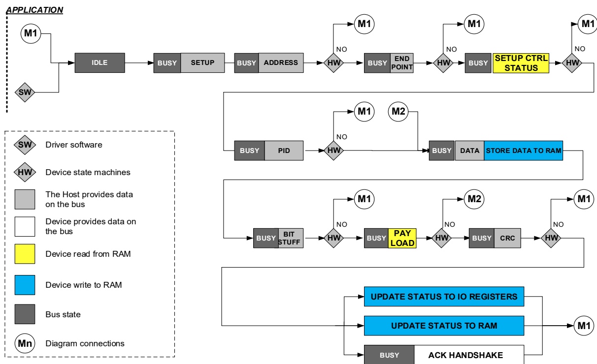
Figure 28-4. SETUP Transaction
