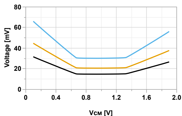
Figure 36-113. Input Hysteresis vs. Common Mode Voltage ( V_{DD} = 2.0V )
