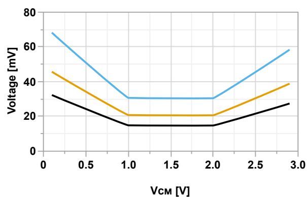
Figure 36-115. Input Hysteresis vs. Common Mode Voltage ( V_{DD} = 3.0V )
