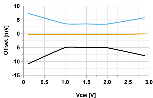
Figure 36-114. Input Offset vs. Common Mode Voltage ( V_{DD} = 3.0V )
