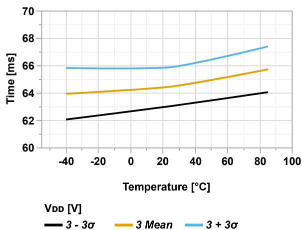
Figure 36-47. Start-up Time vs. Temperature (SYSCFG1 = 0x07, V_{DD} = 3.0V )
