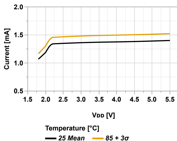
Figure 36-9. Idle Power Consumption vs. V_{DD} (MCLKCTRLA.CLKSEL = OSCHF, OSCHF = 24 MHz)
