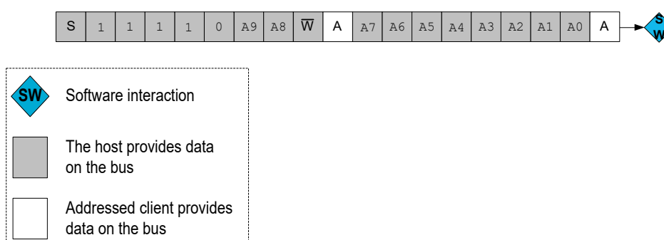
Figure 27-9. 10-Bit Address Transmission
