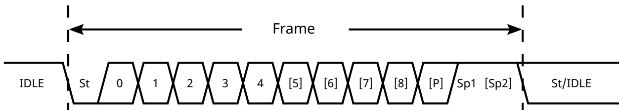
Figure 25-2. Frame Formats
