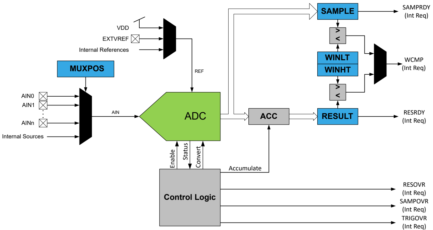
Figure 32-1. Block Diagram
