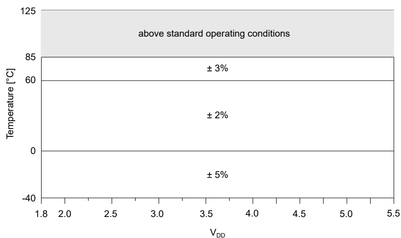
Figure 35-2. Precision Calibrated OSCHF ( f_{\text{OSCHF}} \geq 4\text{ MHz} ) Frequency Accuracy Over Device V_{\text{DD}} and Temperature (1)
