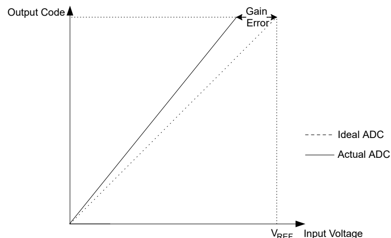
Figure 4-2. Gain Error
