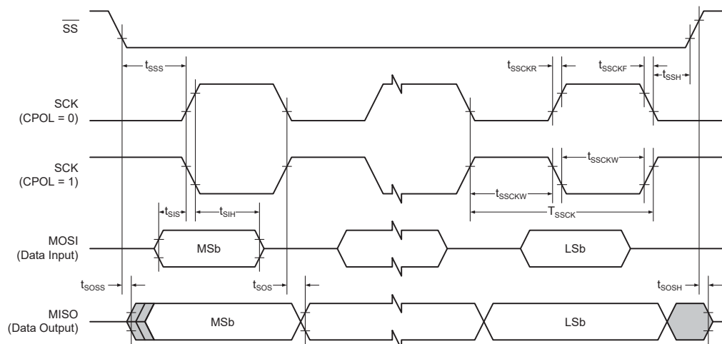
Figure 35-6. SPI - Timing Requirements in Client Mode
