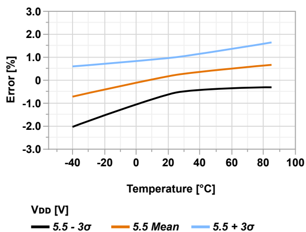
Figure 36-90. ACREF Voltage Error vs. Temperature ( V_{DD} = 5.5V , V_{VREF} = 2.048V )
