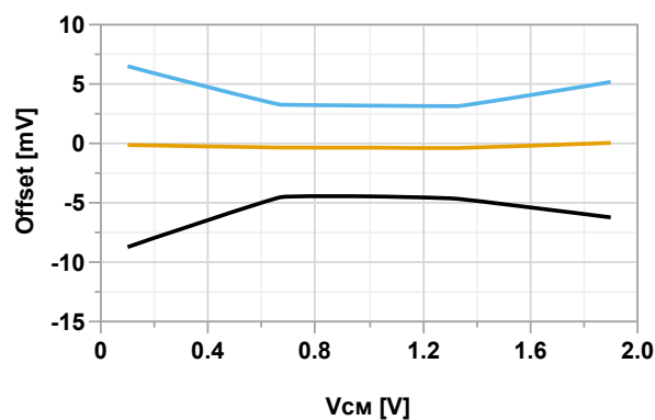
Figure 36-112. Input Offset vs. Common Mode Voltage ( V_{DD} = 2.0V )
