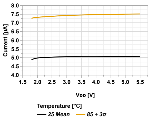
Figure 36-5. Active Power Consumption vs. V_{DD} (MCLKCTRLA.CLKSEL = OSC32K)
