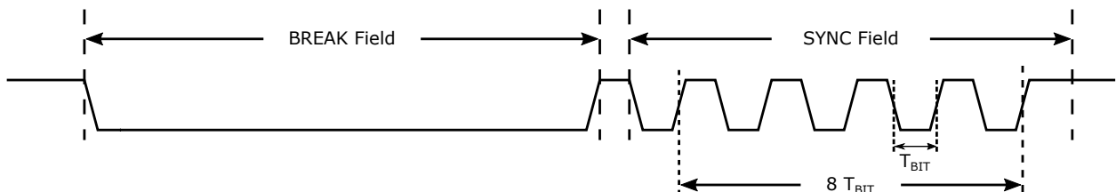
Figure 25-9. Auto-Baud Timing
