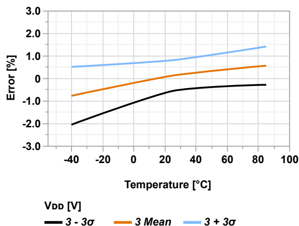
Figure 36-86. ADCOREF Voltage Error vs. Temperature ( V_{DD} = 3.0V , V_{VREF} = 2.5V )
