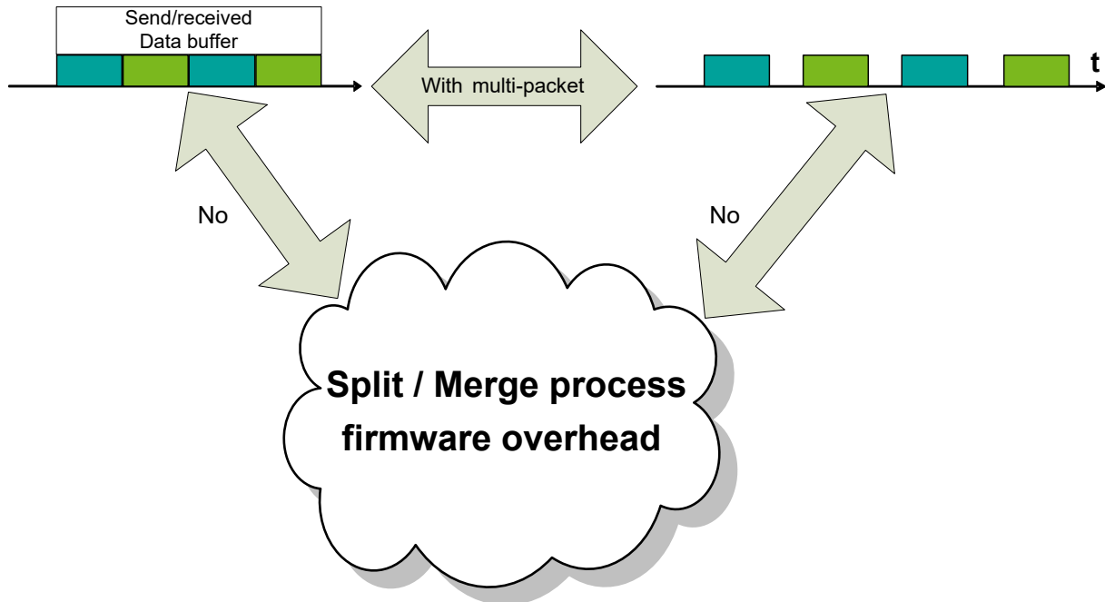
Figure 28-8. Multi-packet Reduces CPU Load
