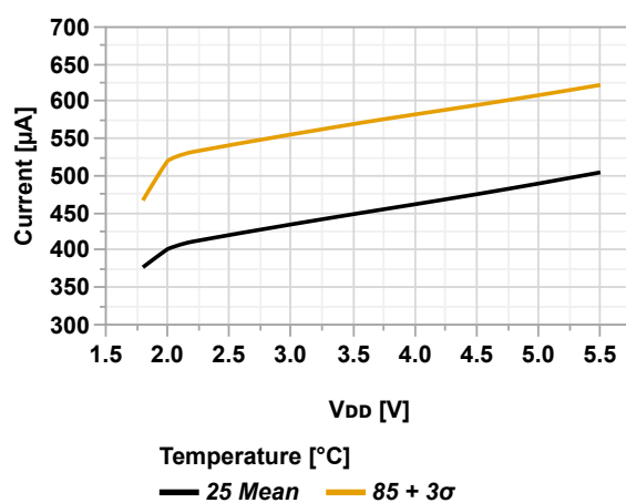
Figure 36-21. ADC Power Consumption vs. V_{DD} (ADC @170 kps)
