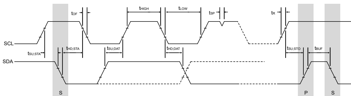
Figure 35-7. TWI - Timing Requirements
