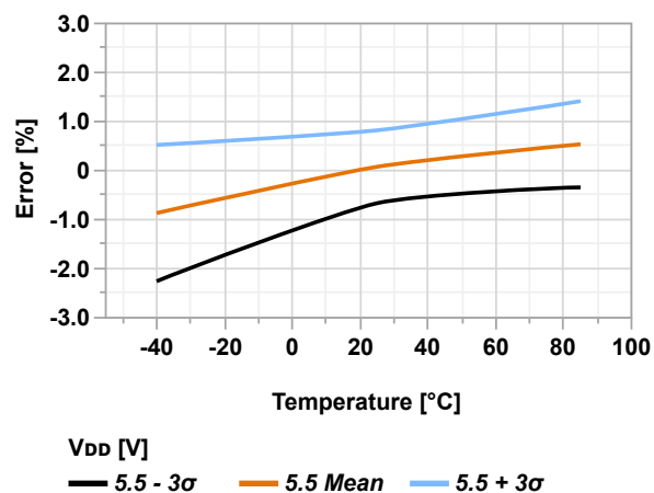
Figure 36-87. ADCOREF Voltage Error vs. Temperature ( V_{DD} = 5.5V , V_{VREF} = 4.096V )
