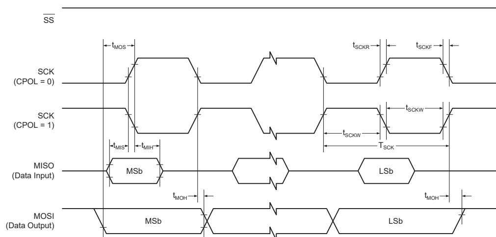
Figure 35-4. USART in SPI Mode - Timing Requirements in Host Mode
