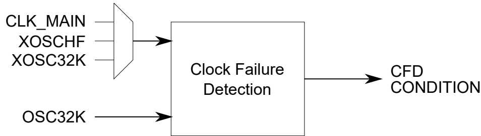
Figure 12-5. Clock Failure Detection (CFD) Block Diagram
