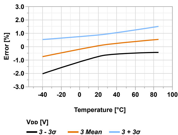
Figure 36-91. ACREF Voltage Error vs. Temperature ( V_{DD} = 3.0V , V_{VREF} = 2.048V )
