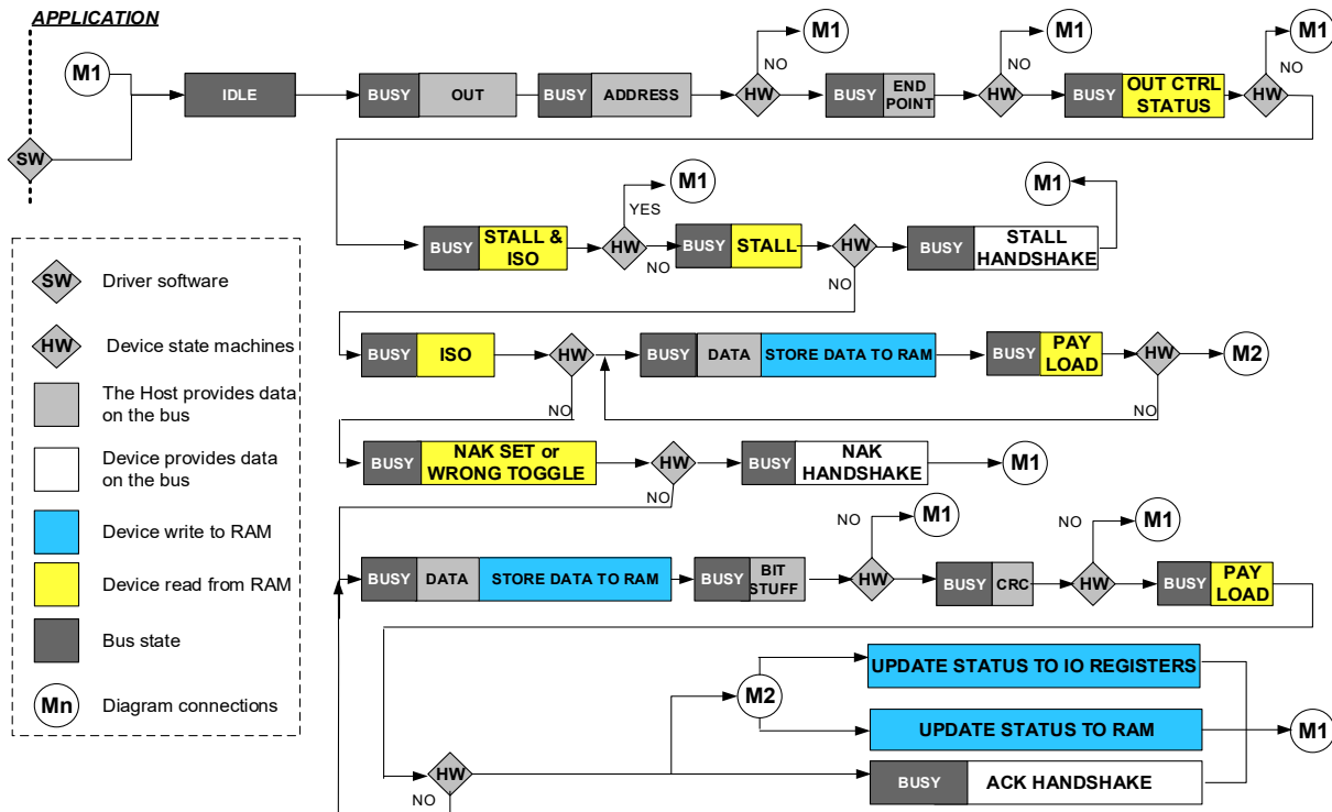
Figure 28-5. OUT Transaction
