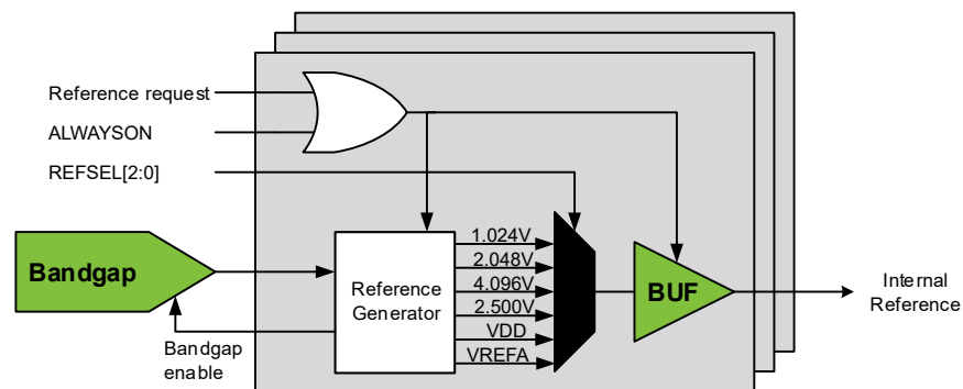
Figure 20-1. VREF Block Diagram
