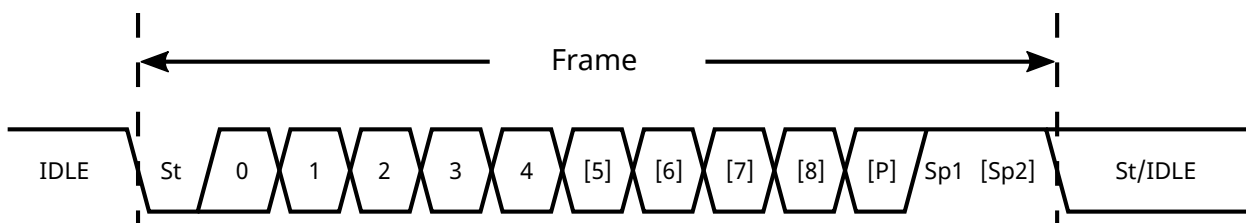
Figure 25-2. Frame Formats
