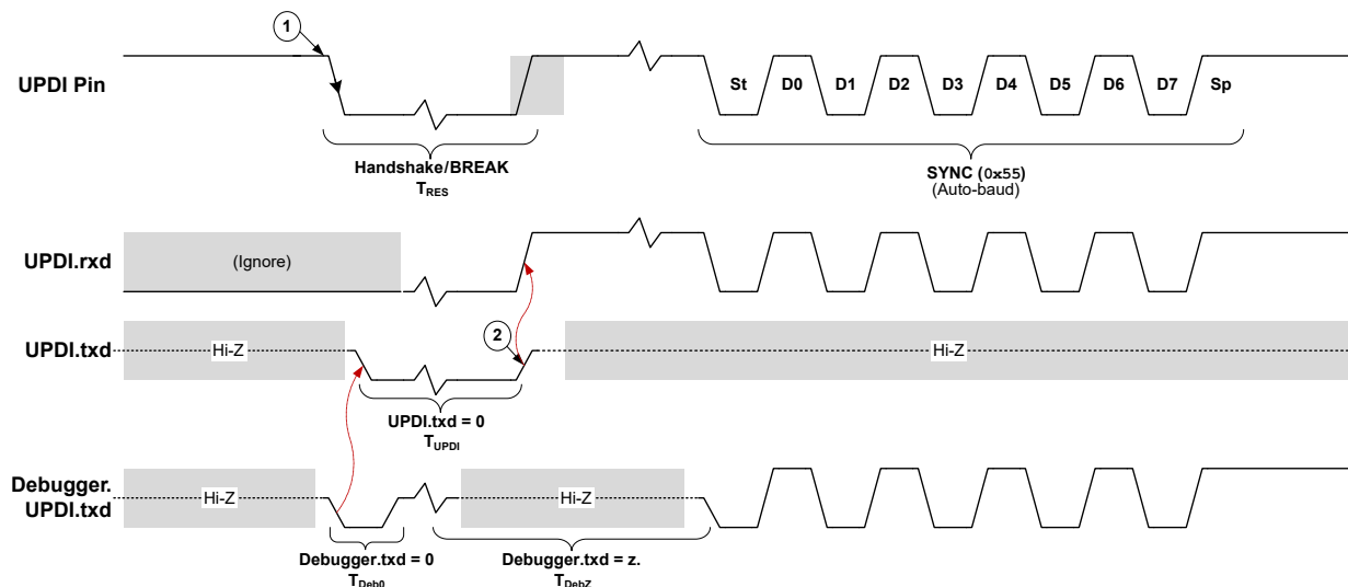
1 Drive low from the debugger to request the UPDI clock. 2 UPDI clock ready; Communication channel ready.
