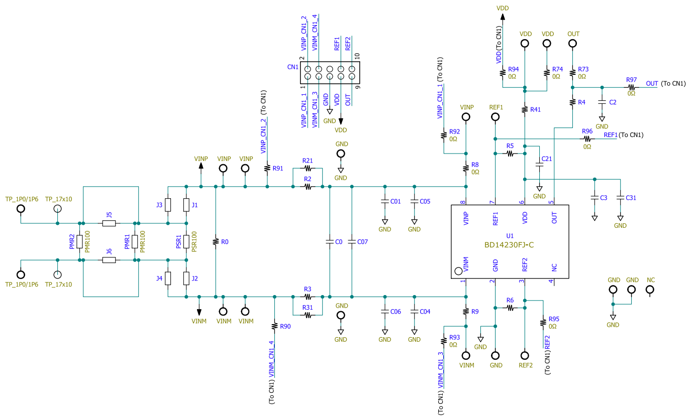
Figure 2. Schematic of the BD14230FJ-EVK-001
