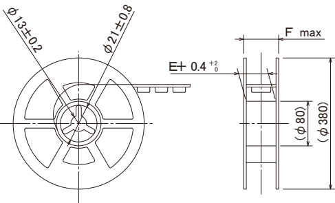
Reel Diagram
