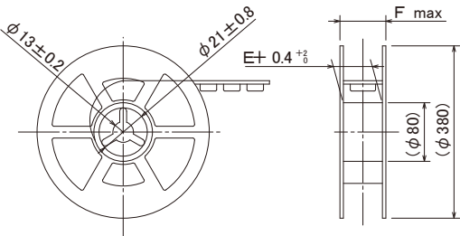
Reel Diagram
