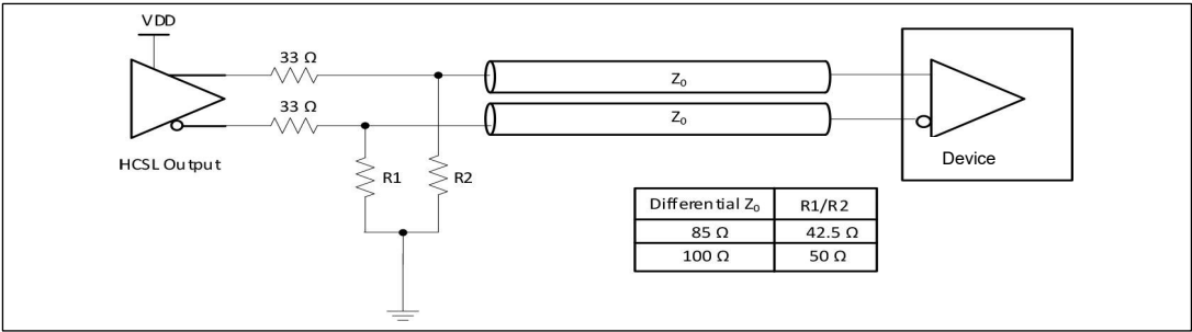
FIGURE 3- 2: INPUT DRIVEN BY AN HCSL OUTPUT.
