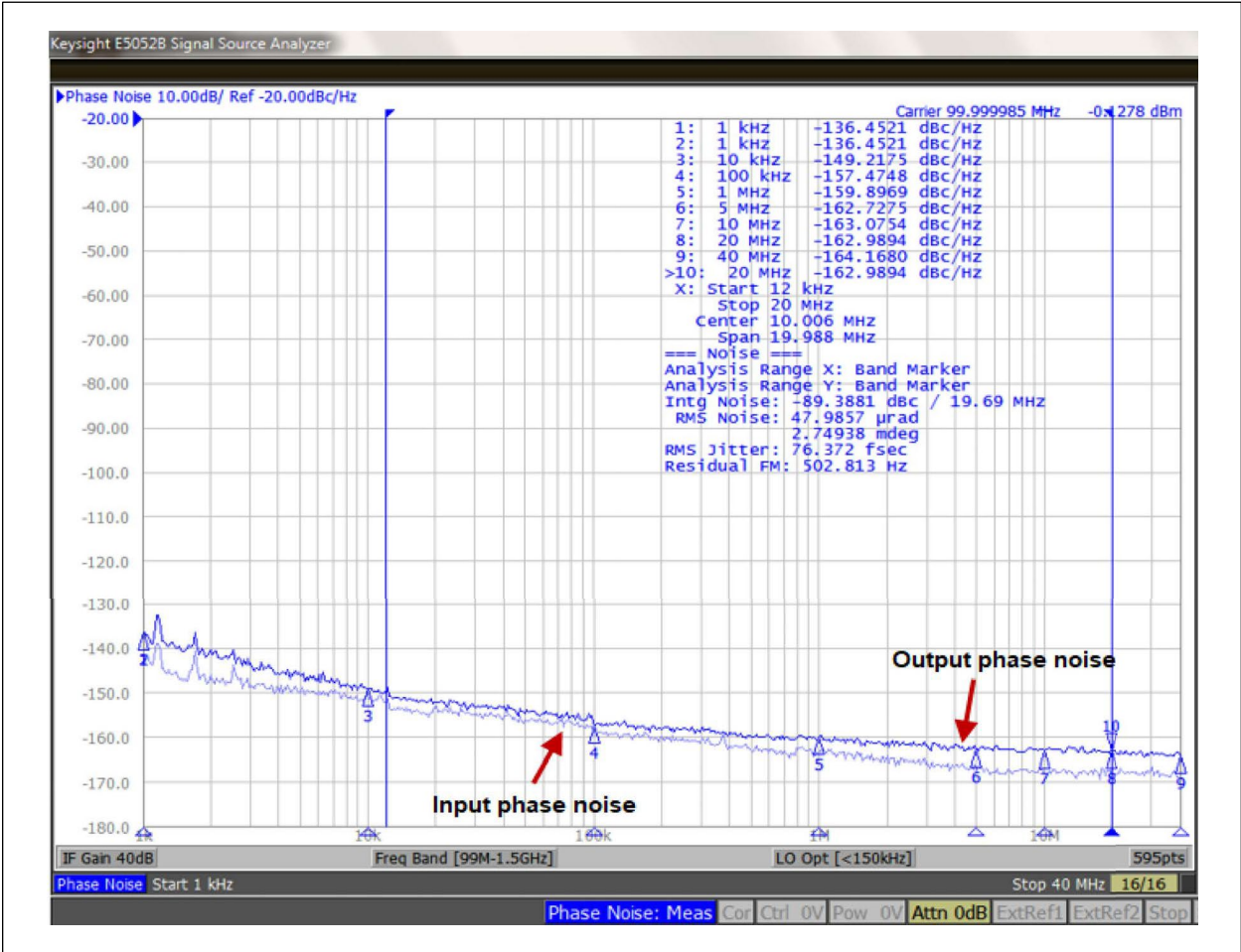
FIGURE 3- 15: TYPICAL PHASE NOISE.
