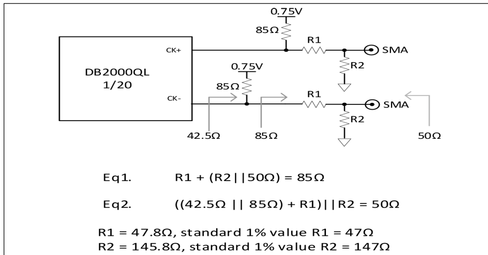
FIGURE 5- 1: DC TEST LOAD (AS PER DB2000QL).
