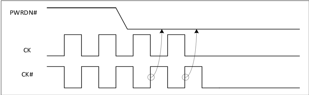
FIGURE 3- 6: PWRDN# ASSERTION
