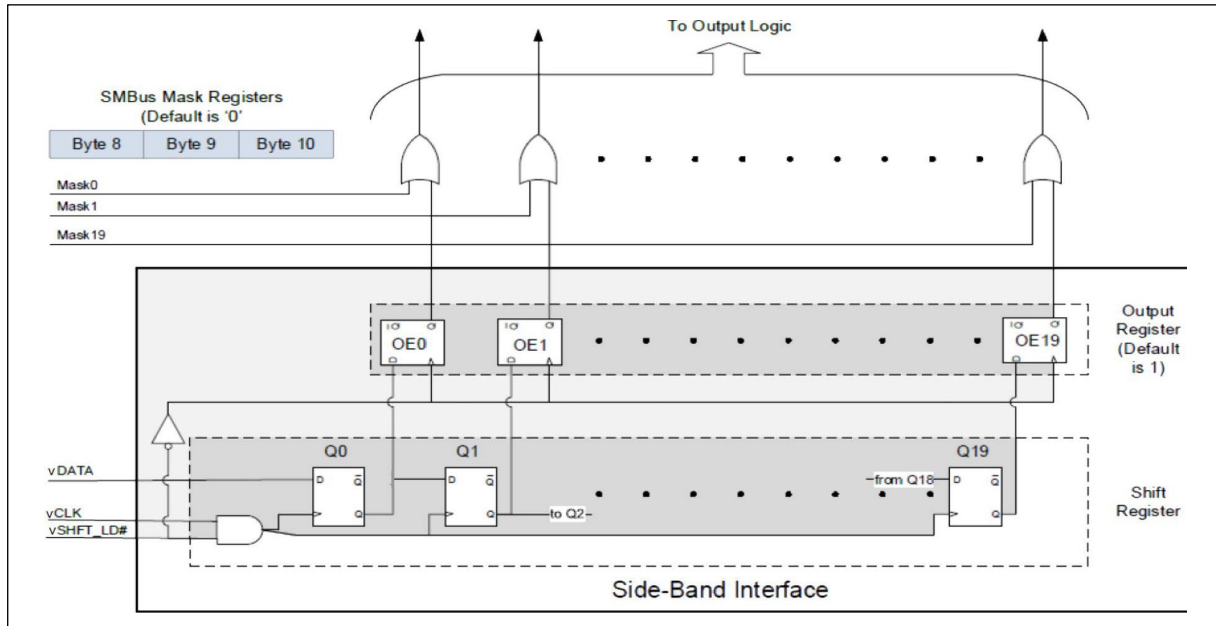
FIGURE 3- 13: SIDE-BAND INTERFACE CONTROL LOGIC (FUNCTIONAL DESCRIPTION).
