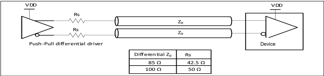
FIGURE 3- 1: INPUT DRIVEN BY A PUSH-PULL DIFFERENTIAL OUTPUT.
