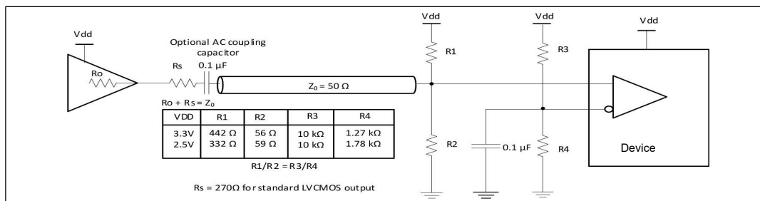
FIGURE 3- 3: INPUT DRIVEN BY A SINGLE ENDED OUTPUT.
