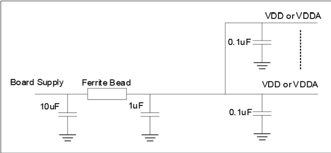
FIGURE 3- 5: POWER SUPPLY FILTERING.
