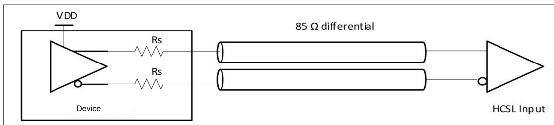
FIGURE 3- 4: TERMINATING DIFFERENTIAL OUTPUTS.
