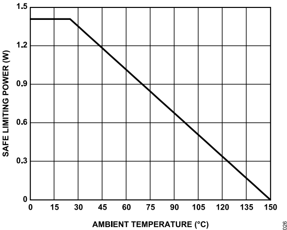
Figure 6. Thermal Derating Curve for 16-Lead QSOP (RQ-16), Dependence of Safety Limiting Power with Ambient Temperature per IEC 60747-17
