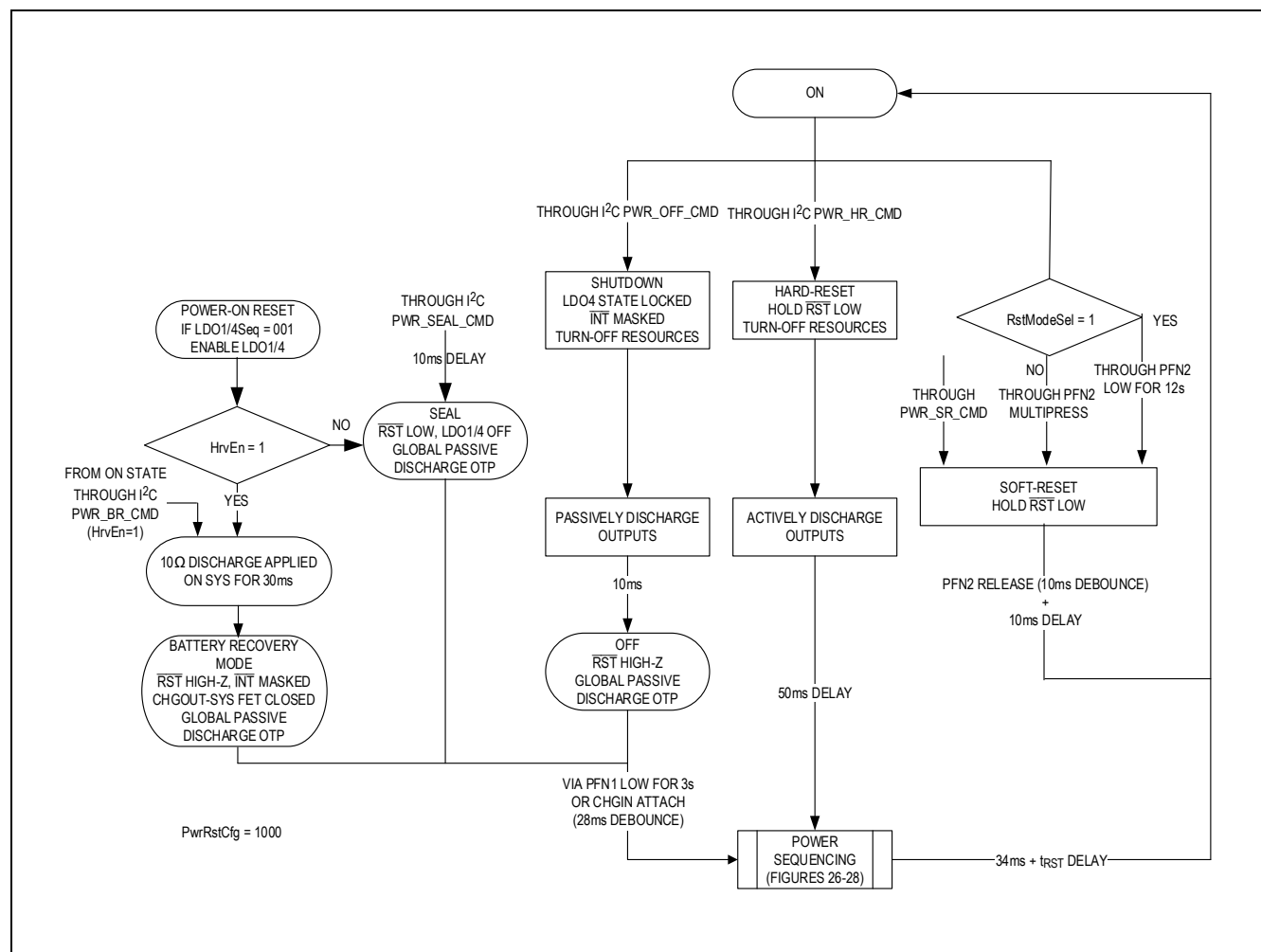
Figure 18. PwrRstCfg 1000
