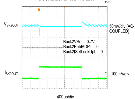
BUCK2 LOAD TRANSIENT
