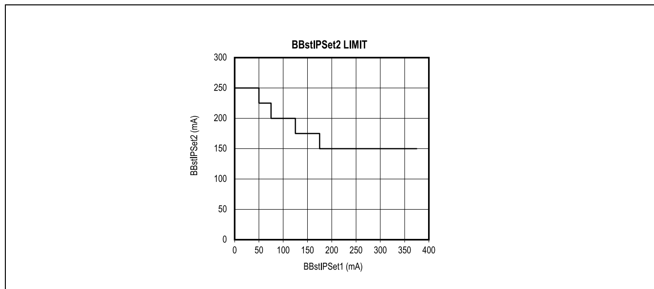
Figure 9. Minimum BBstIPSet2 Limit for a Given BBstIPSet1 Setting
