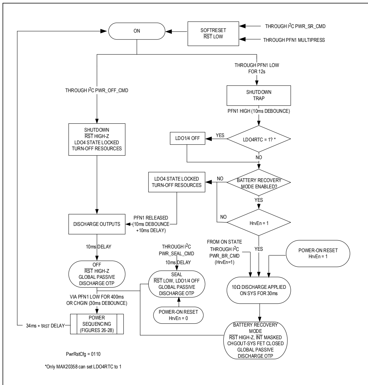
Figure 16. PwrRstCfg 0110
