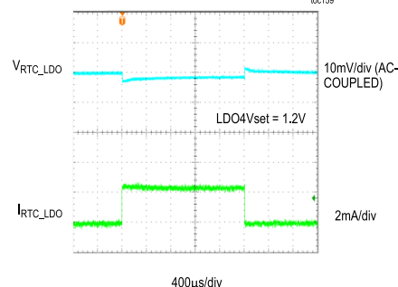
RTC LDO LOAD TRANSIENT
