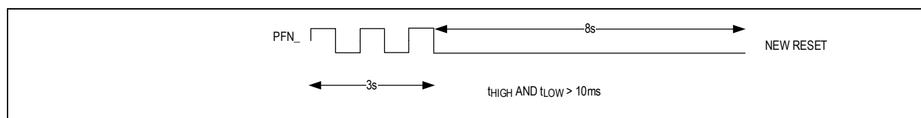
Figure 25. Reset Using PFN_
