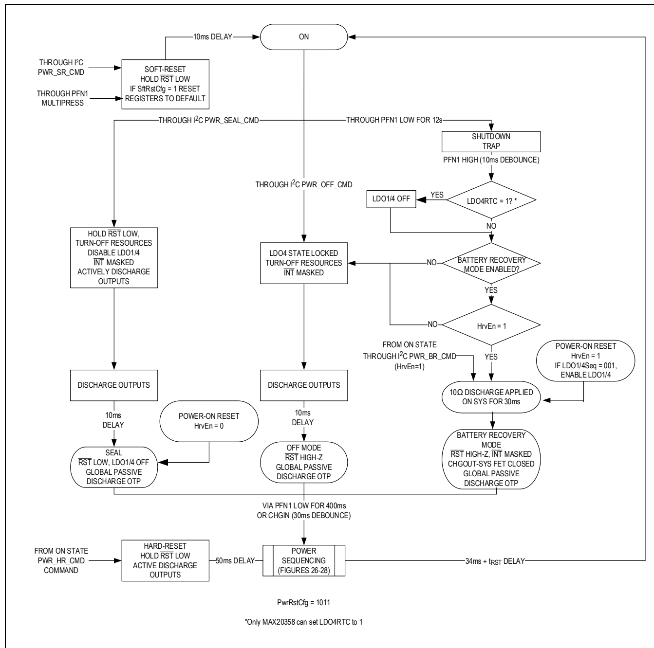
Figure 20. PwrRstCfg 1011
