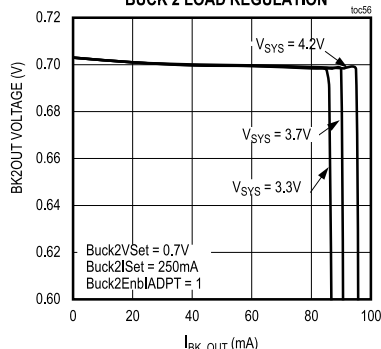
BUCK 2 LOAD REGULATION
