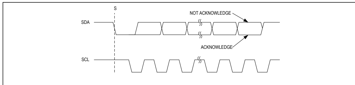
Figure 40. Acknowledge Bits
