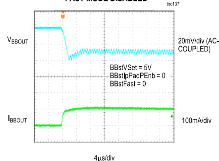
BUCK-BOOST LOAD TRANSIENT FAST MODE DISABLED
