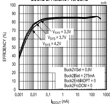
BUCK2 EFFICIENCY vs. LOAD
