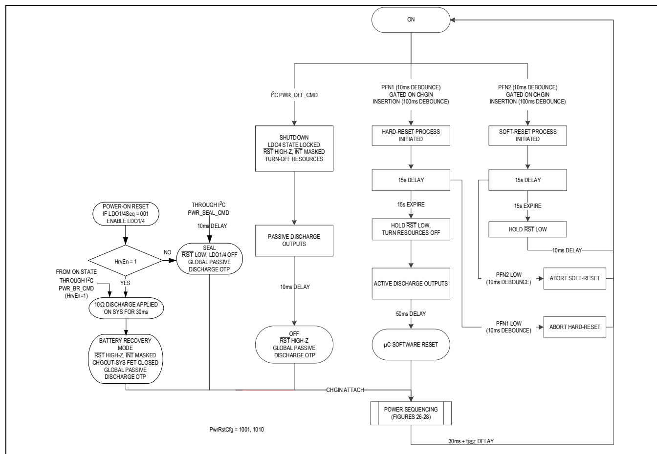
Figure 19. PwrRstCfg 1001, 1010
