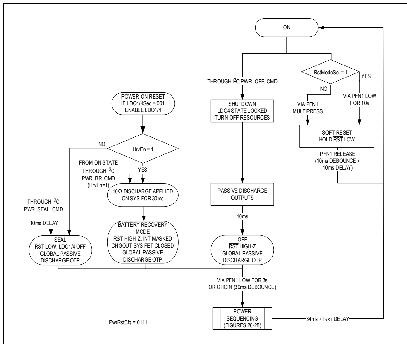
Figure 17. PwrRstCfg 0111
