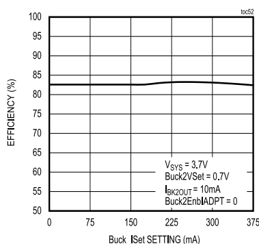
BUCK2 EFFICIENCY vs. Buck_ISet SETTING
