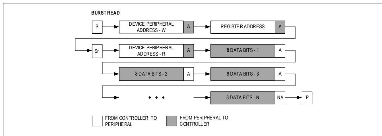
Figure 39. Burst-Read Sequence
