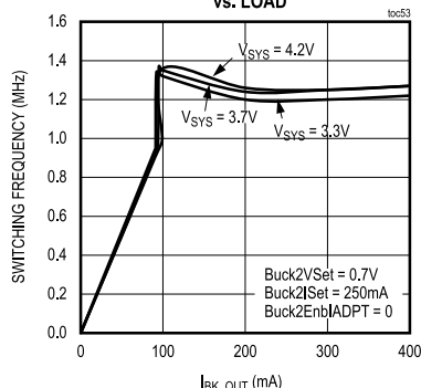
BUCK 2 SWITCHING FREQUENCY vs. LOAD
