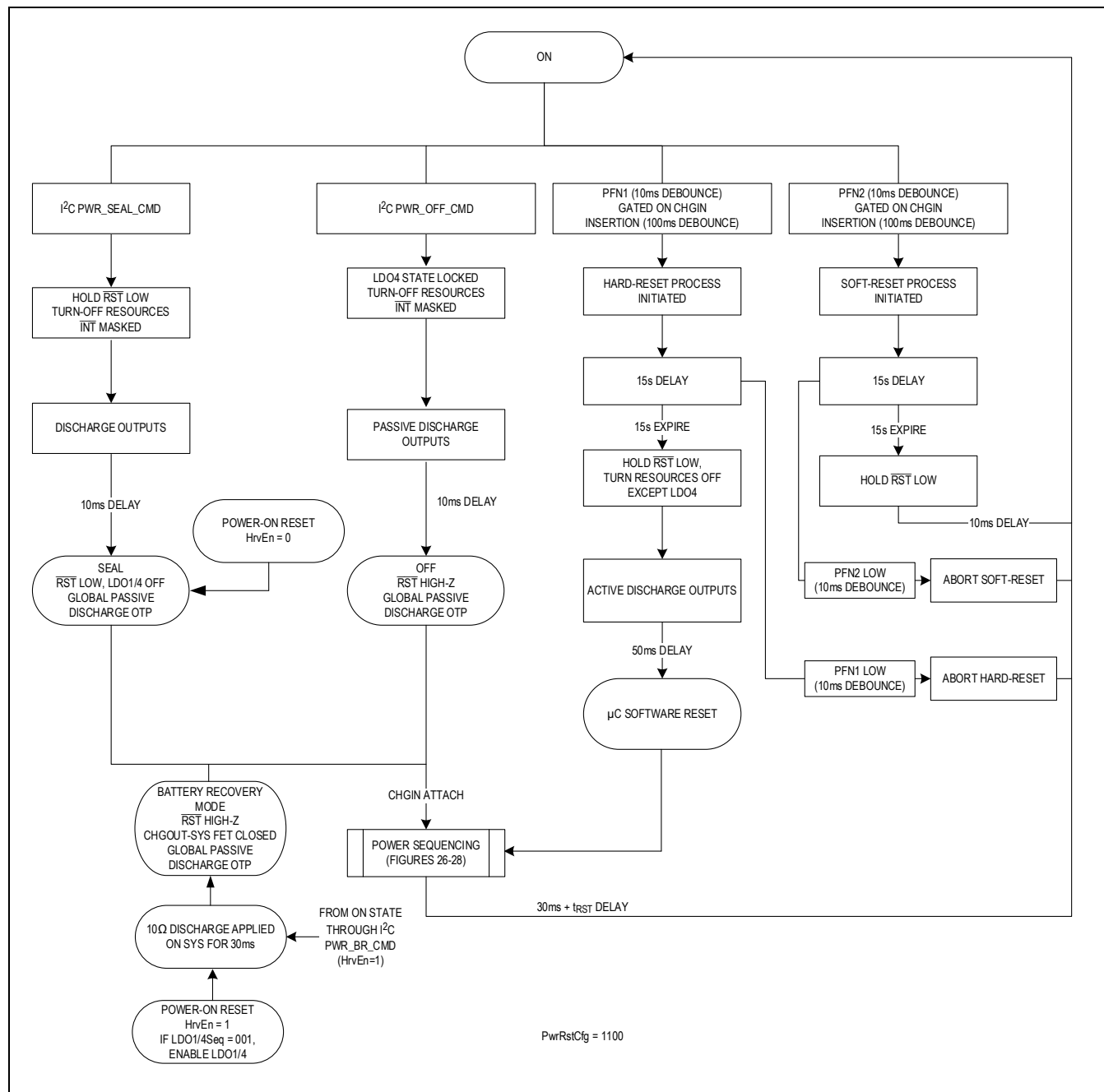
Figure 21. PwrRstCfg 1100
