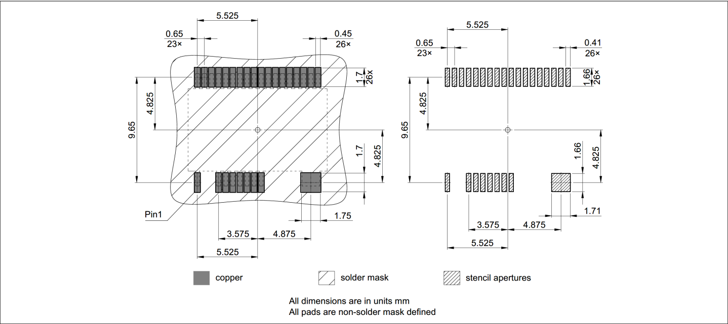
Figure 12 Footprint PG-DSO-21-1
