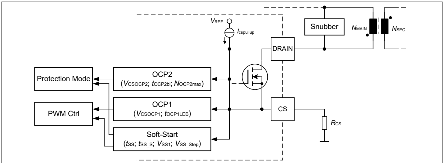
Figure 6 Primary current sensing at CS pin
