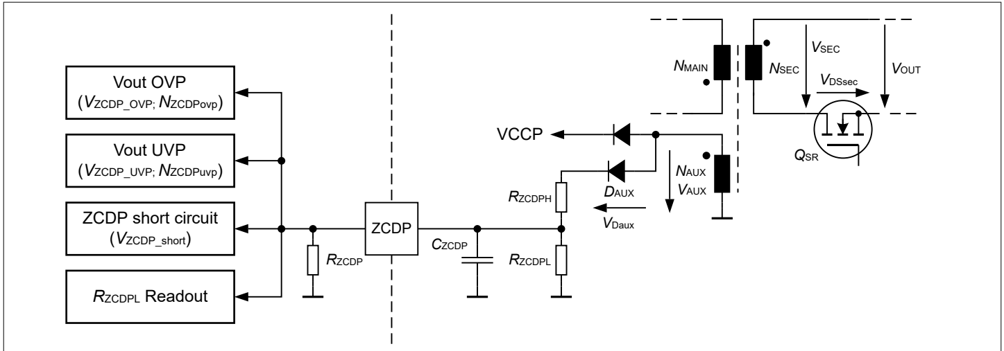
Figure 7 Primary ZCDP pin sensing
