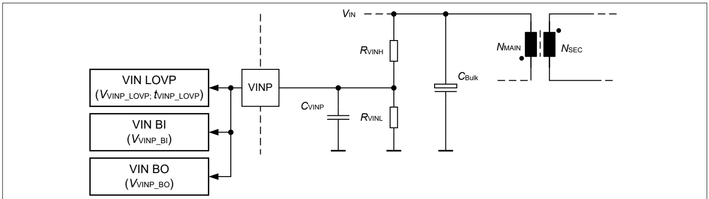
Figure 5 VINP pin sensing
