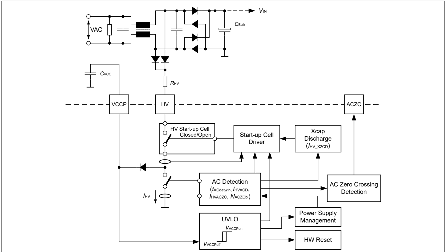
Figure 3 HV sensing circuitry for AC zero crossing detection and X2 capacitor discharge function
