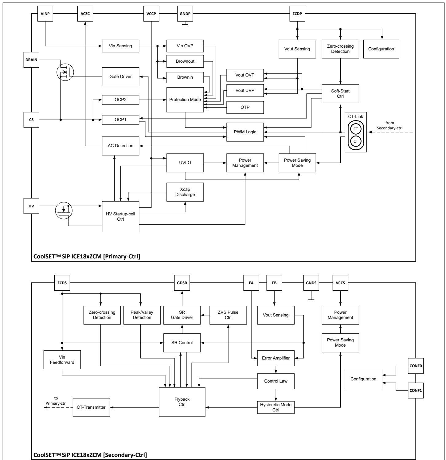
Figure 2 Block diagram CoolSET™ SiP ICE18xZCM
