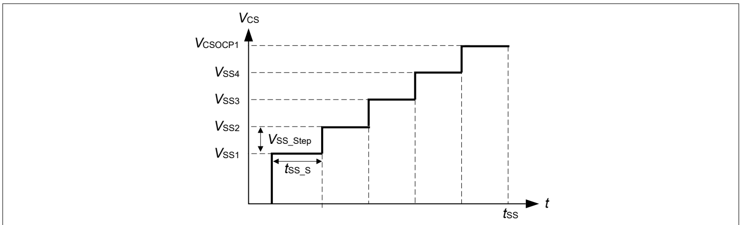
Figure 8 Maximum current sense voltage during soft-start
