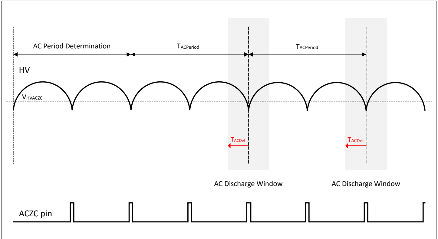
Figure 4 AC zero crossing detection
