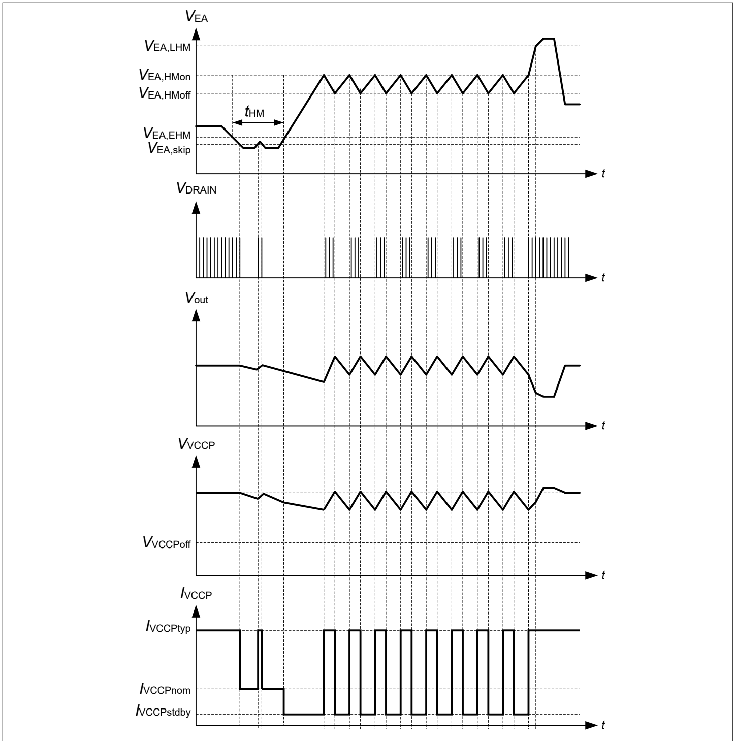
Figure 9 Typical signals for entering, during and exiting hysteretic mode
