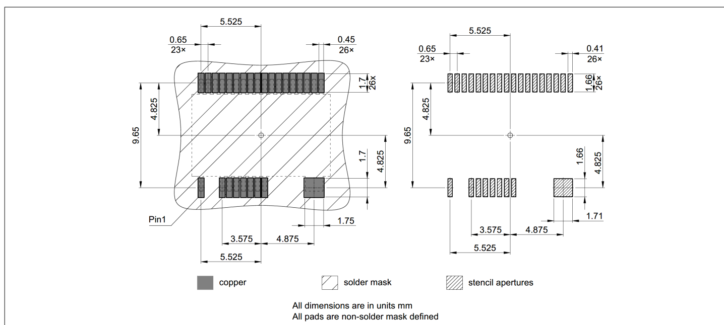
Figure 12 Footprint PG-DSO-21-1
