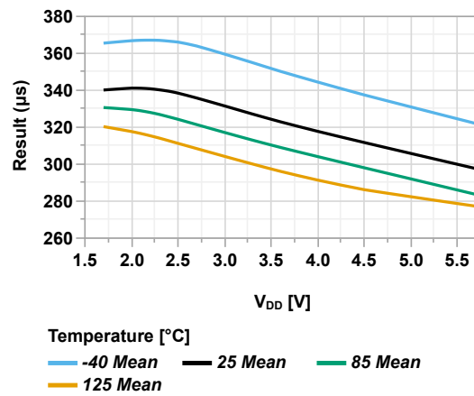
Figure 45-75. LFO Oscillator Start-Up Time vs V_{DD}
