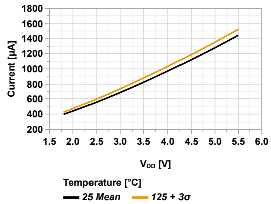
Figure 45-30. I_{DD} vs V_{DD} (Idle Mode, HFINTOSC = 16 MHz, PMDx = 0xFF)
