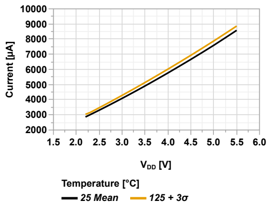
Figure 45-25. I_{DD} vs V_{DD} (ECH = 32 MHz, PMDx = 0x00)
