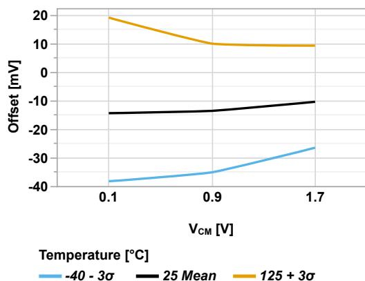
Figure 45-161. Input Offset vs Common-Mode Voltage ( V_{DD} = 3.0V )
