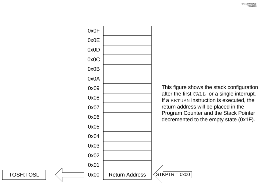
Figure 9-16. Accessing the Stack Example 2
