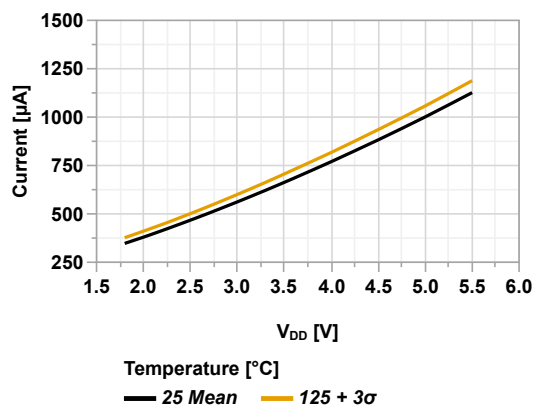
Figure 45-8. I_{DD} vs V_{DD} (HFINTOSC = 8 MHz, PMDx = 0xFF)
