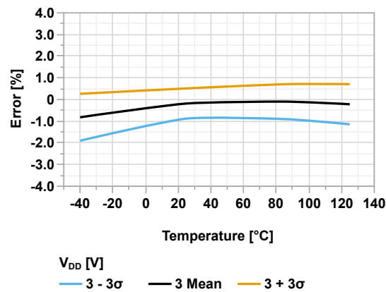
Figure 45-173. ADFVR Voltage Error vs Temperature ( V_{DD} = 3.0\text{V} , V_{REF} = 1.024\text{V} )
