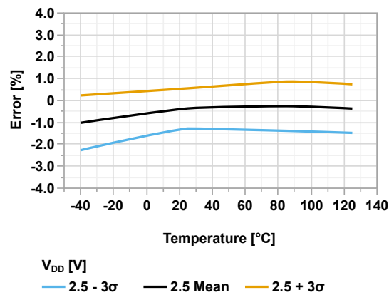
Figure 45-172. ADFVR Voltage Error vs Temperature ( V_{DD} = 2.5\text{V} , V_{REF} = 1.024\text{V} )
