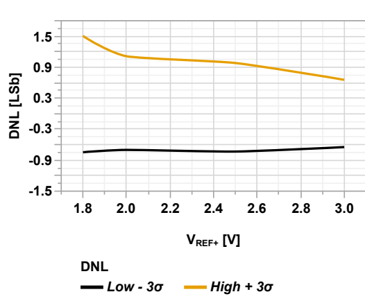
Figure 45-96. ADC DNL vs V_{REF+} (Single-Ended Mode, T_{AD} = 1 \mu s , V_{DD} = 3.0V , T_A = 125^{\circ}C , CPON = 'b11')
