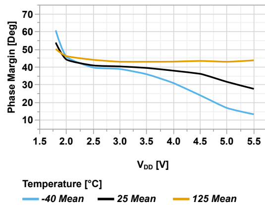
Figure 45-139. Phase Margin vs V_{DD} (CPON = '0', GSEL = 'b001')
