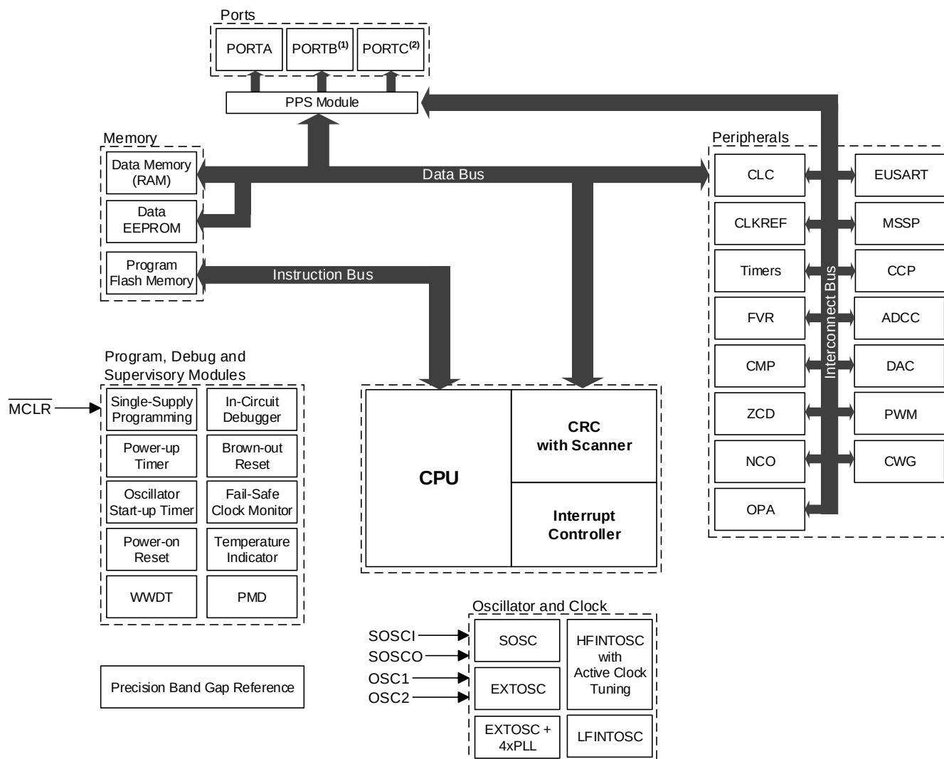
Figure 1. PIC16F17114/15/24/25/44/45 Block Diagram
