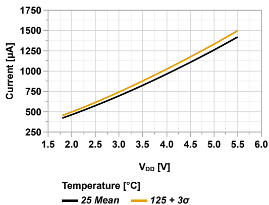
Figure 45-7. I_{DD} vs V_{DD} (HFINTOSC = 8 MHz, PMDx = 0x00)
