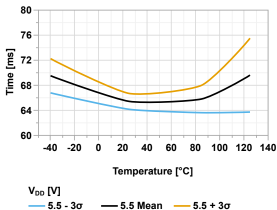
Figure 45-88. Start-Up Time vs Temperature (PWRTS = 'b10, V_{DD} = 5.5V )
