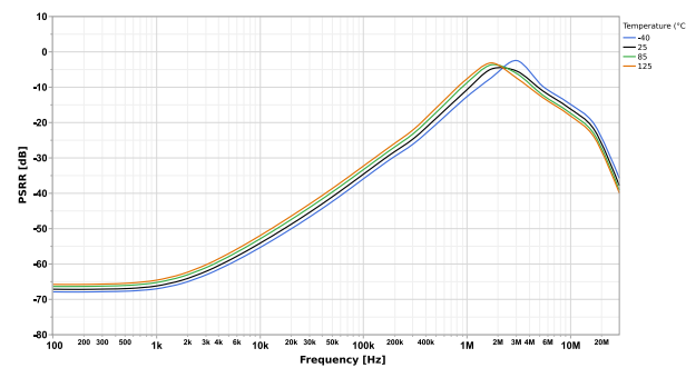
Figure 45-122. OPA PSRR (log(f) vs PSRR (dB) over Temperature)
