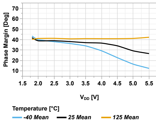
Figure 45-138. Phase Margin vs V_{DD} (CPON = '1', GSEL = 'b001')
