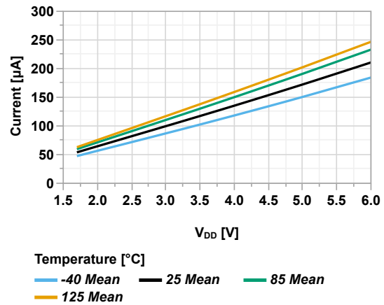
Figure 45-67. Weak Pull-Up Current vs V_{DD} (Mean Values)
