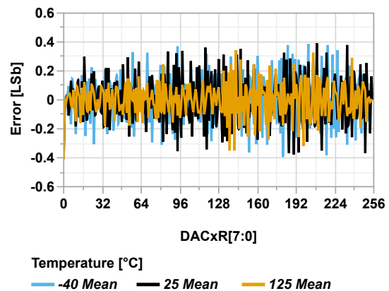
Figure 45-108. DAC DNL vs. DAC Code ( V_{REF} = V_{DD} = 5.5V )
