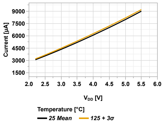
Figure 45-11. I_{DD} vs V_{DD} (HFINTOSC = 32 MHz, PMDx = 0x00)
