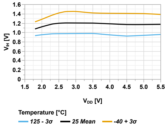
Figure 45-56. Input Pin with SMBus 3.0 Minimum V_{IH} vs V_{DD}
