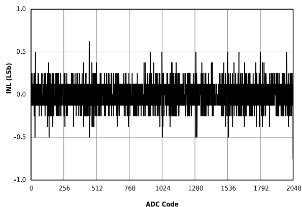
Figure 45-97. ADC INL vs ADC Code (Single-Ended Mode, V_{DD} = 3.0V , T_{AD} = 1 \mu s )
