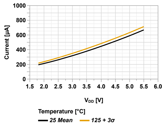
Figure 45-1. I_{DD} vs V_{DD} (HFINTOSC = 1 MHz, PMDx = 0x00)
