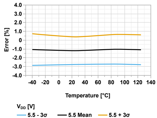
Figure 45-181. CDAFVR Voltage Error vs Temperature ( V_{DD} = 5.5V , V_{REF} = 1.024V )
