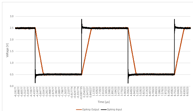
Figure 45-121. OPA Small Signal
