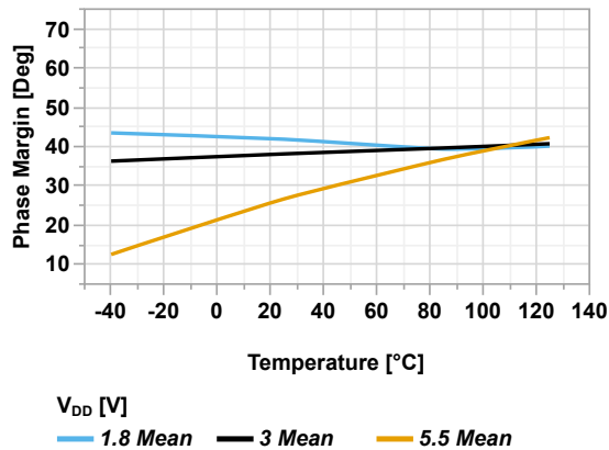
Figure 45-134. Phase Margin vs Temperature (CPON = '1', GSEL = 'b001')
