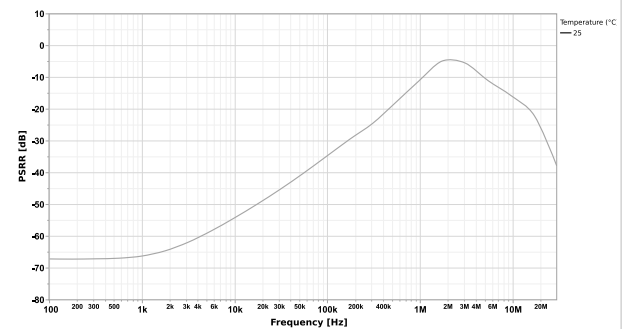
Figure 45-123. OPA PSRR (log(f) vs PSRR (dB) (Typical))
