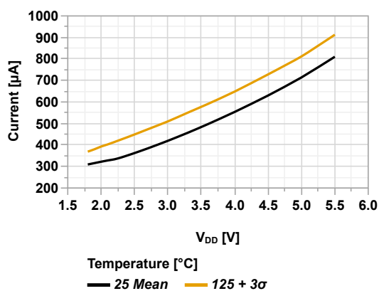
Figure 45-45. I_{PD} Op Amp (CPON = 'b11) vs V_{DD}
