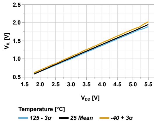
Figure 45-53. Input Pin with Schmitt Trigger Maximum V_{IL} vs V_{DD}
