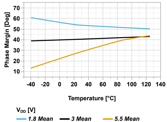
Figure 45-135. Phase Margin vs Temperature (CPON = '0', GSEL = 'b001')
