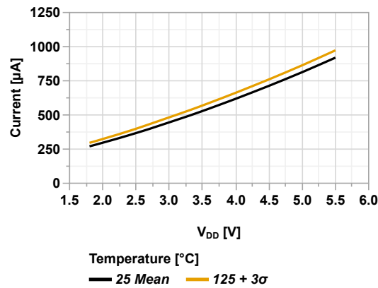
Figure 45-3. I_{DD} vs V_{DD} (HFINTOSC = 2 MHz, PMDx = 0x00)
