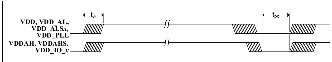
FIGURE 5-1: POWER SEQUENCE TIMING
