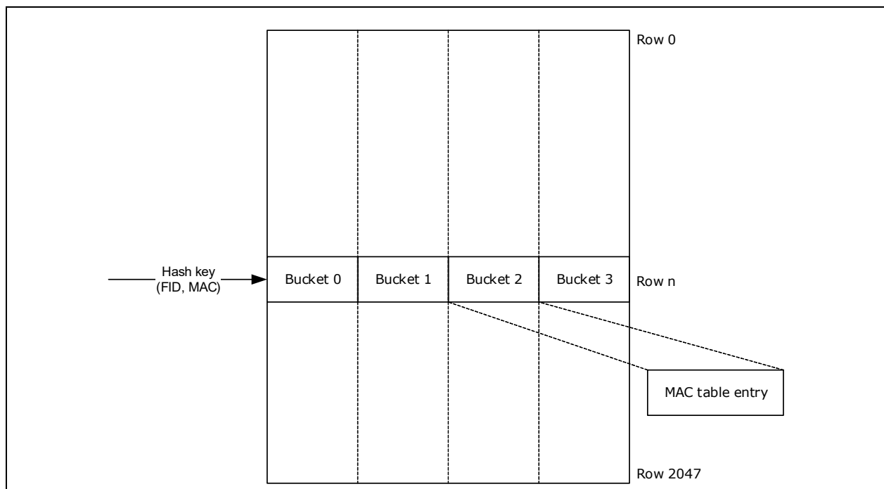
FIGURE 4-10: MAC TABLE ORGANIZATION
