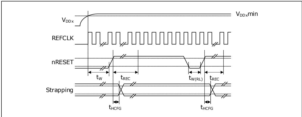
FIGURE 5-2: NRESET TIMING DIAGRAM
