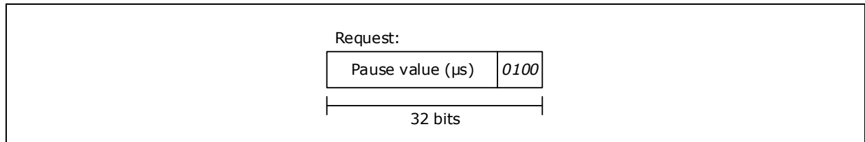
FIGURE 4-36: PAUSE COMMAND
