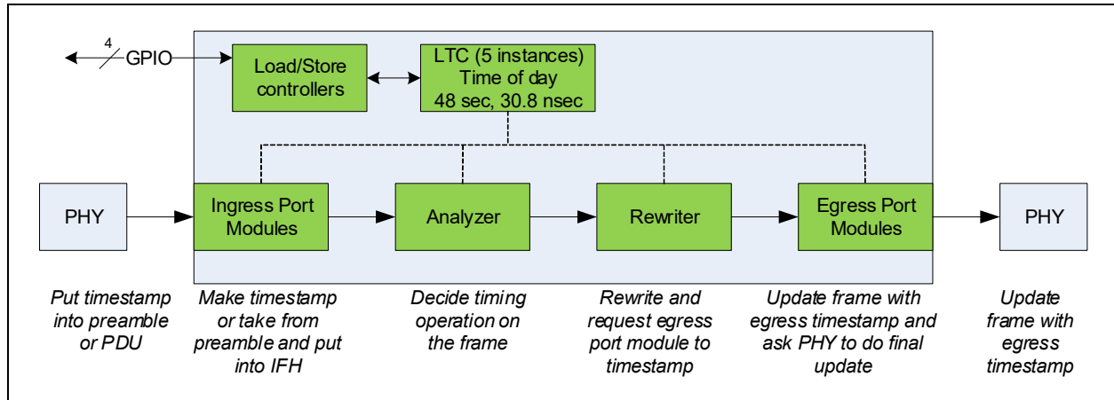
FIGURE 4-37: PTP FRAME PASSAGE
