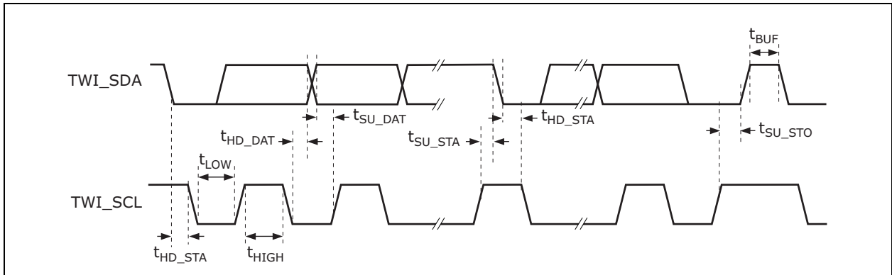
FIGURE 5-12: TWO-WIRE SERIAL WRITE TIMING DIAGRAM
