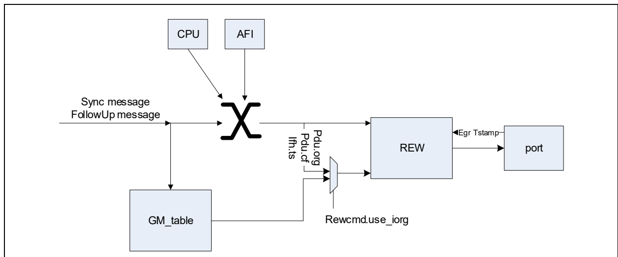
FIGURE 4-43: GPTP OPERATION
