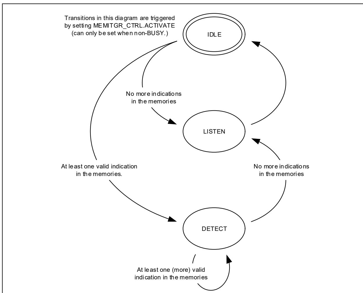
FIGURE 4-56: MONITOR STATE DIAGRAM
