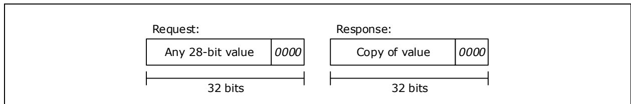
FIGURE 4-35: IDLE COMMAND
