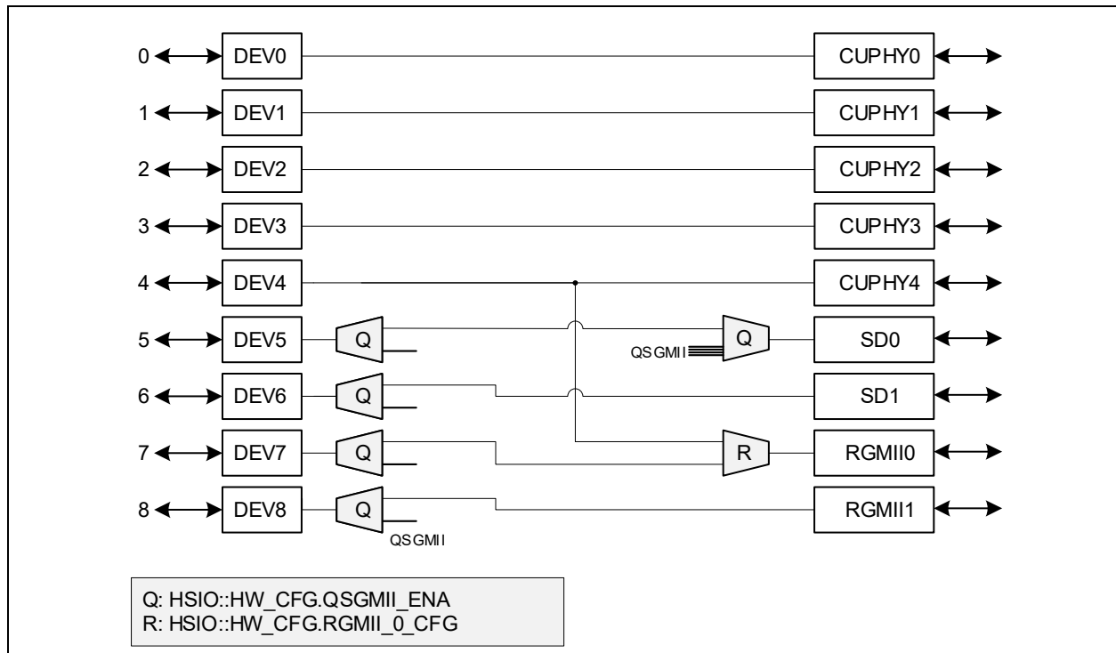
FIGURE 4-1: PORT MULTIPLEXING
