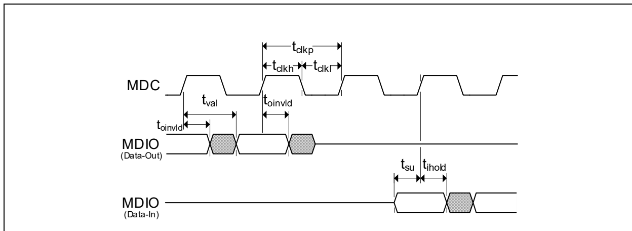
FIGURE 5-4: MIIM CLIENT TIMING DIAGRAM
