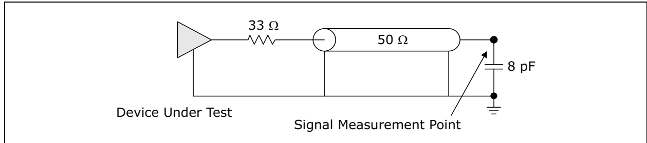
FIGURE 5-10: TEST CIRCUIT FOR RECOVERED CLOCK OUTPUT SIGNALS
