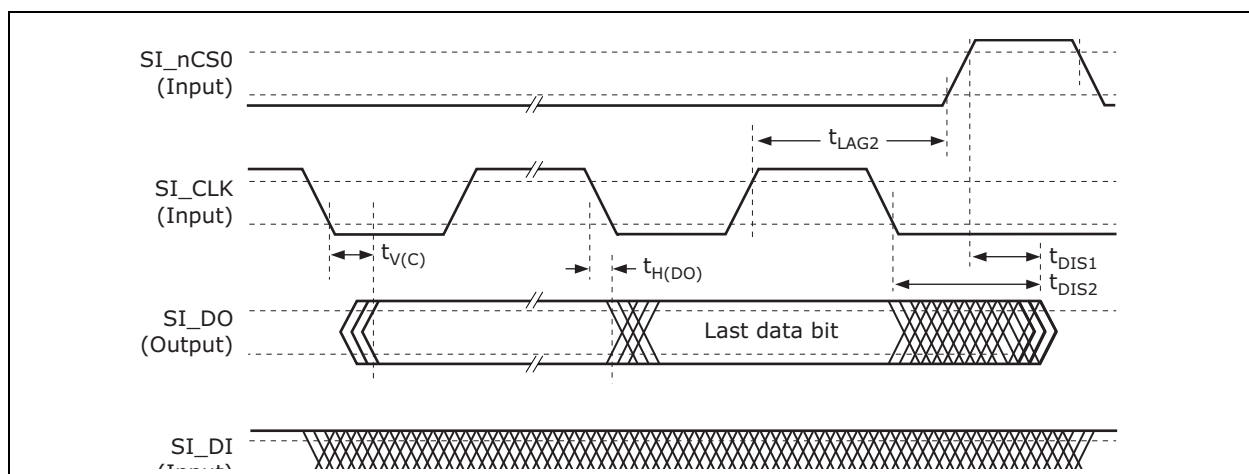
FIGURE 5-7: SI OUTPUT DATA TIMING DIAGRAM FOR CLIENT MODE
