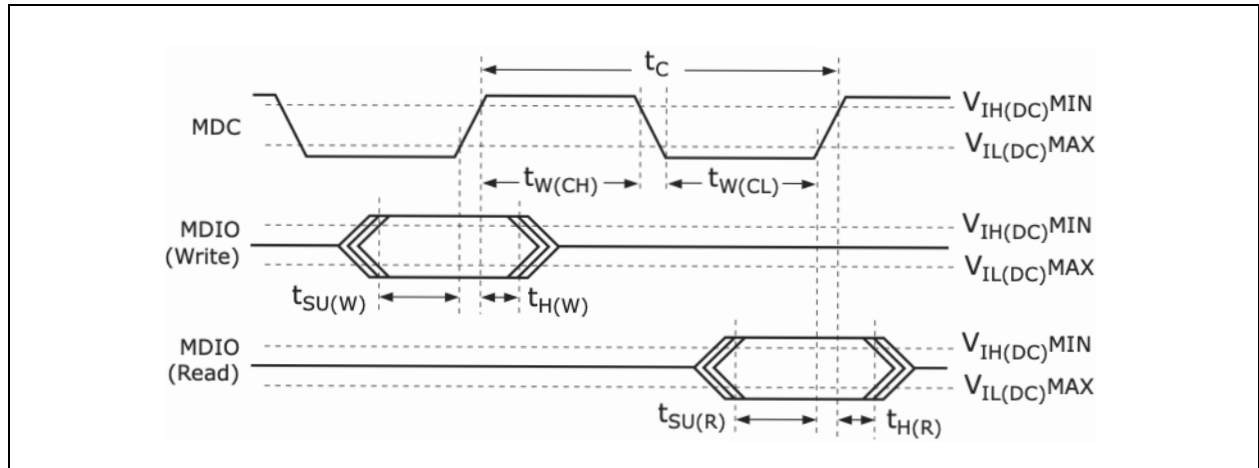
FIGURE 5-3: MIIM TIMING DIAGRAM
