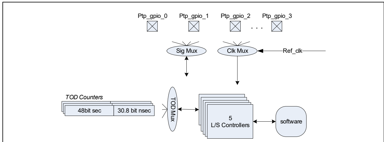
FIGURE 4-39: TIME-OF-DAY LOAD/STORE
