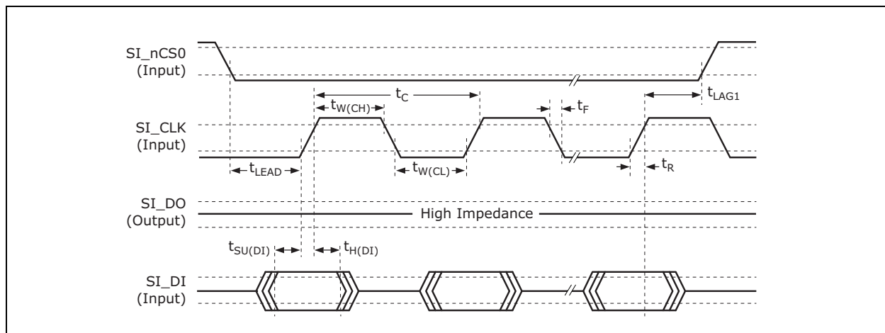
FIGURE 5-6: SI INPUT DATA TIMING DIAGRAM FOR CLIENT MODE
