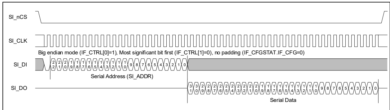
FIGURE 4-45: READ SEQUENCE FOR SI_CLK SLOW
