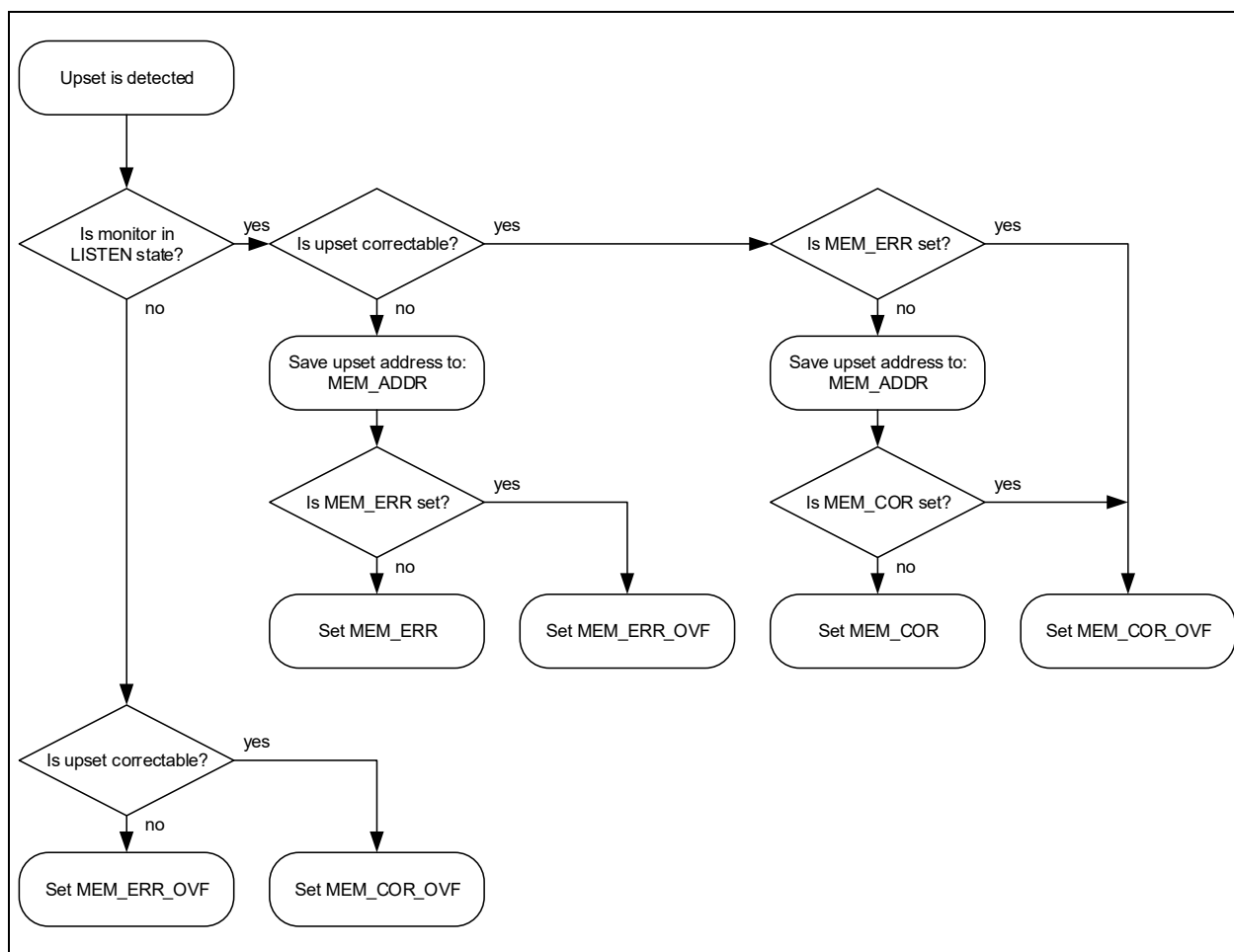
FIGURE 4-57: MEMORY DETECTION LOGIC
