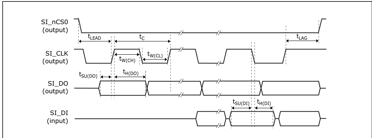
FIGURE 5-5: SI TIMING DIAGRAM
