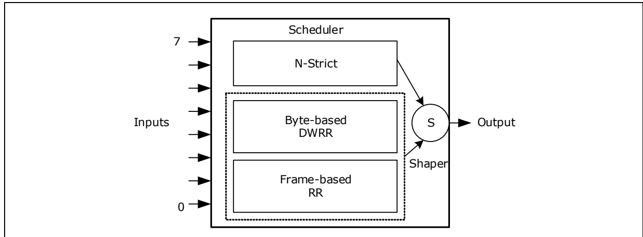
FIGURE 4-17: SCHEDULER ELEMENT
