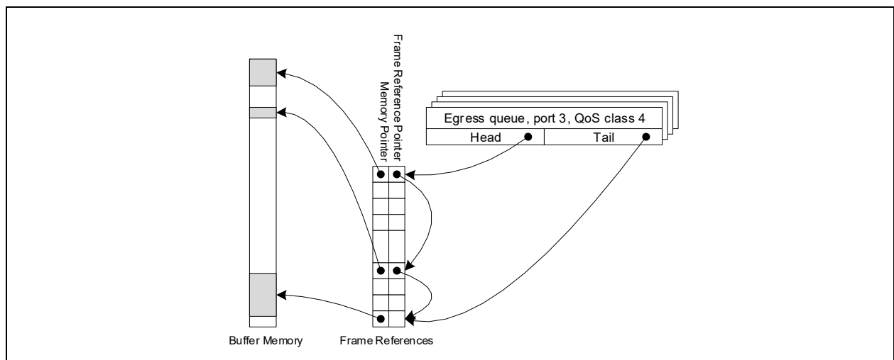
FIGURE 4-13: FRAME REFERENCE
