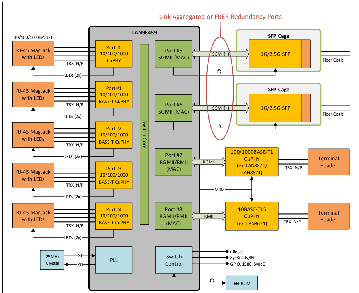
FIGURE 2-3: LAN96459S (WITH LAN8870/LAN8872 & LAN8671) - UNMANAGED 9-PORT 10/100/1000BASE-T + T1 + T1S + DUAL SFP SWITCH SYSTEM
