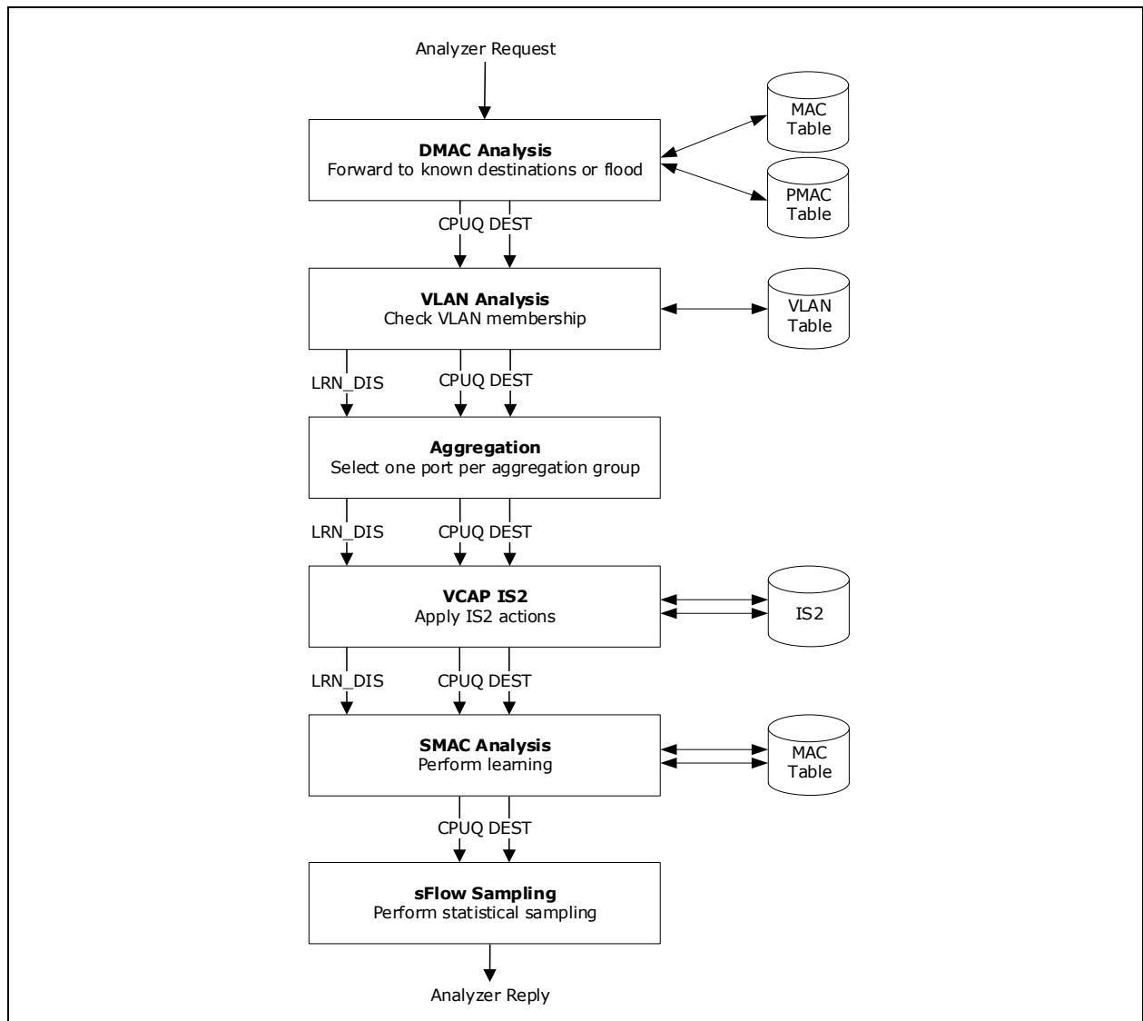
FIGURE 4-11: ANALYSIS STEPS
