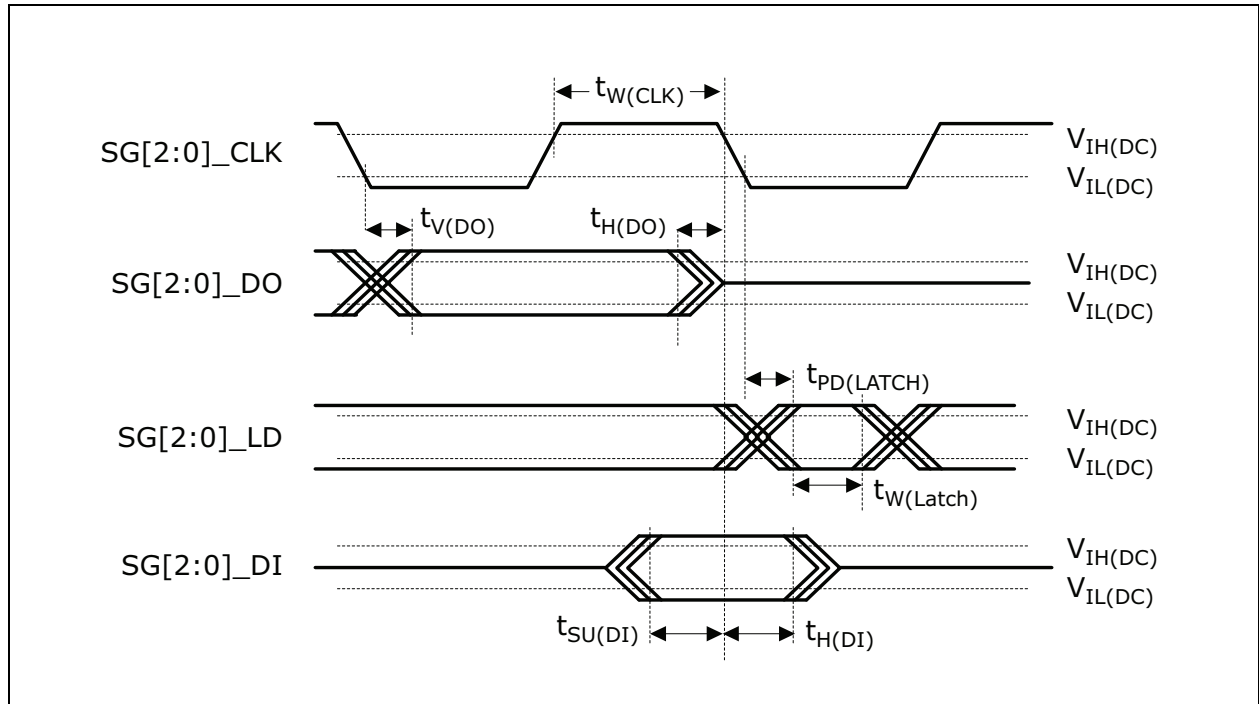
FIGURE 5-9: SERIAL I/O TIMING
