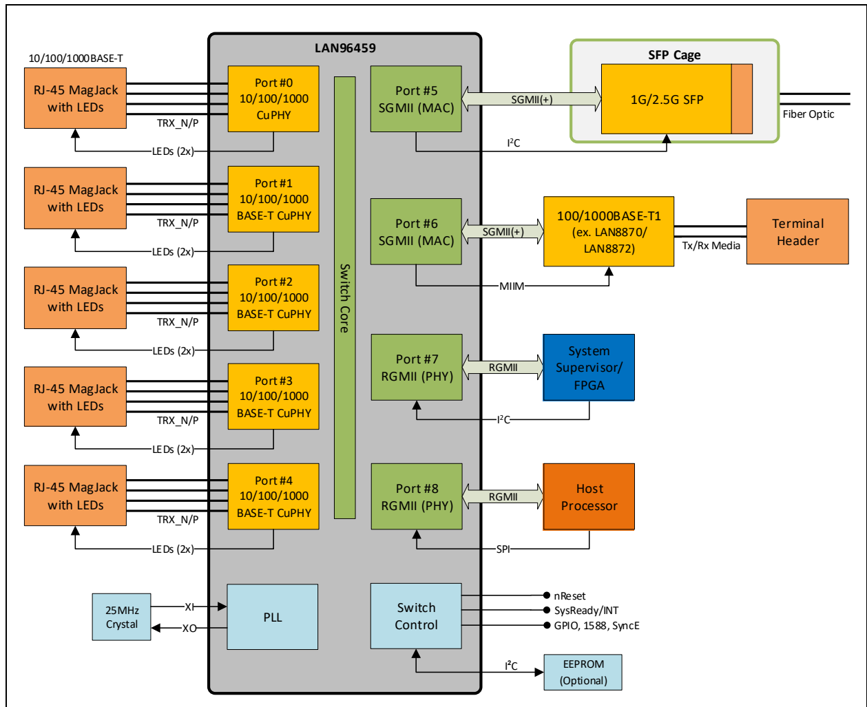
FIGURE 2-5: LAN96459F (WITH LAN8870/LAN8872 & LAN8671) - TSN MANAGED 9-PORT 10/100/1000BASE-T + T1 + DUAL NODE WITH SFP UPLINK SWITCH SYSTEM
