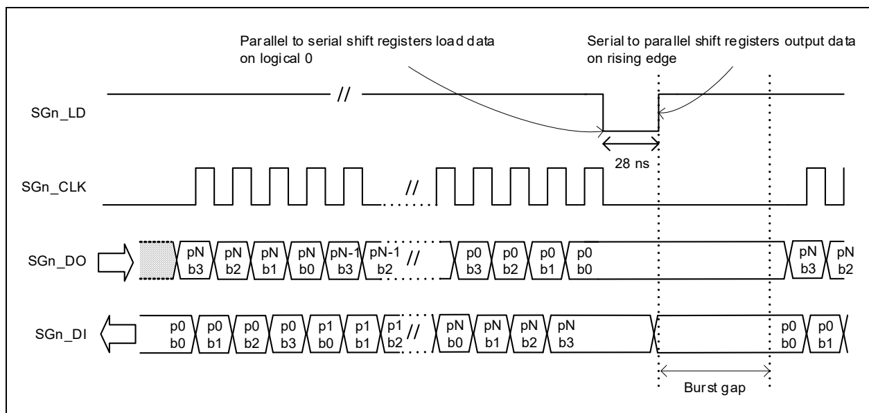
FIGURE 4-55: SIO TIMING
