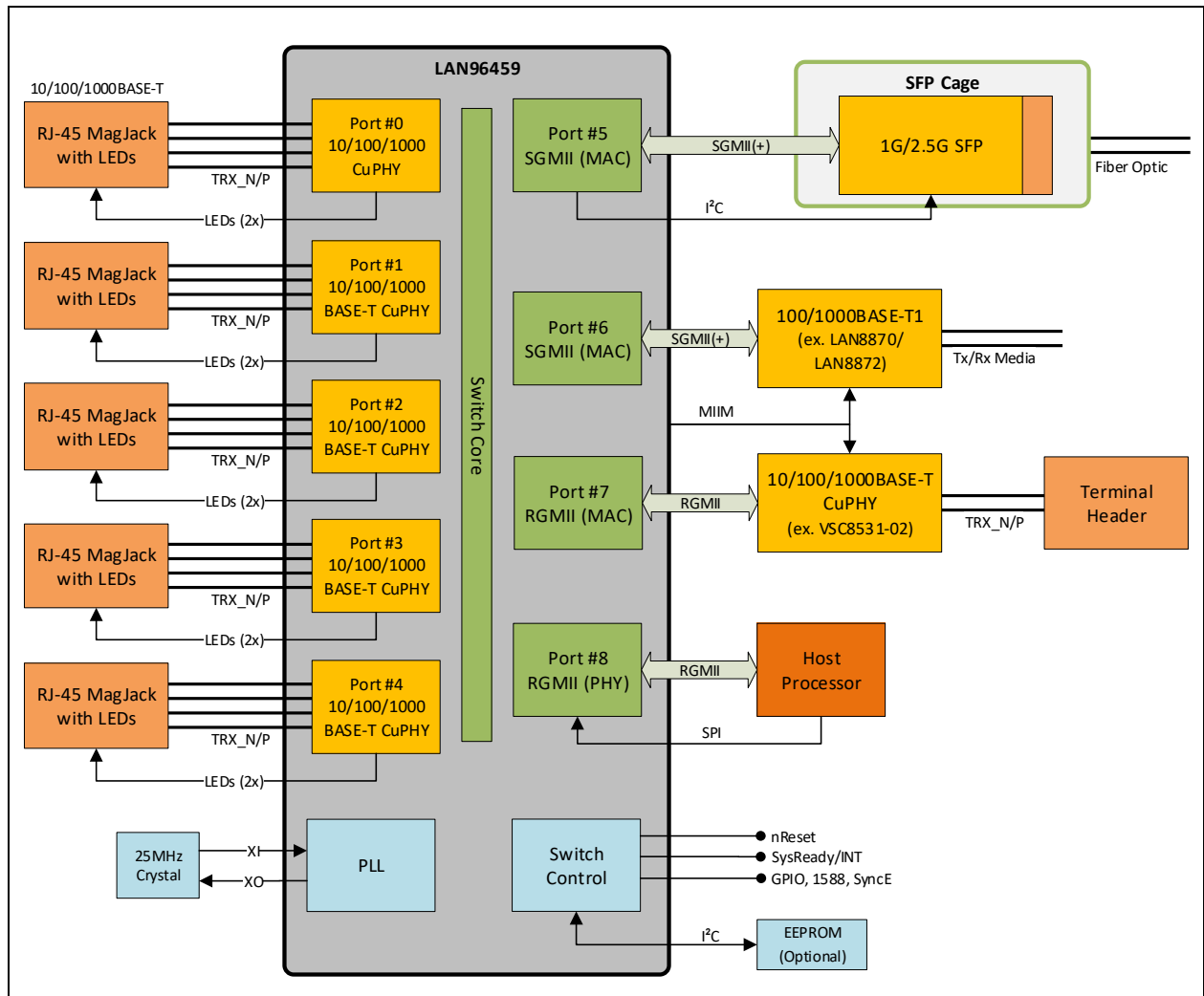
FIGURE 2-3: LAN96459F (WITH LAN8870/LAN8872 & VSC8531-02) MANAGED 9-PORT TSN 10/100/1000BASE-T + T1 SWITCH SYSTEM
