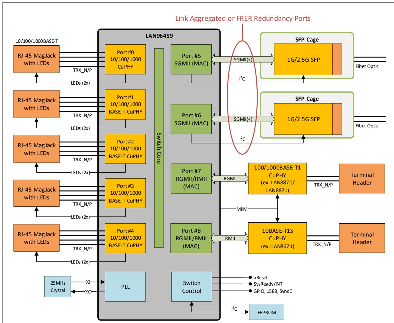
FIGURE 2-4: LAN96459F (WITH LAN8870/LAN8872 & LAN8671) - UNMANAGED 9-PORT 10/100/1000BASE-T + T1 + T1S + DUAL SFP SWITCH SYSTEM
