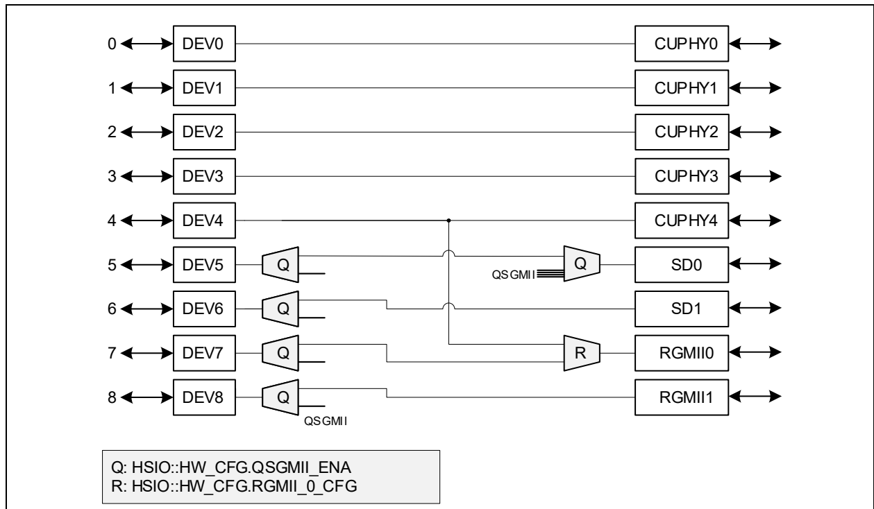
FIGURE 4-1: PORT MULTIPLEXING
