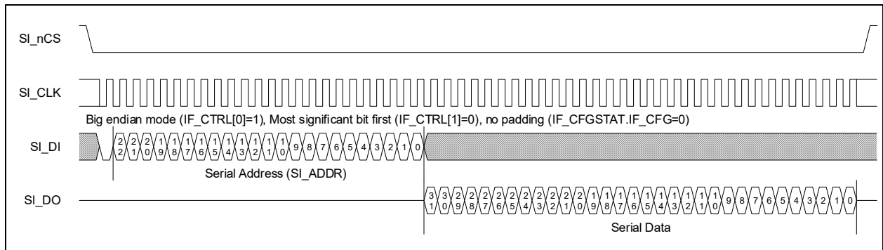
FIGURE 4-48: READ SEQUENCE FOR SI_CLK SLOW
