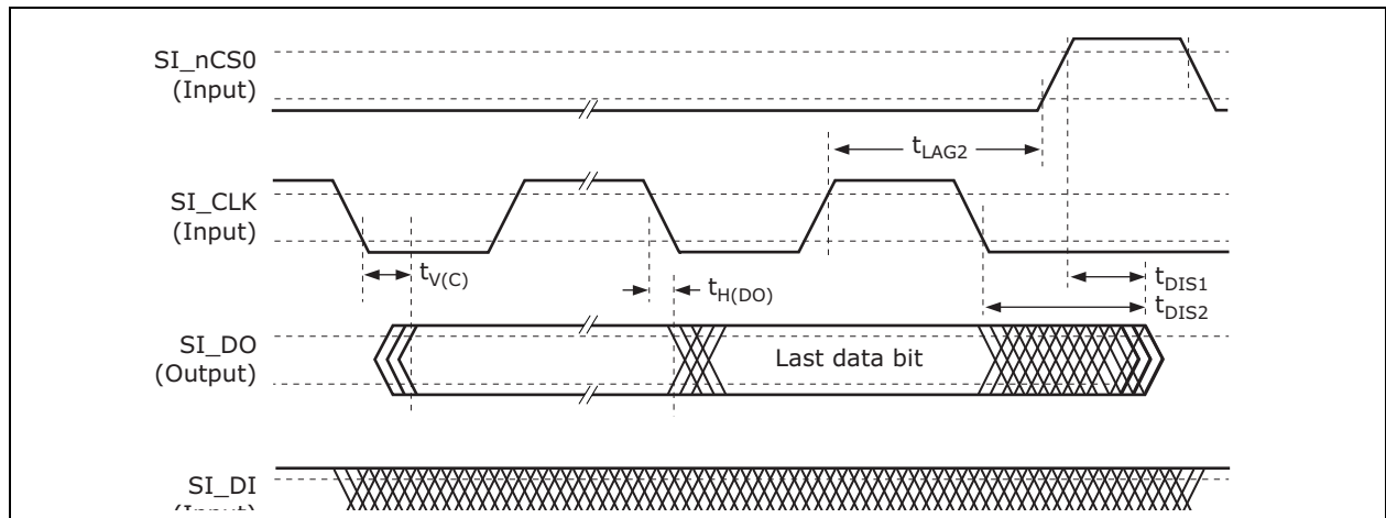
FIGURE 5-7: SI OUTPUT DATA TIMING DIAGRAM FOR CLIENT MODE
