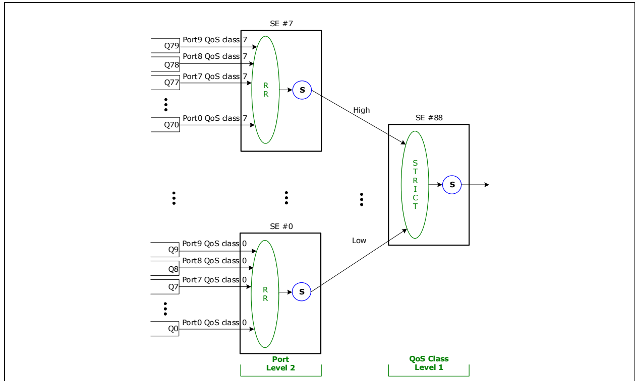
FIGURE 4-18: EGRESS SCHEDULER PORT 0
