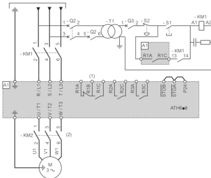
Three-phase Power Supply - Diagram With Downstream Contactor
