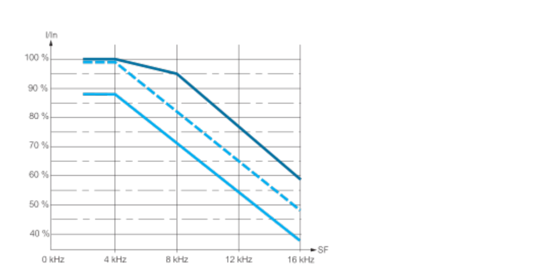
— 40 °C (104 °F) - Mounting type A, B and C - - - 50 °C (122 °F) - Mounting type A, B and C — 60 °C (140 °F) - Mounting type B and C I n : Nominal Drive Current SF : Switching Frequency
