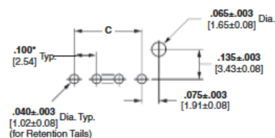
Section X-X
