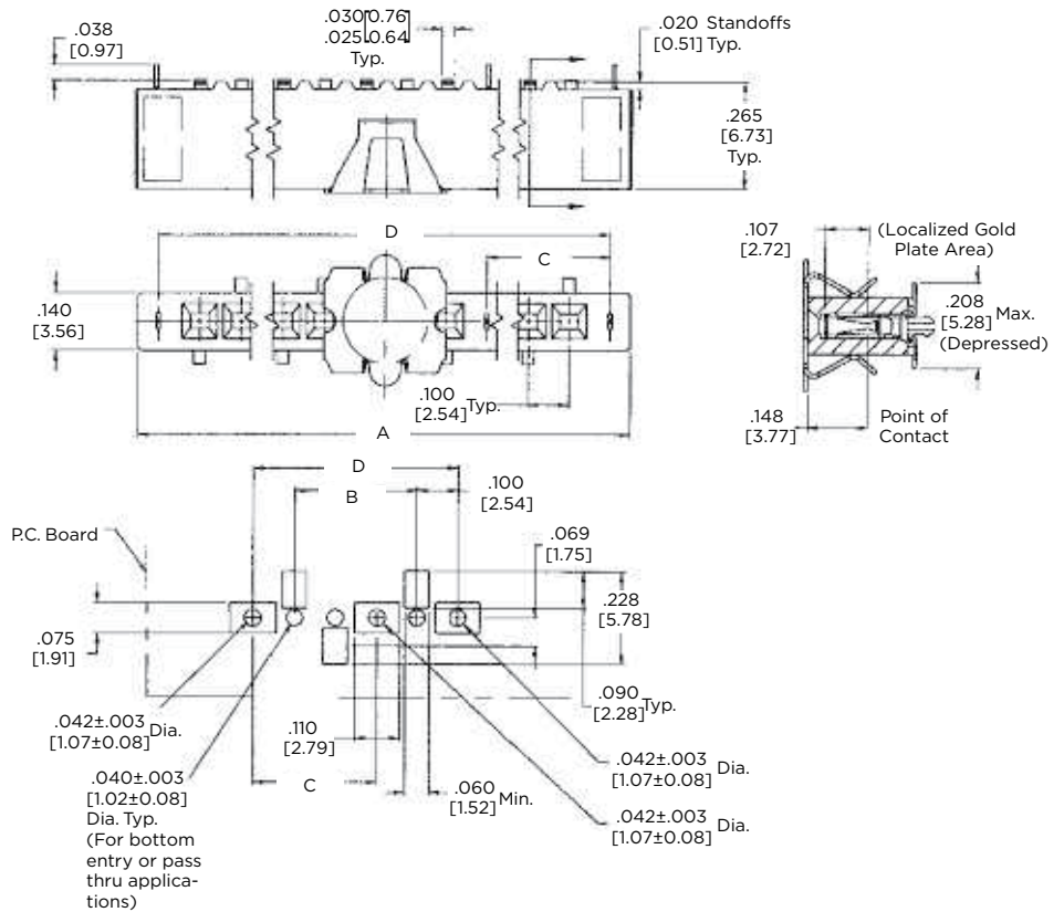
Recommended PC Board Pad Pattern (.008 [0.20] thick stencil)
