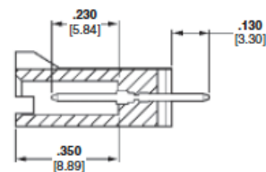
Section X-X
