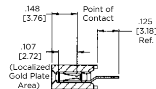
Section XX
