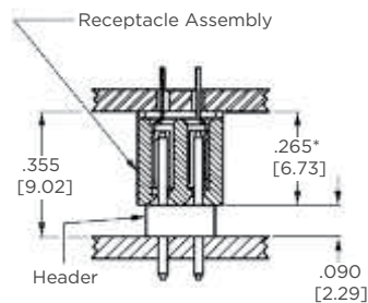
Figure 2 Double-Row, Mod IV, Top Entry, Breakaway Header
