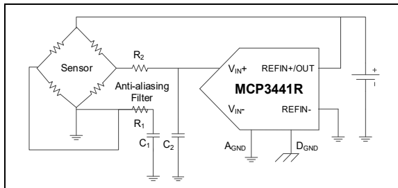
FIGURE 7-3: Wheatstone Bridge Ratiometric Connection.
