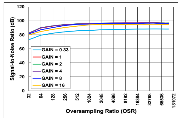
FIGURE 2-12: SNR vs. OSR (Internal V_{REF} ).
