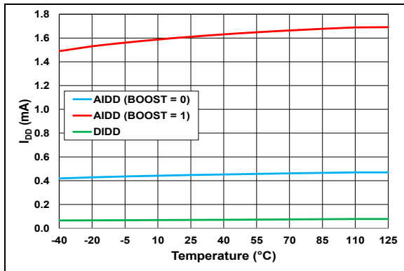
FIGURE 2-50: D I_{DD} and A I_{DD} vs. Temperature (External V_{REF} ).
