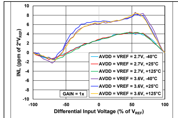
FIGURE 2-4: INL vs. Differential Input Voltage.
