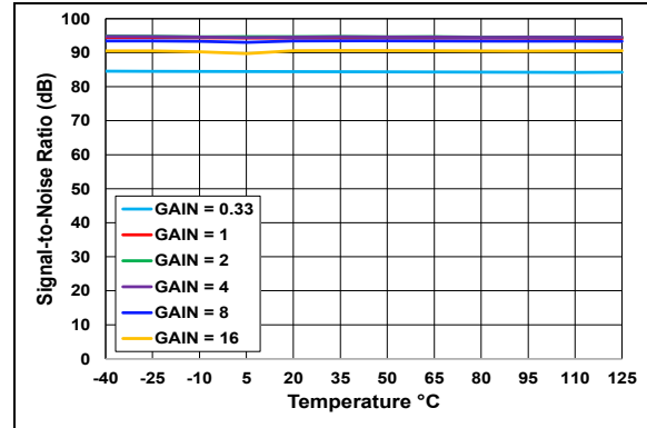
FIGURE 2-28: SNR vs. Temperature (Internal V_{REF} ).
