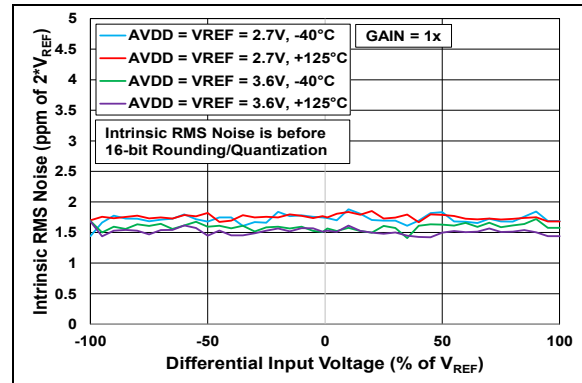
FIGURE 2-5: Output Noise vs. Differential Input Voltage.
