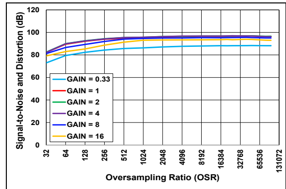
FIGURE 2-11: SINAD vs. OSR (Internal V_{REF} ).
