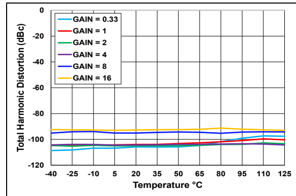
FIGURE 2-29: THD vs. Temperature (Internal V_{REF} ).
