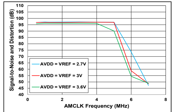
FIGURE 2-36: SINAD vs. AMCLK ( AV_{DD} = 2.7V, 3V, 3.6V ).
