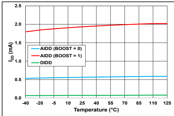
FIGURE 2-51: D I_{DD} and A I_{DD} vs. Temperature (Internal V_{REF} ).
