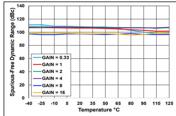
FIGURE 2-30: SFDR vs. Temperature (Internal V_{REF} ).
