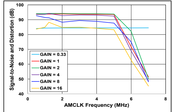
FIGURE 2-34: SINAD vs. AMCLK (BOOST = 0, Internal V_{REF} ).
