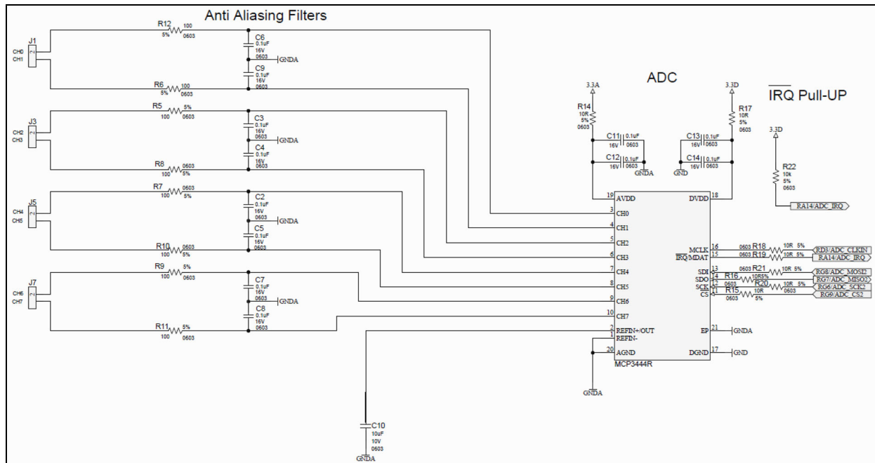
FIGURE 7-1: MCP3444R Application Example.
