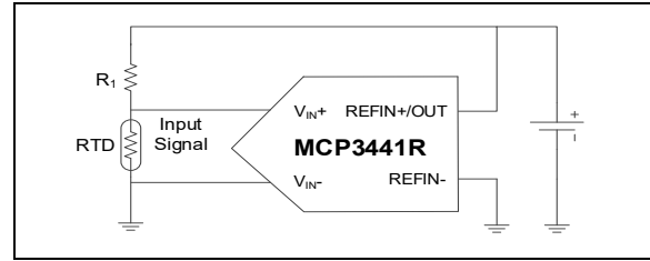
FIGURE 7-4: RTD Ratiometric Connection.
