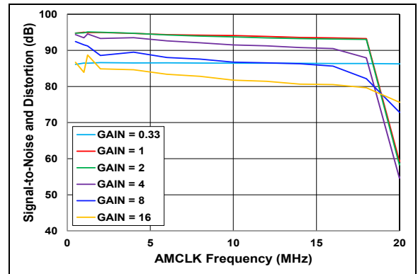
FIGURE 2-35: SINAD vs. AMCLK (BOOST = 1, Internal V_{REF} ).
