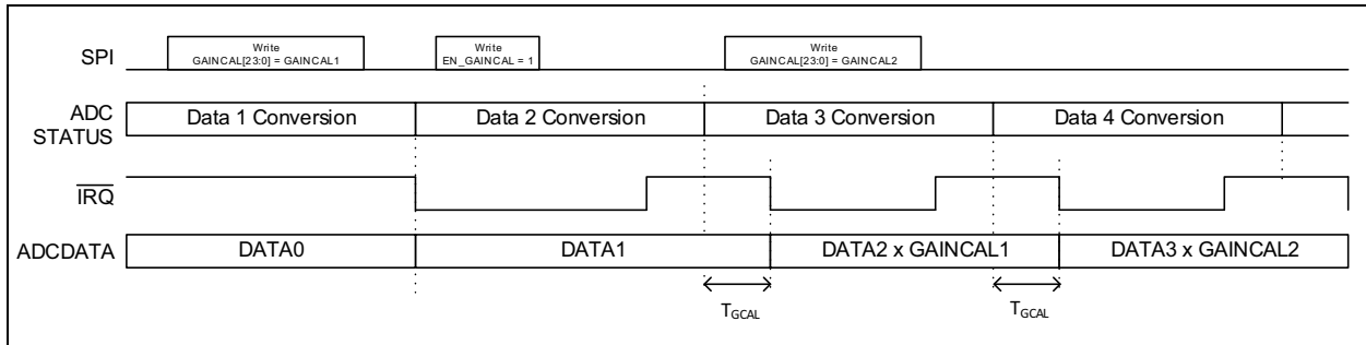
FIGURE 5-13: ADC Output and \overline{\text{IRQ}} Behavior with Digital Gain Error Calibration Enabled.
