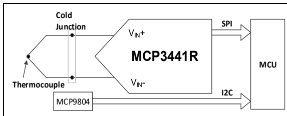
FIGURE 7-2: Thermocouple Connection.
