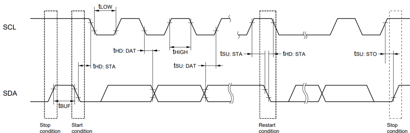
Figure 15. Bus Timing
