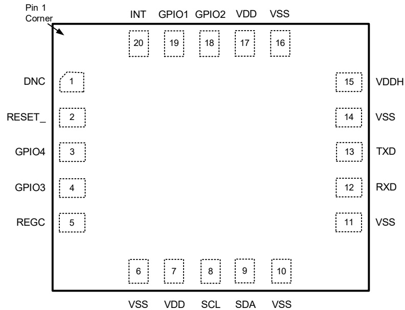
Figure 4. Pin Assignments (Top View)
