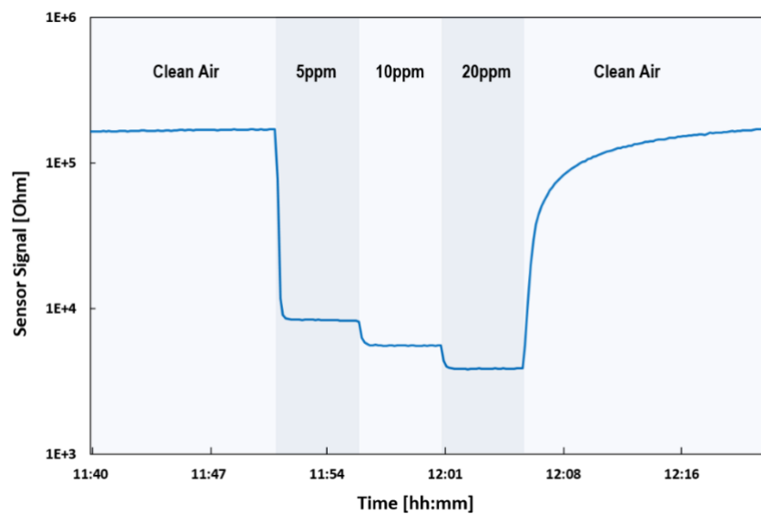
Figure 12. SGX6410 Typical Response Time and Signal Stability for TVOC Exposure
