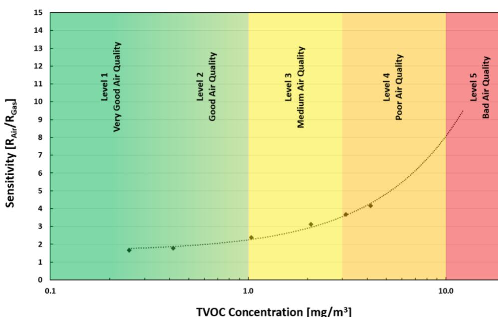
Figure 5. Typical SGX6410 Response to Levels of TVOC Described by UBA Using EPA Standard Mixture
