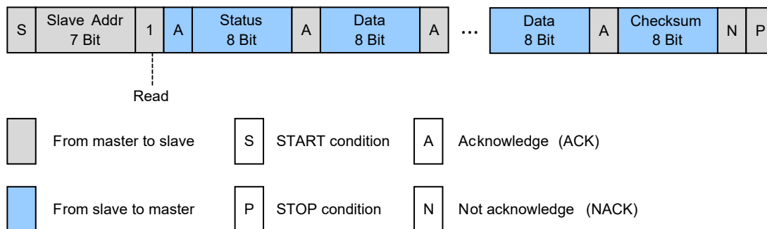
Figure 14. I 2 C Command Transmission Protocol
