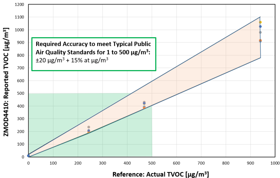
Figure 11. TVOC Measurement According to Typical PBAQ Standards using SGX6410
