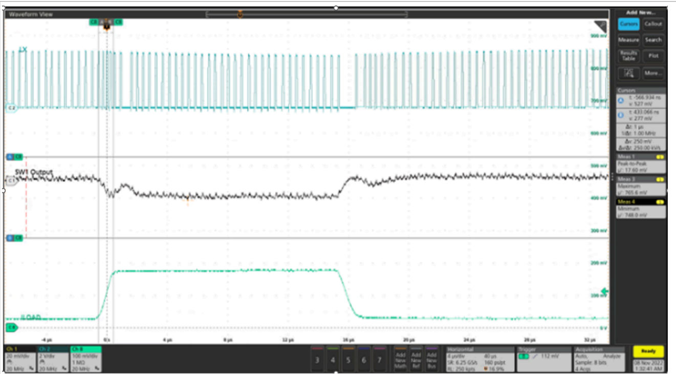
Figure 26. SW1 load transient response with AVP
