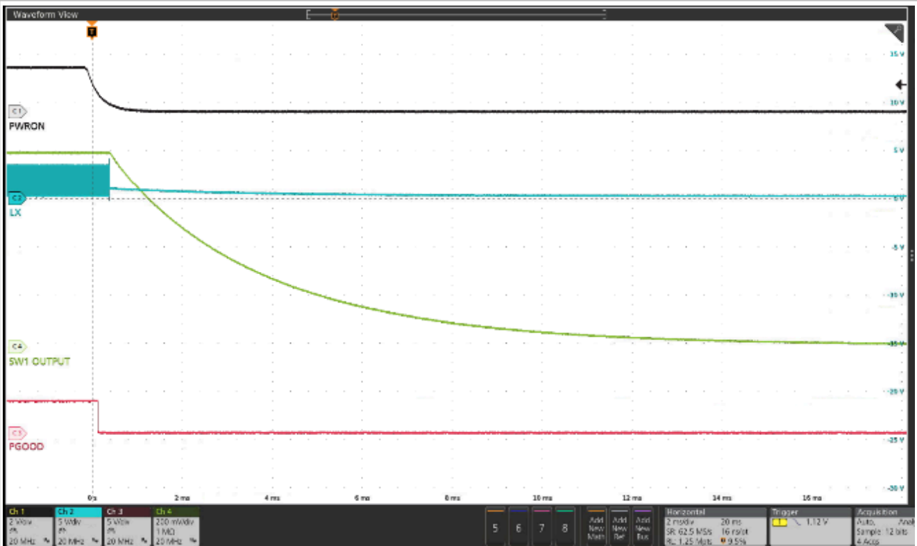
Figure 38. SW1 turn-off with OTP\_SW1\_RDIS = 1 and OTP\_SW1\_HIZOFF = 1
