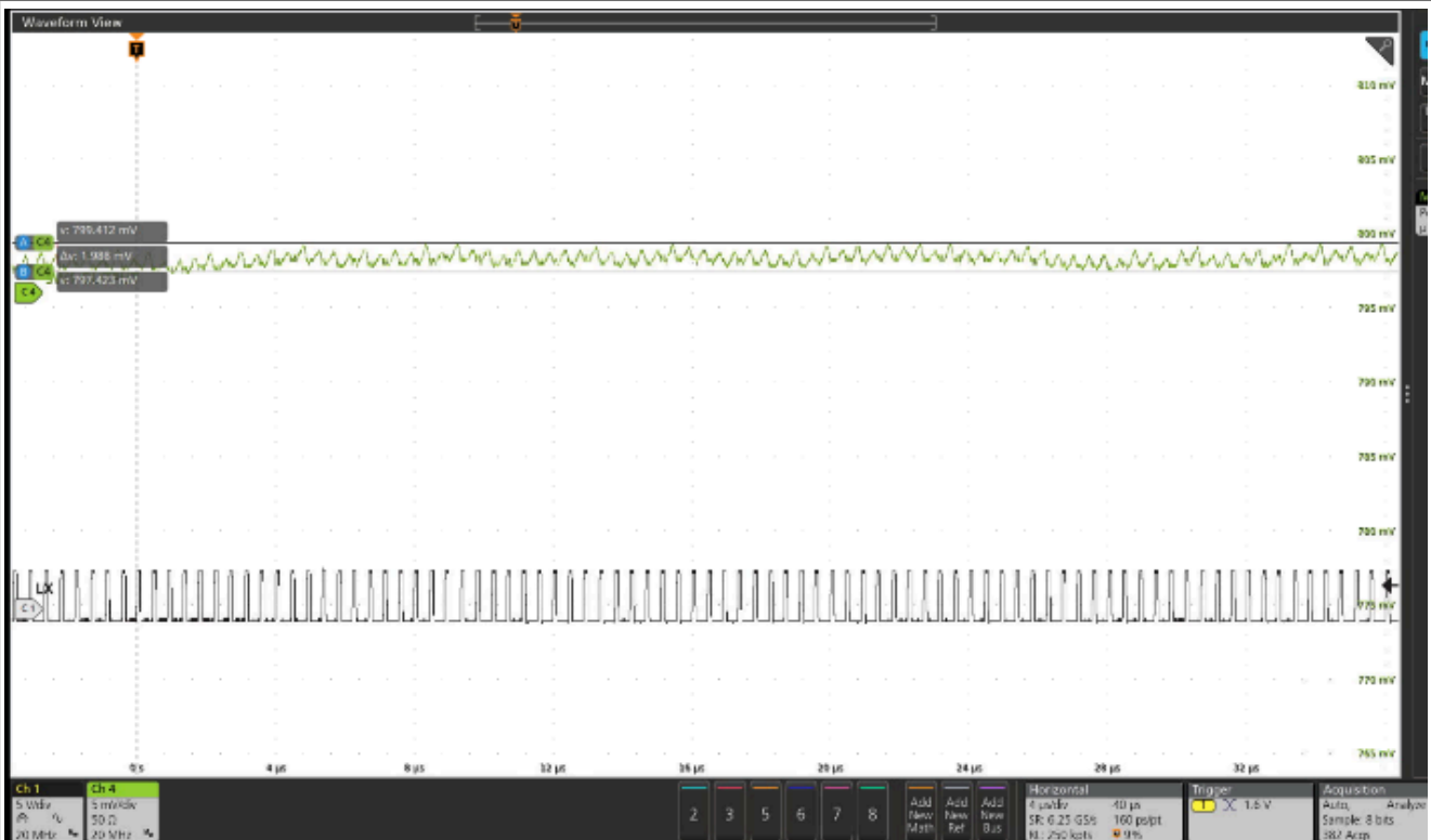
Figure 25. SW1 output ripple (MPF53BDAMMA1ES) ~ 3 mV
