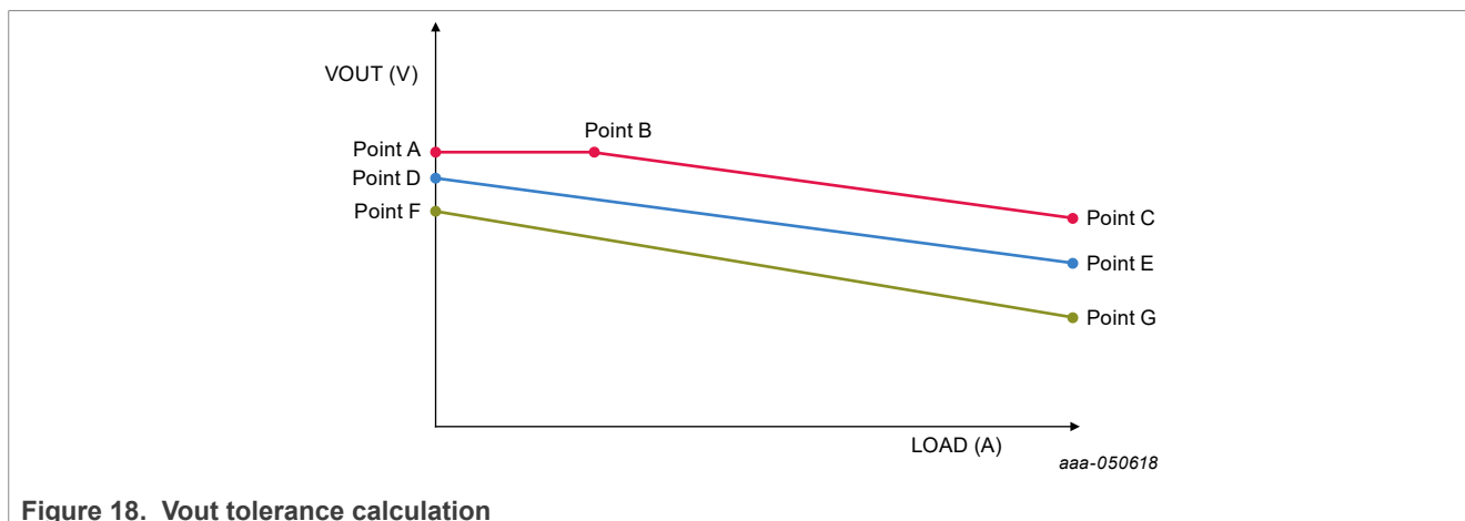
Figure 18. Vout tolerance calculation
