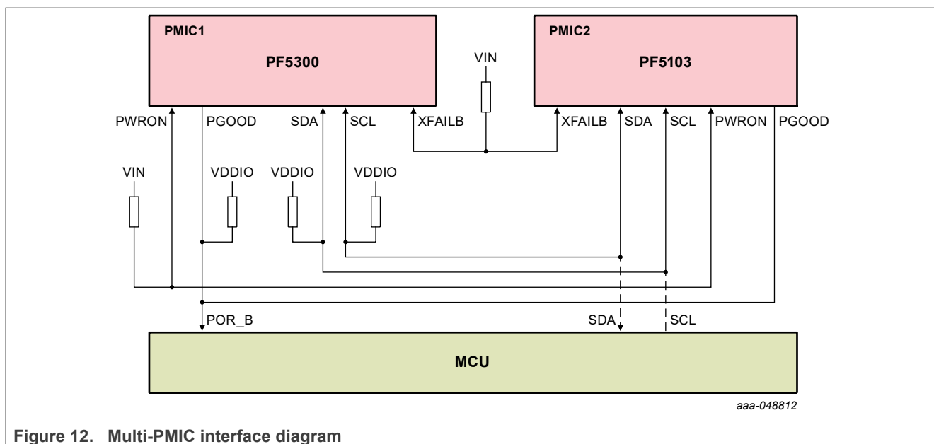
Figure 12. Multi-PMIC interface diagram
