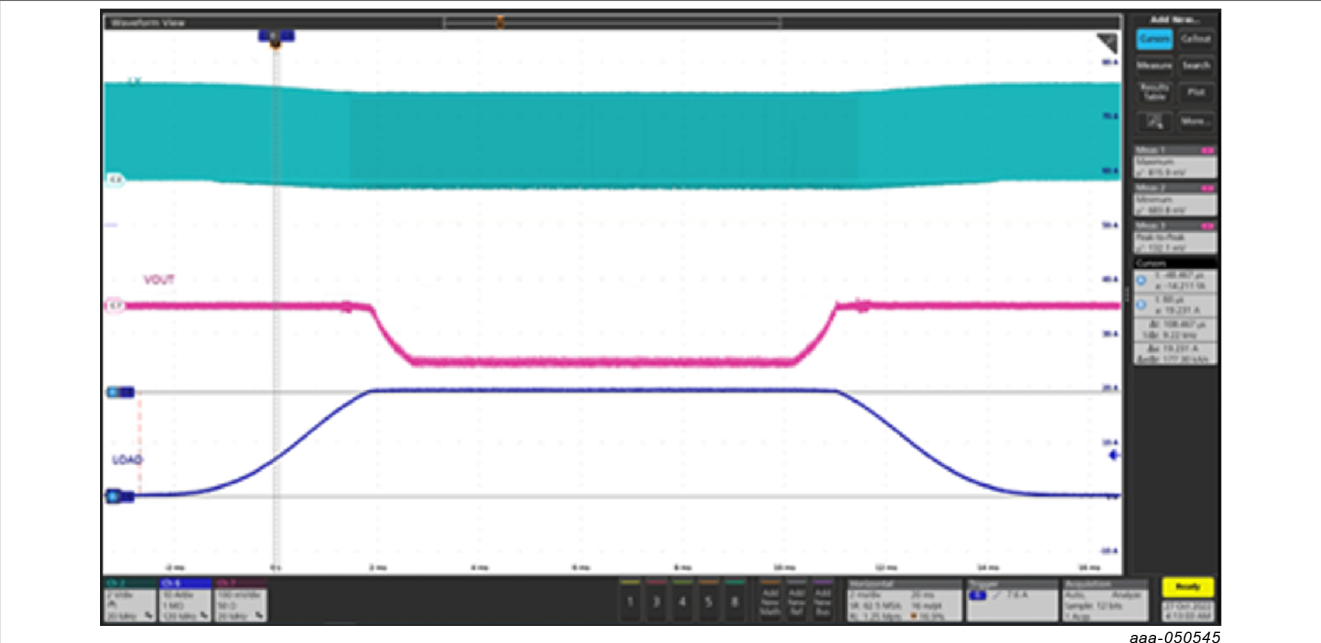
Figure 37. SW1 current limit entry and exit: V_{out} drops and recovers smoothly
