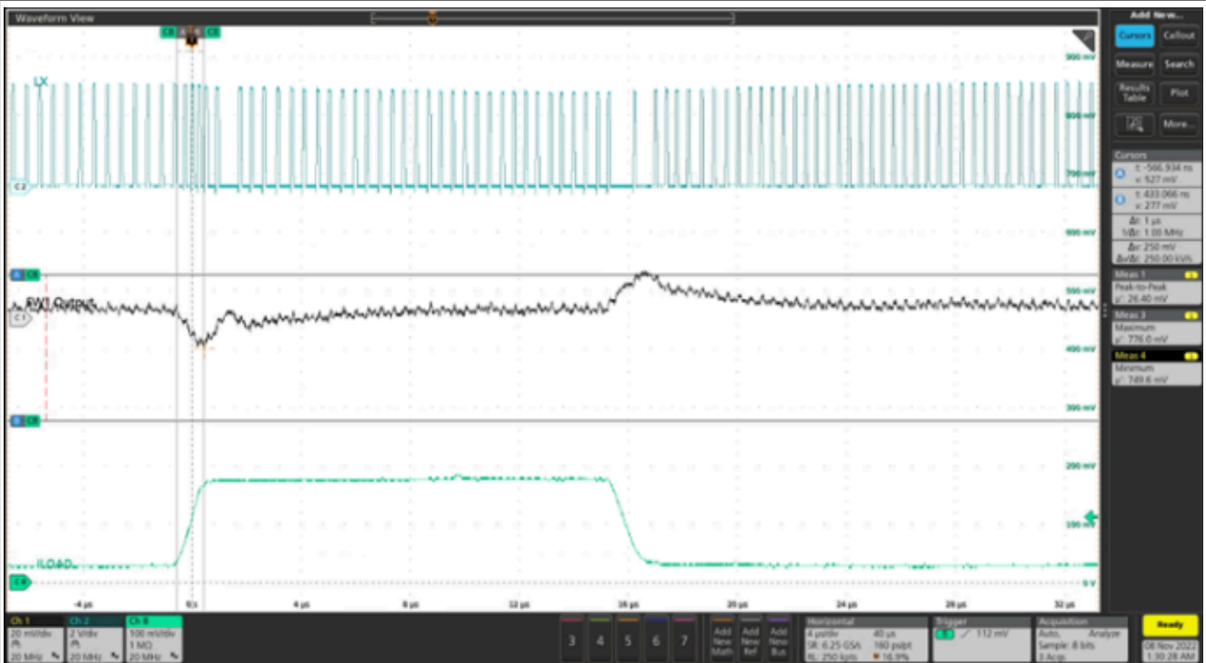
Figure 27. SW1 load transient response without AVP
