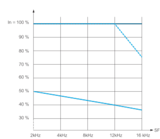
— 40 °C (104 °F) - Mounting type A - - - 50 °C (122 °F) - Mounting type A — 60 °C (140 °F) - Mounting type A In : Nominal Drive Current SF : Switching Frequency
