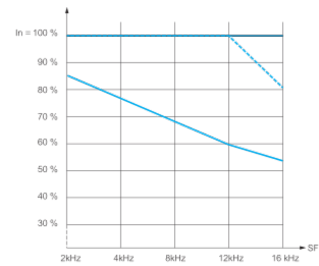
— 40 °C (104 °F) - Mounting type B - - - 50 °C (122 °F) - Mounting type B — 60 °C (140 °F) - Mounting type B In : Nominal Drive Current SF : Switching Frequency
