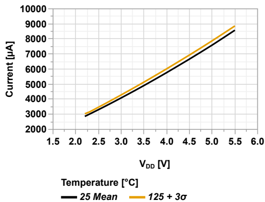
Figure 44-25. I_{DD} vs V_{DD} (ECH = 32 MHz, PMDx = 0x00)
