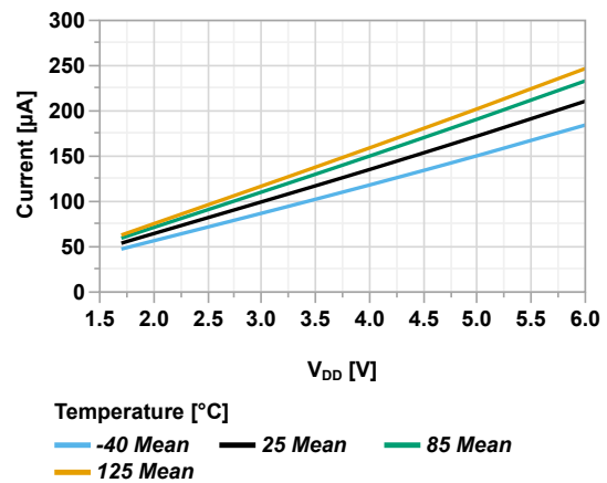
Figure 44-65. Weak Pull-Up Current vs V_{DD} (Mean Values)
