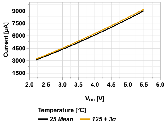
Figure 44-11. I_{DD} vs V_{DD} (HFINTOSC = 32 MHz, PMDx = 0x00)
