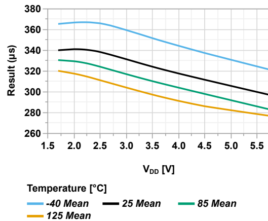
Figure 44-73. LFO Oscillator Start-Up Time vs V_{DD}
