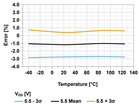
Figure 44-146. CDAFVR Voltage Error vs Temperature ( V_{DD} = 5.5V , V_{REF} = 2.048V )
