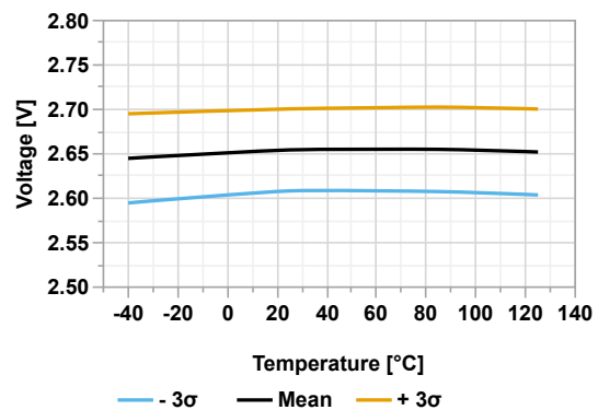
Figure 44-76. Brown-out Reset Voltage Threshold Level vs Temperature (BORV = '0')
