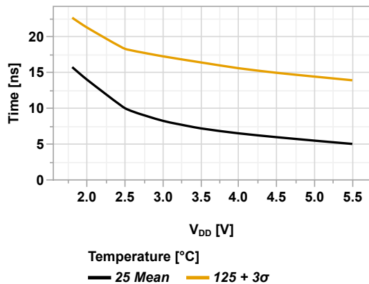
Figure 44-46. Fall Time vs V_{DD} (SLRxn = '1', T_A = 125^\circ\text{C} )
