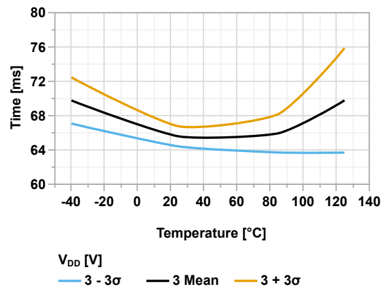
Figure 44-85. Start-Up Time vs Temperature (PWRTS = 'b10, V_{DD} = 3.0V )
