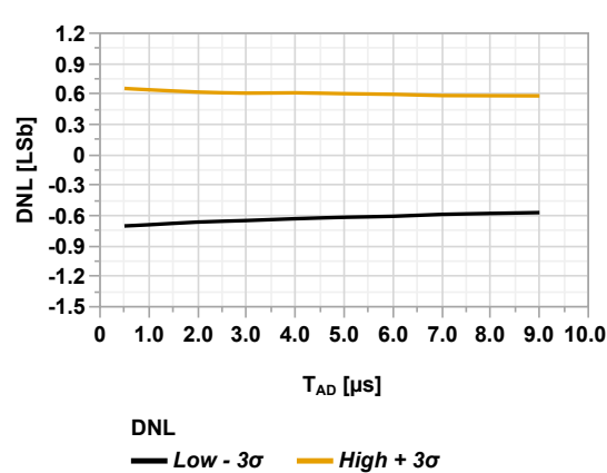
Figure 44-93. ADC DNL vs T_{AD} (Single-Ended Mode, V_{REF+} = V_{DD} = 3.0V , T_A = 125^\circ C , CPON = 'b11')
