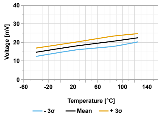
Figure 44-80. Low-Power Brown-out Reset Hysteresis vs Temperature
