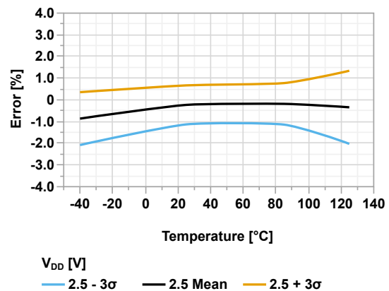
Figure 44-138. ADFVR Voltage Error vs Temperature ( V_{DD} = 2.5V , V_{REF} = 2.048V )
