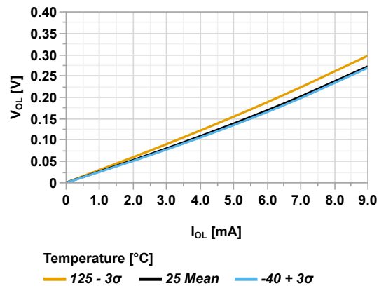
Figure 44-61. Output Pin Maximum V_{OL} vs Current ( V_{DD} = 1.8V )
