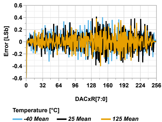
Figure 44-106. DAC DNL vs. DAC Code ( V_{REF} = V_{DD} = 5.5V )
