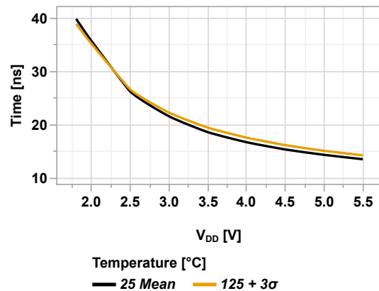
Figure 44-47. Fall Time vs V_{DD} (SLRxn = '0', T_A = 125^\circ\text{C} )
