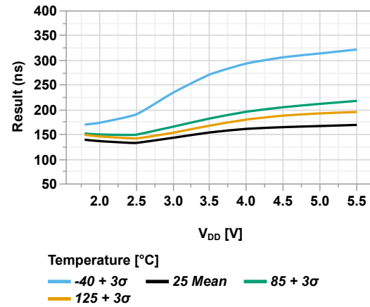
Figure 44-131. Falling Edge Response Time vs V_{DD} (CxSP = '0', CPON = 'b01')
