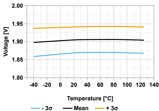
Figure 44-75. Brown-out Reset Voltage Threshold Level vs Temperature (BORV = '1')
