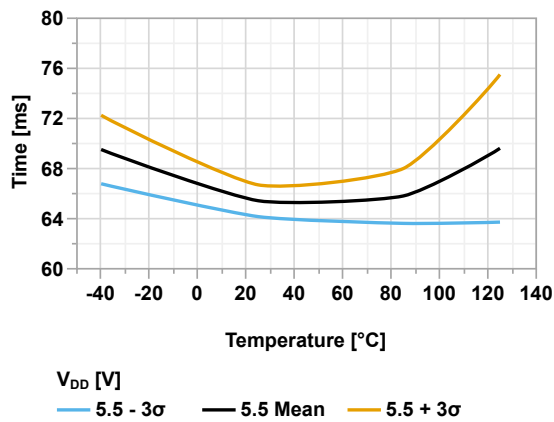
Figure 44-86. Start-Up Time vs Temperature (PWRTS = 'b10, V_{DD} = 5.5V )
