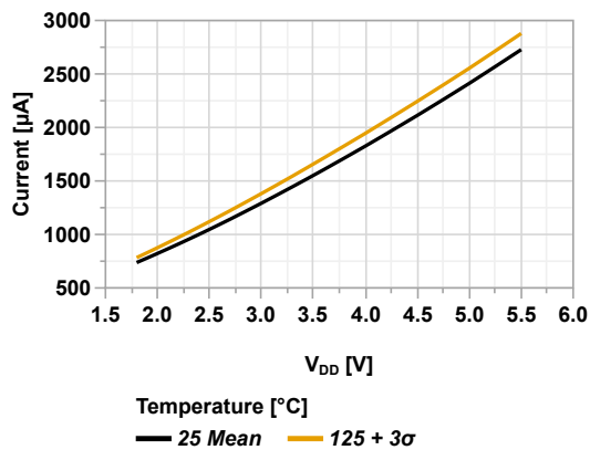
Figure 44-27. I_{DD} vs V_{DD} (Doze Mode, HFINTOSC = 16 MHz, PMDx = 0x00)
