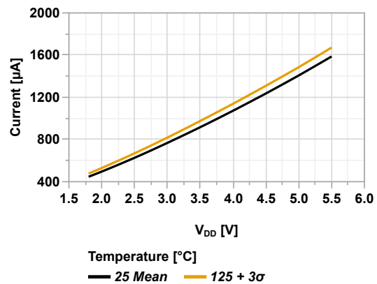
Figure 44-28. I_{DD} vs V_{DD} (Doze Mode, HFINTOSC = 16 MHz, PMDx = 0xFF)
