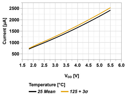
Figure 44-7. I_{DD} vs V_{DD} (HFINTOSC = 8 MHz, PMDx = 0x00)
