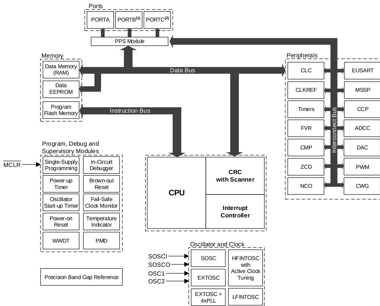
Figure 1. PIC16F18114/15/24/25/44/45 Block Diagram
