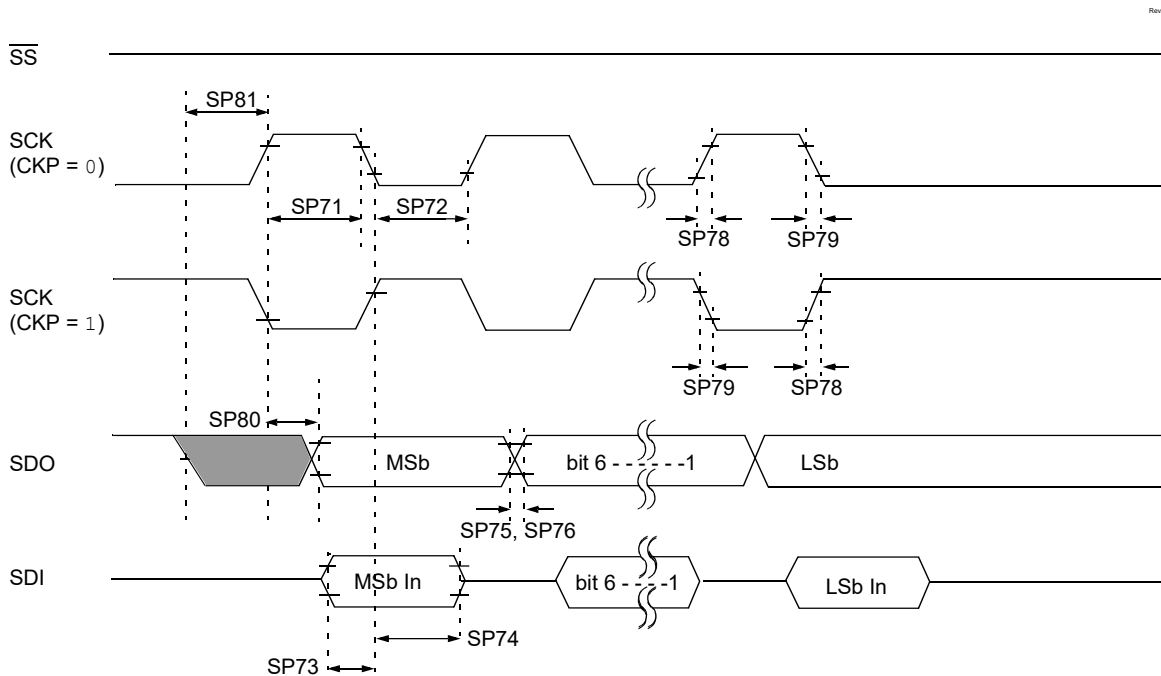
Figure 43-15. SPI Host Mode Timing (CKE = 0, SMP = 0)
