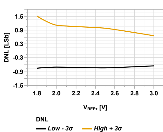
Figure 44-94. ADC DNL vs V_{REF+} (Single-Ended Mode, T_{AD} = 1 \mu s , V_{DD} = 3.0V , T_A = 125^\circ C , CPON = 'b11')
