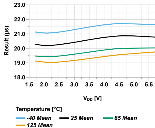
Figure 44-69. HFO Oscillator Start-Up Time vs V_{DD}
