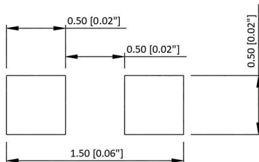
Recommend Pad Layout
