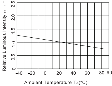
Ambient Temperature VS. Relative Intensity T a -I v
