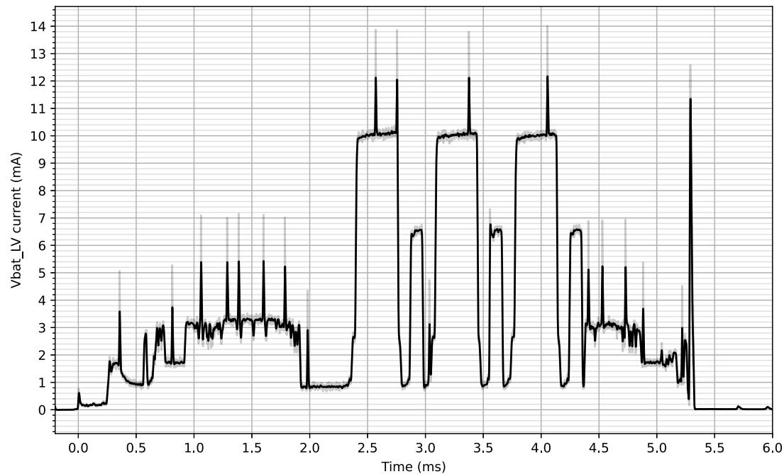
Figure 19. Power consumption during Bluetooth Low Energy advertising during LV_SM mode with VBAT_LV = 1.5 V, VBAT_HV = 1.8V and VDD_RF = VBAT_LV
