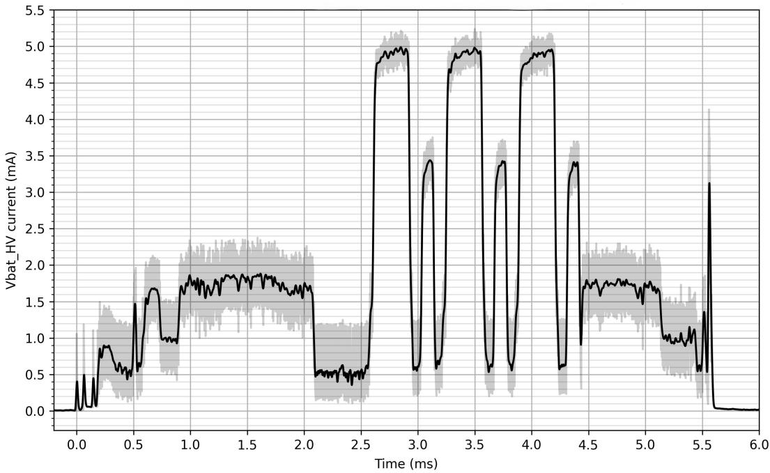
Figure 18. Power consumption during Bluetooth Low Energy advertising during HV_SM mode with VBAT_HV = 3 V, VBAT_LV = 1.2V and VDD_RF = VBAT_LV
