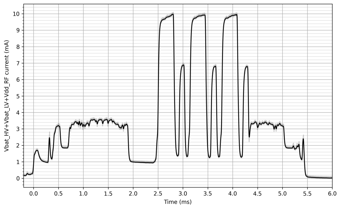
Figure 17. Power consumption during Bluetooth Low Energy advertising during XR_SM mode with VBAT_HV = VBAT_LV = VDD_RF = 1.8V
