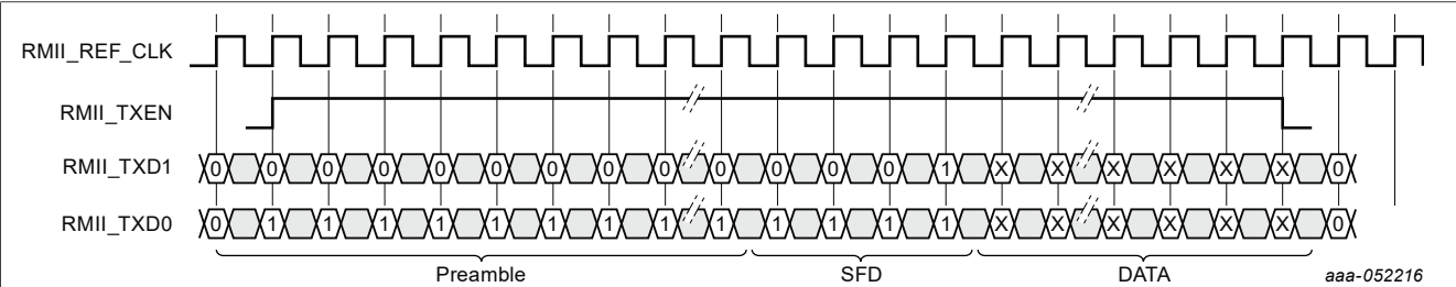
Figure 20. RMII transmit operation
