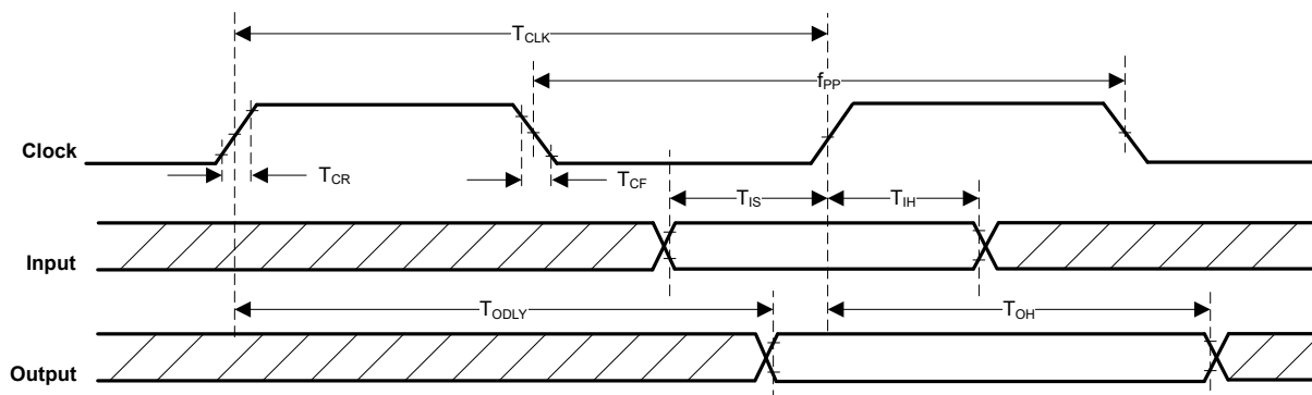
Figure 59. SDIO protocol timing diagram—SDR12, SDR25, SDR50 Modes (up to 100 MHz) (1.8V)
