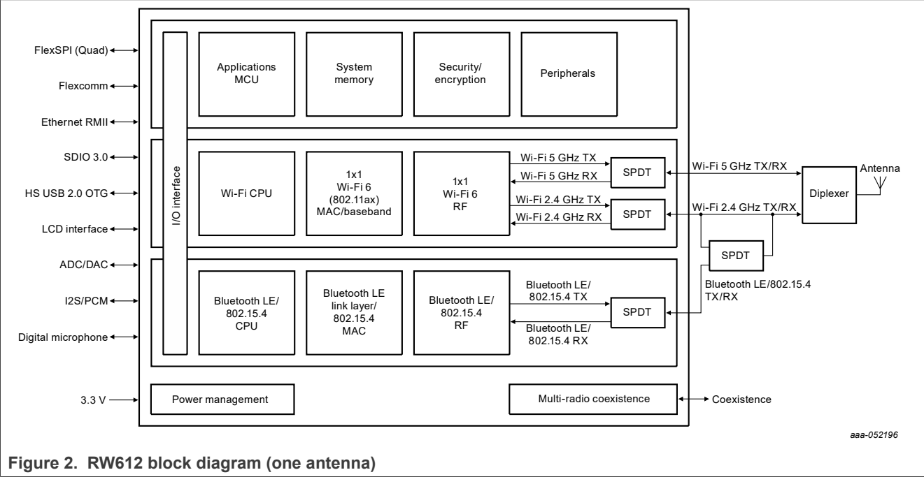
Figure 2 shows RW612 overall block diagram for the single-antenna configuration.
