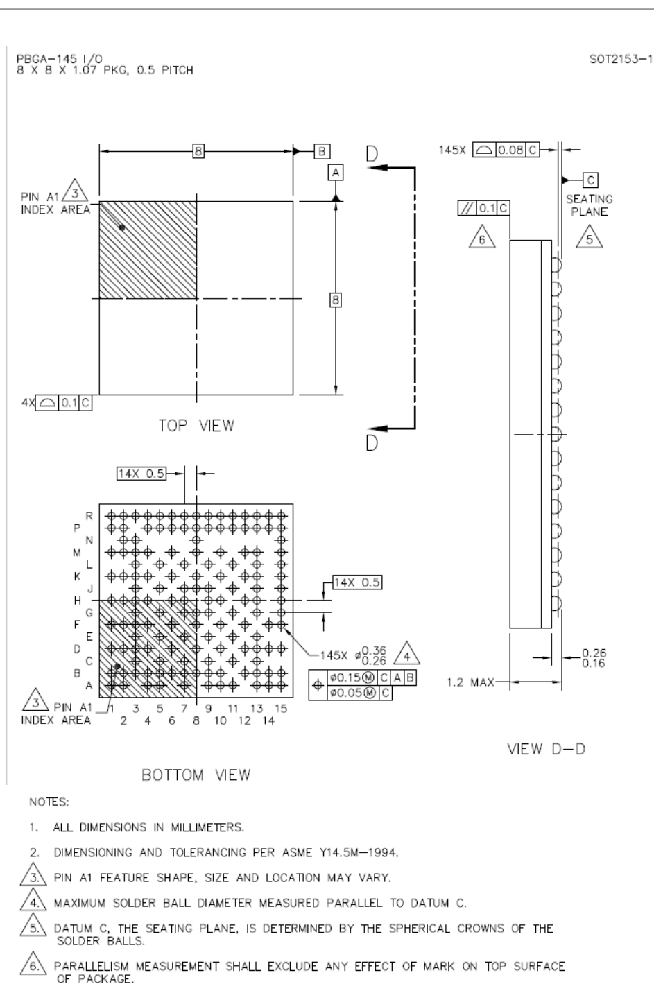
Figure 78. TFBGA145 package mechanical drawing
