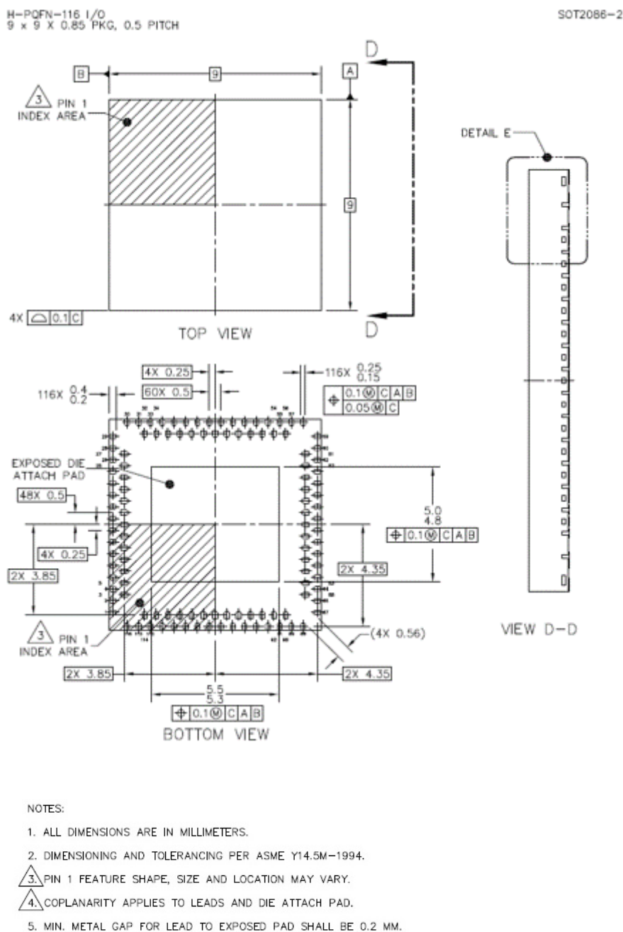
Figure 79. HVQFN116 package drawing
