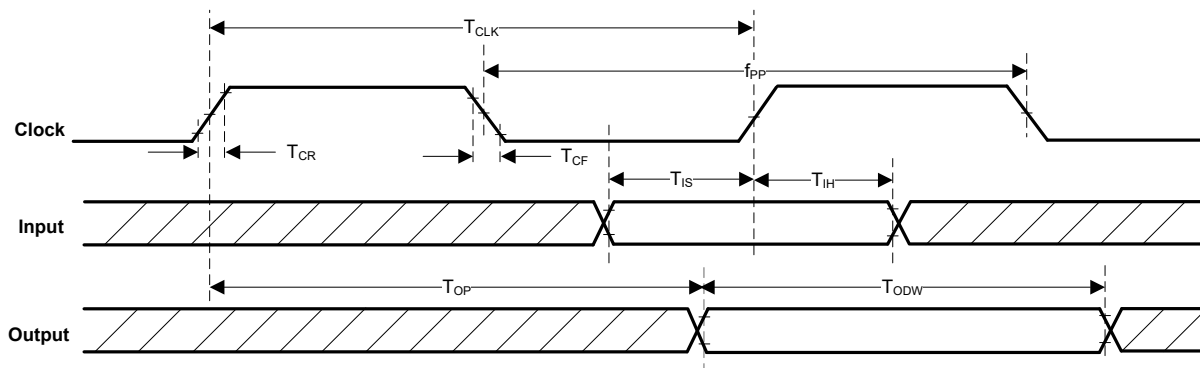
Figure 60. SDIO protocol timing diagram—SDR104 mode (208 MHz)
