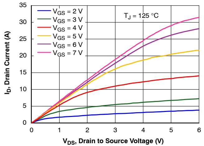
Figure 2. Output Characteristics at T_J = 125^\circ\text{C}
