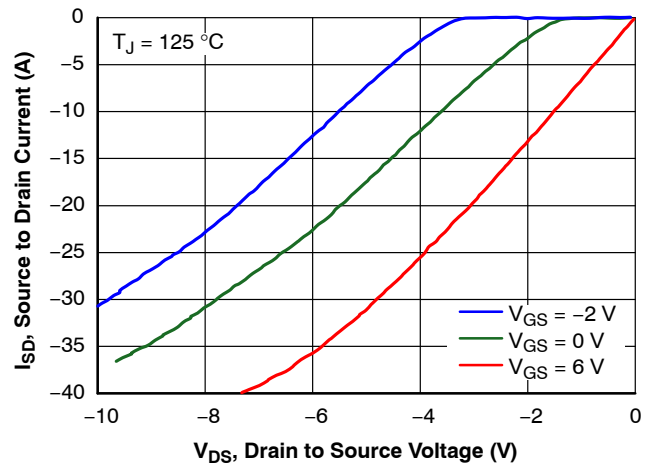
Figure 8. Reverse Conduction Characteristics at T_J = 125^\circ\text{C}
