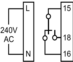
A) 1 Channel Device
