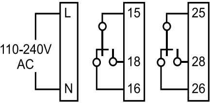
B) 2 Channel Device
