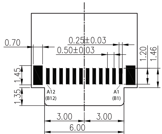
Recommended Stencil Top View (Bottom View)
