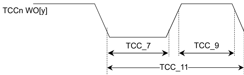
Figure 38-13. TCCn Timer Compare Output Module Timing Diagrams
