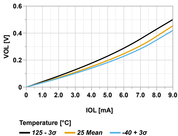
Figure 39-10. Output Pin - Maximum V_{OL} vs. Current, V_{DD} = 1.8V
