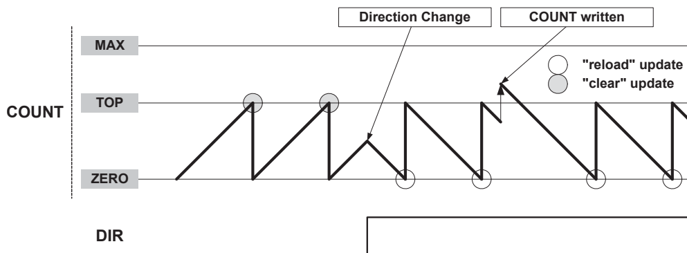
Figure 23-4. Counter Operation
