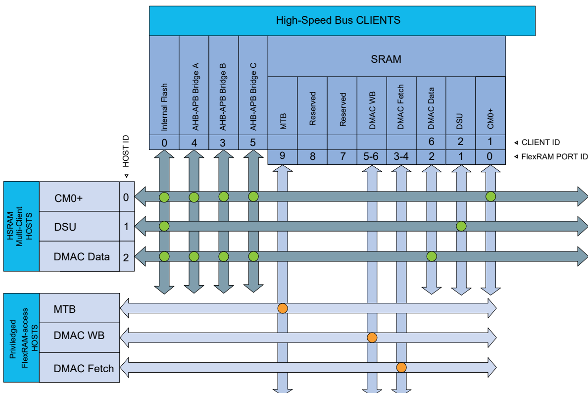
Figure 4-2. Host/Client Relation High-Speed Bus Matrix
