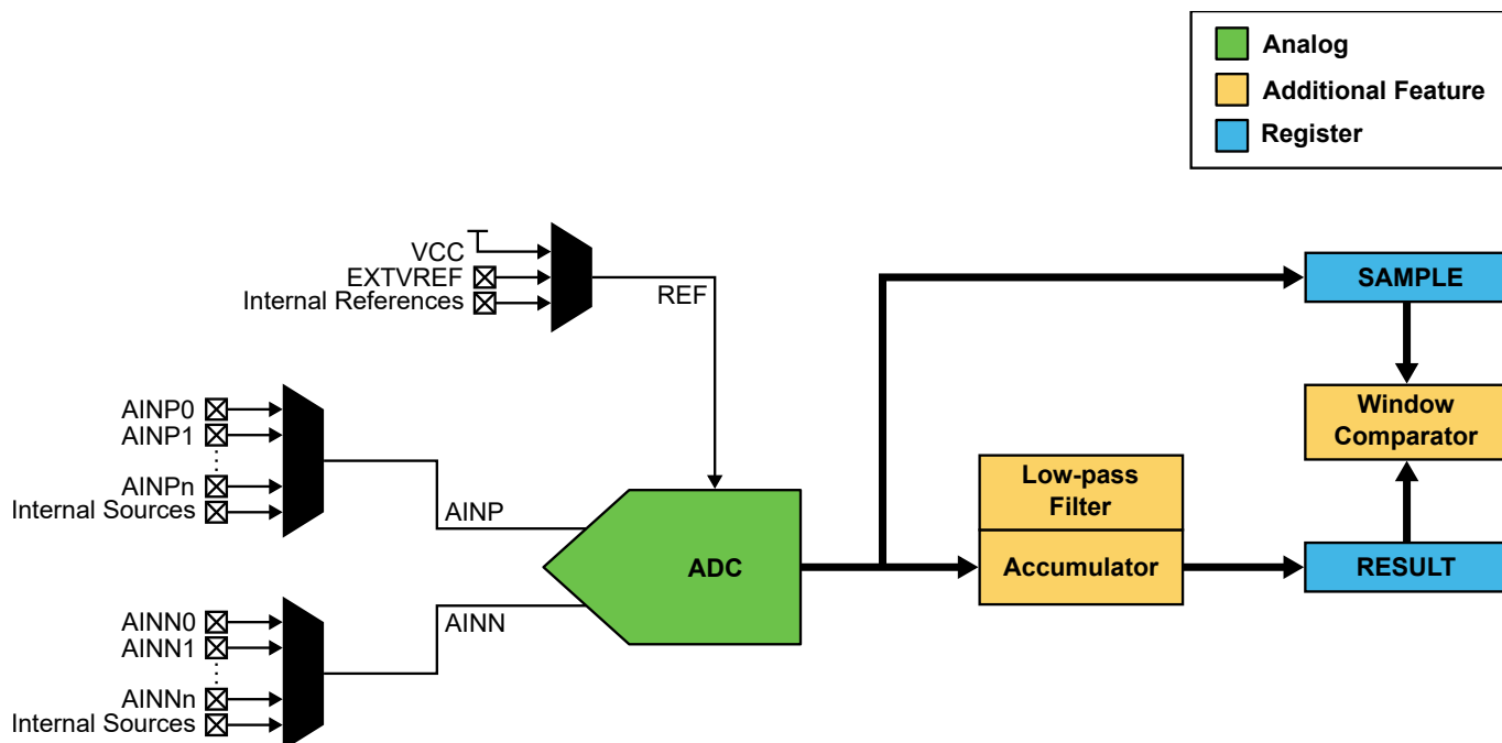
Figure 33-1. Block Diagram
