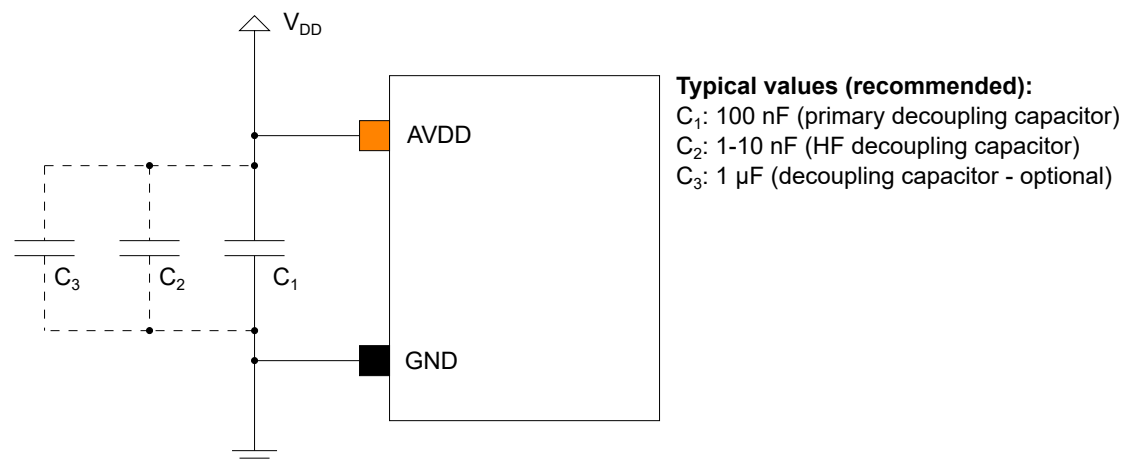
Figure 41-2. Recommended AVDD Connection Circuit Schematic
