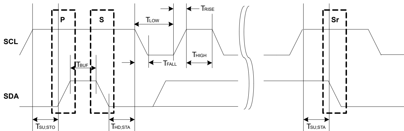
Figure 31-7. SCL Timing
