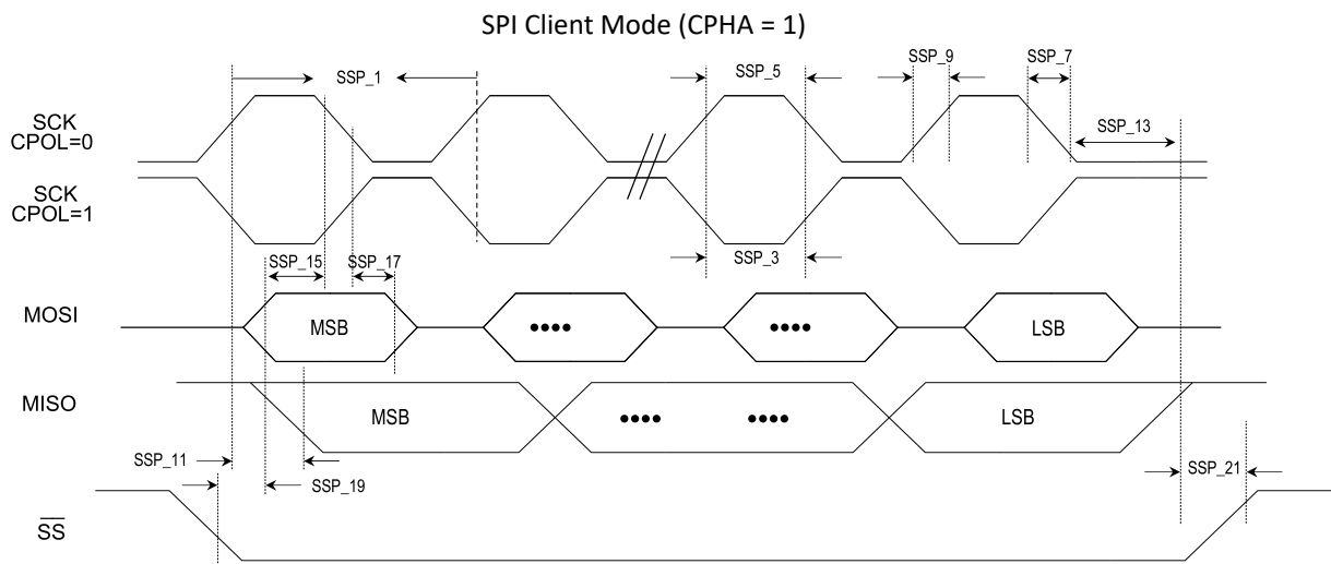
Figure 38-5. SERCOMn SPI Client Module (CPHA = 1) Timing Diagram
