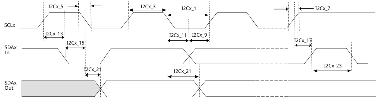
Figure 38-9. I 2 C Bus Data Client Mode Timing Diagrams
