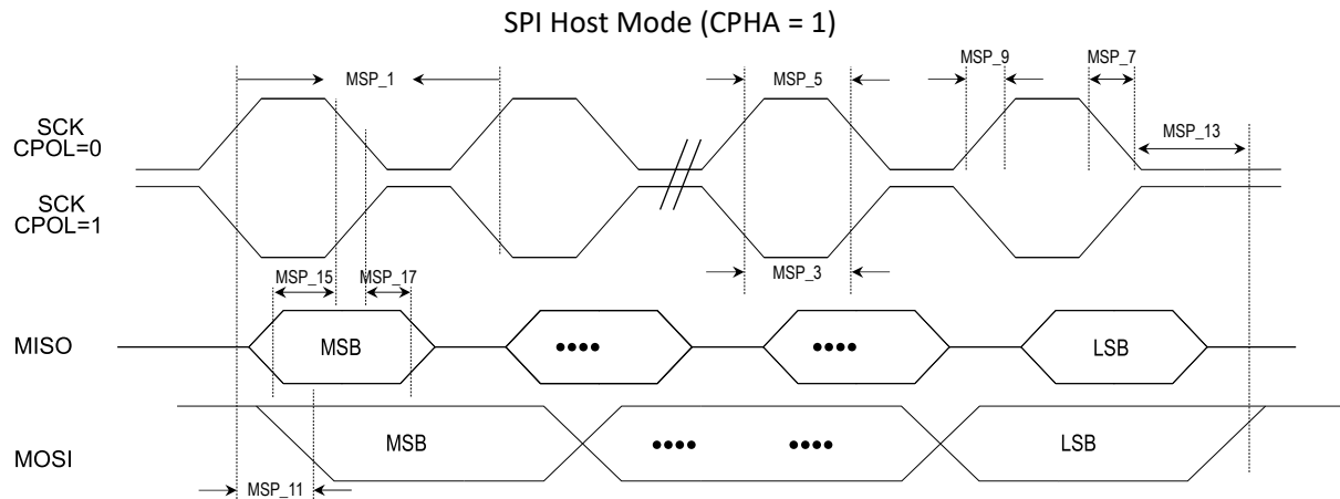
Figure 37-3. SERCOMn SPI Host Module CPHA=1 Timing Diagrams
