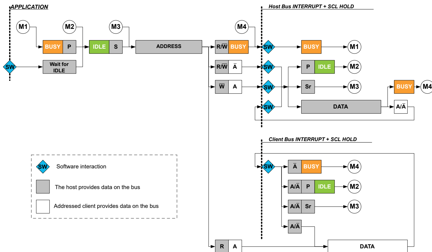
Figure 31-5. I 2 C Host Behavioral Diagram (SCLSM=0)
