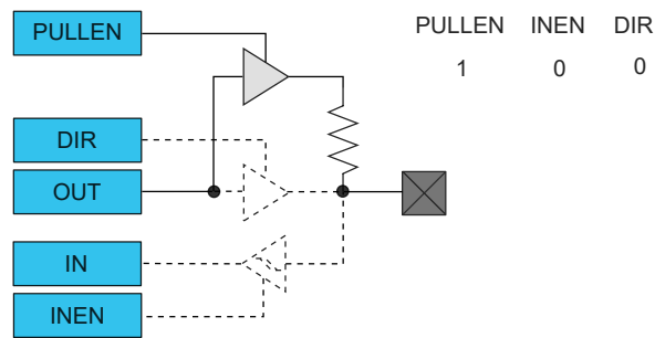
Figure 27-7. I/O Configuration - Output With Programmable Pull
