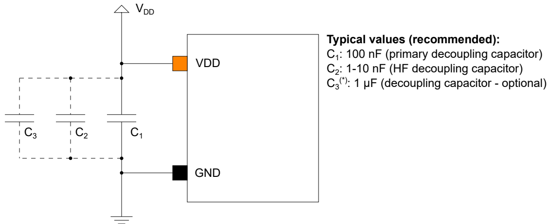
Figure 41-1. Recommended V_{DD} Connection Circuit Schematic
