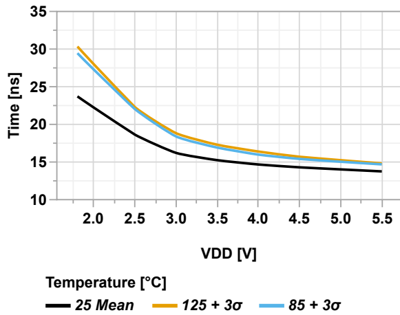
Figure 39-3. Rise Time vs. V_{DD} (SLEWLIM = b'0)
