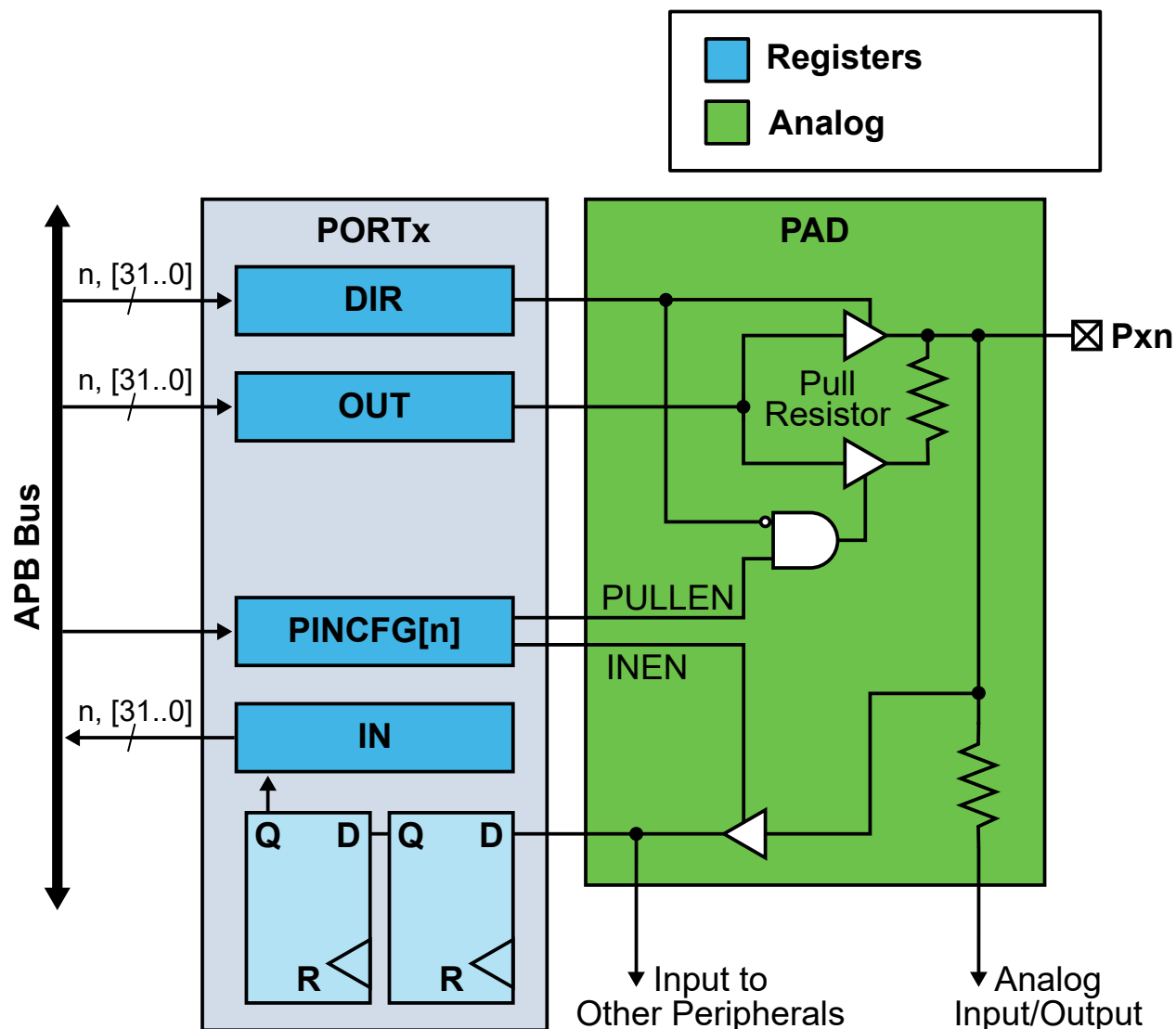
Figure 27-2. Overview of the PORT
