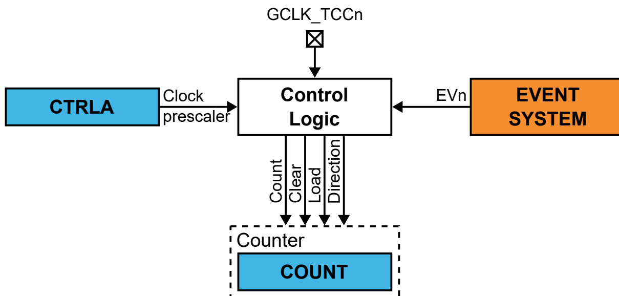
Figure 23-3. TCC - Counter Operation
