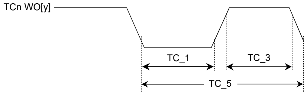
Figure 38-11. TCn Timer Compare Output Module Timing Diagram
