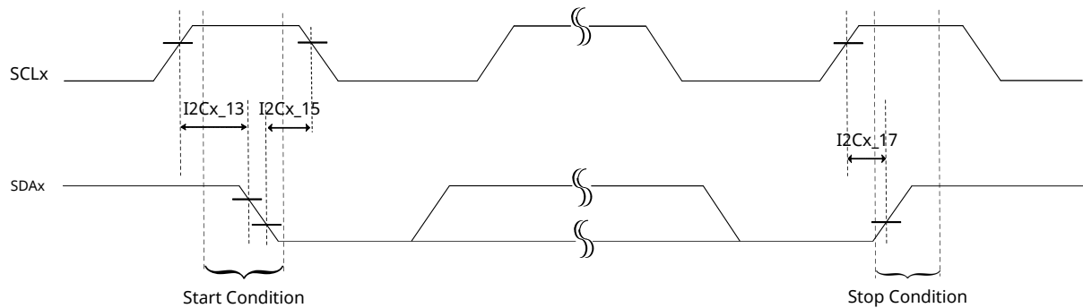
Figure 38-7. I 2 C Bus Data Host Mode Timing Diagrams
