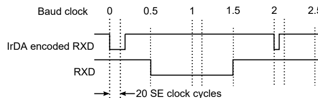
Figure 29-11. IrDA Receive Decoding
