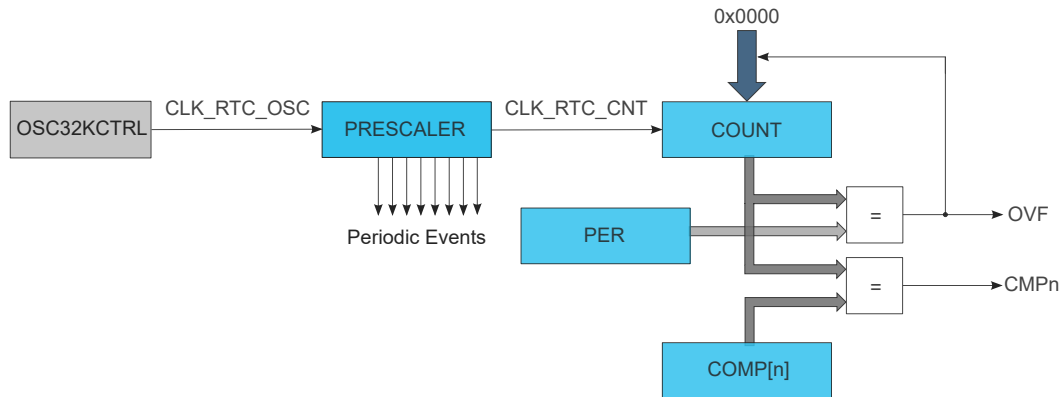
Figure 21-2. RTC Block Diagram (Mode 1 – 16-Bit Counter)
