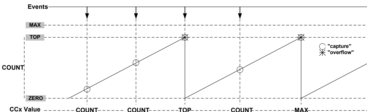
Figure 22-15. Time-Stamp
