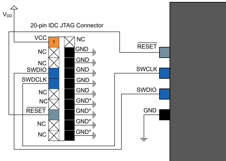
Figure 41-13. 20-pin IDC JTAG Connector
