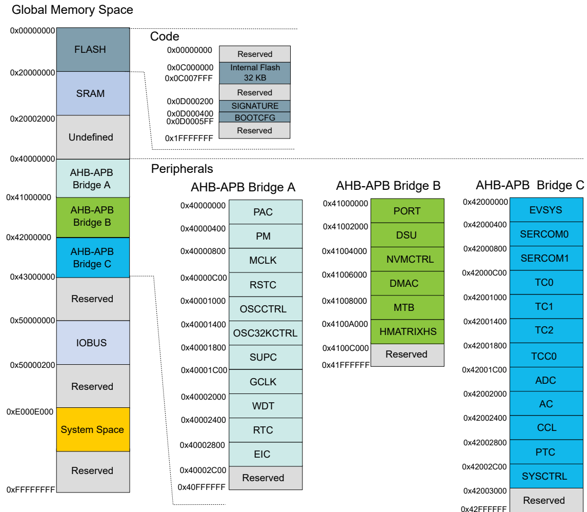
Figure 4-1. PIC32CM3204PL10 Product Mapping
