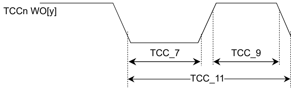
Figure 37-14. TCCn Timer Compare Fault Output Module Timing Diagrams
