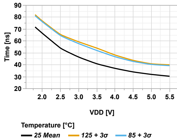
Figure 39-4. Rise Time vs. V_{DD} (SLEWLIM = b'1)
