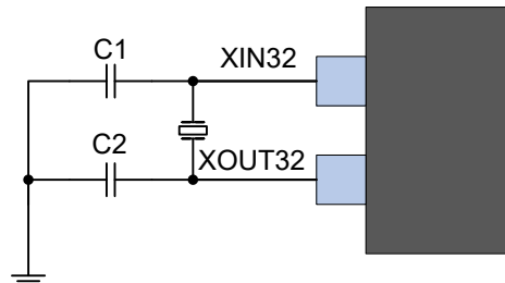
Figure 41-10. 32.768 kHz Crystal Oscillator Schematics
