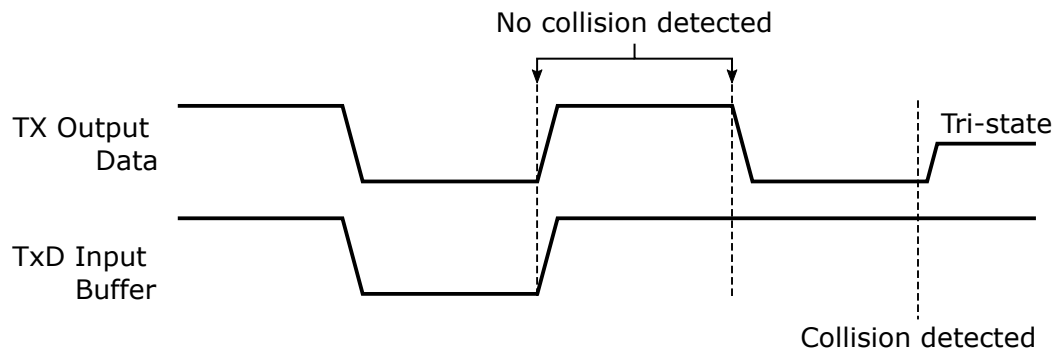
Figure 29-18. Collision Detected
