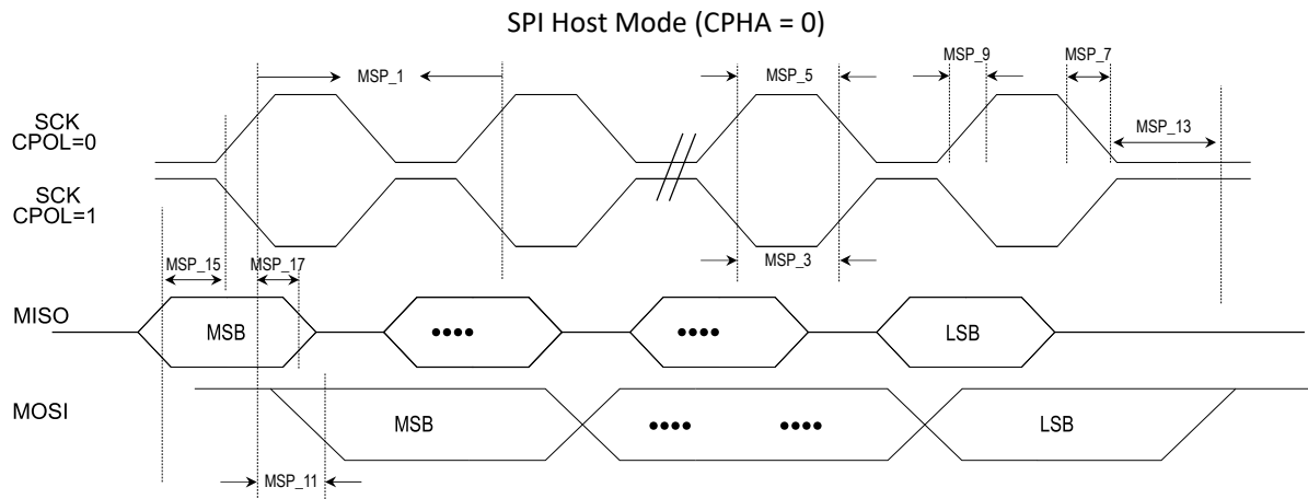
Figure 38-2. SERCOMn SPI Host Module CPHA = 0 Timing Diagrams
