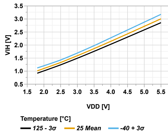
Figure 39-6. Input Pin with Schmitt Trigger - Minimum V_{IH} vs. V_{DD}
