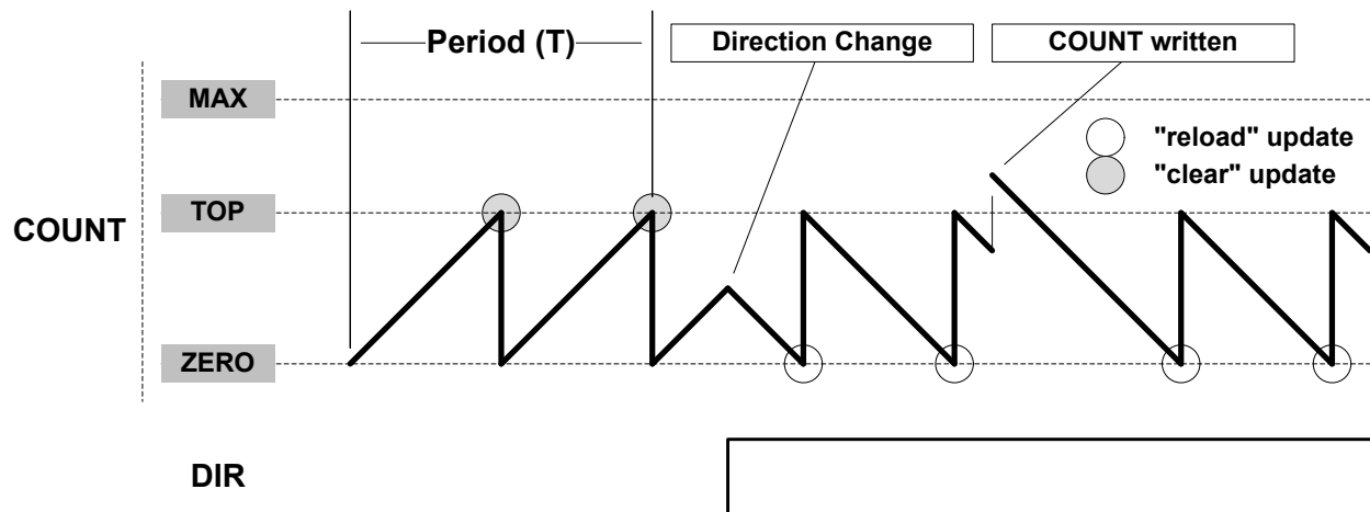
Figure 22-3. Counter Operation
