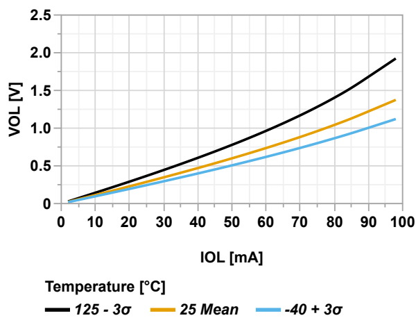
Figure 39-14. Output Pin - Maximum V_{OL} vs. Current, V_{DD} = 5.5V
