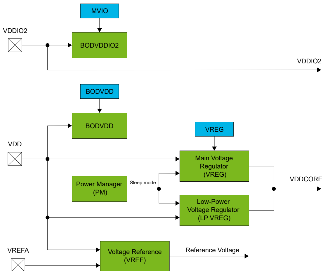
Figure 15-1. SUPC Block Diagram
