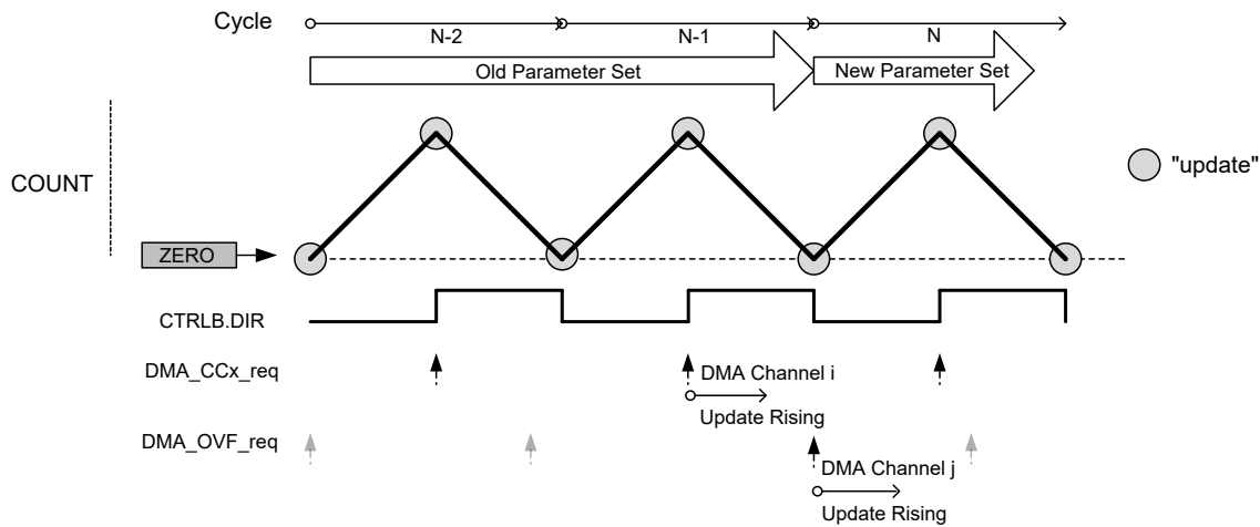
Figure 23-38. DMA Triggers in DSBOOTH Operation Mode and Circular Buffer Enabled
