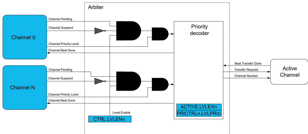
Figure 19-4. Arbiter Overview
