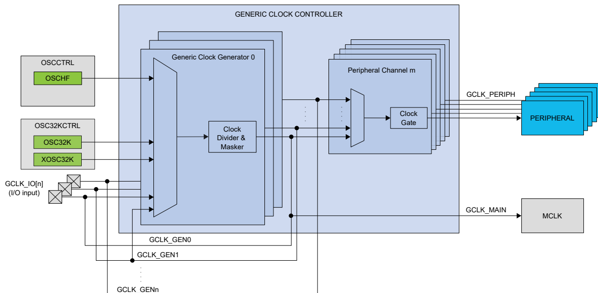
Figure 10-1. Device Clocking Diagram
