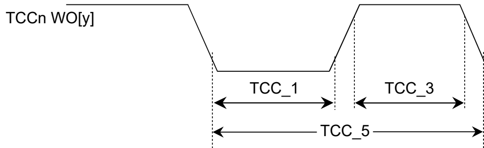
Figure 37-13. TCCn Timer Compare Output Module Timing Diagrams
