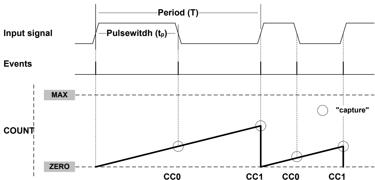
Figure 22-13. PWP Capture
