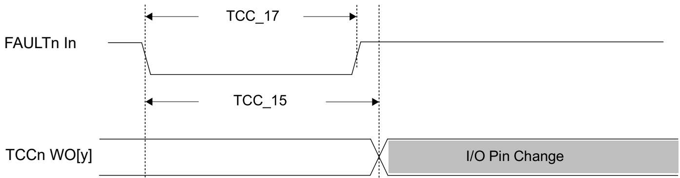
Figure 37-14. TCCn Timer Compare Fault Output Module Timing Diagrams
