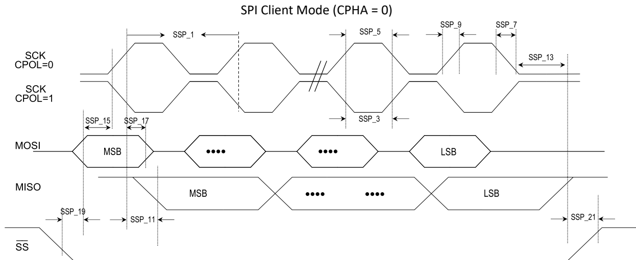
Figure 38-4. SERCOMn SPI Client Module (CPHA = 0) Timing Diagram
