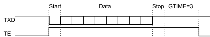
Figure 29-16. Example of TE Drive With Guard Time
