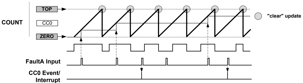
Figure 23-30. Capture Action "DERIVO"
