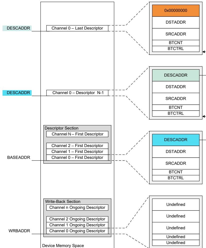
Figure 19-3. Memory Sections
