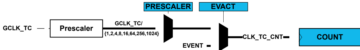
Figure 22-2. Prescaler
