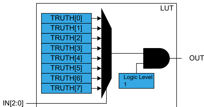
Figure 32-2. Truth Table Output Value Selection
