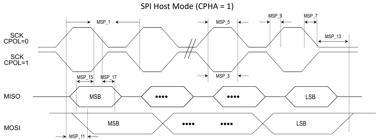
Figure 38-3. SERCOMn SPI Host Module CPHA = 1 Timing Diagrams
