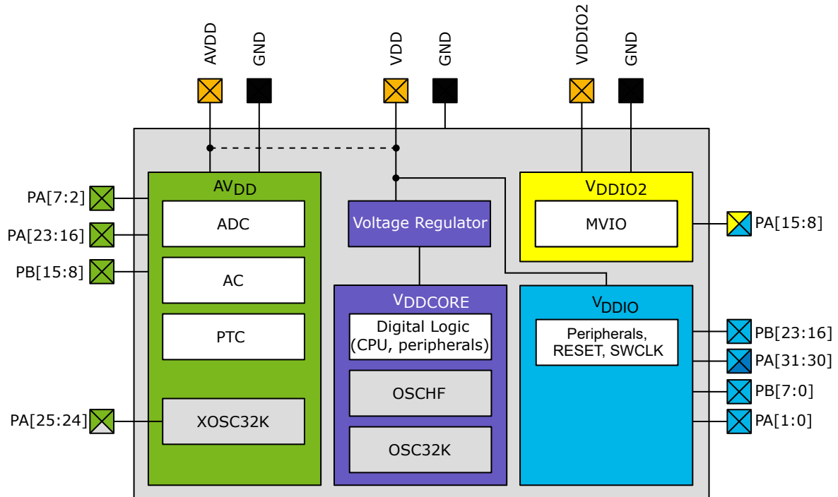
Figure 3-1. Power Domains of the PIC32CM PL10 Family
