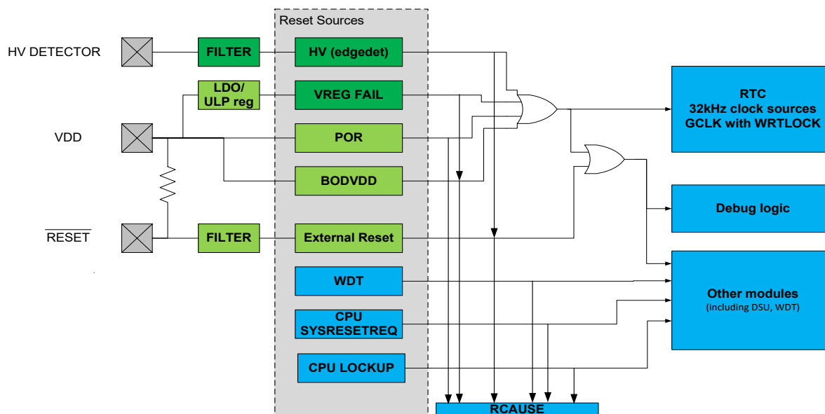
Figure 16-1. Reset System
