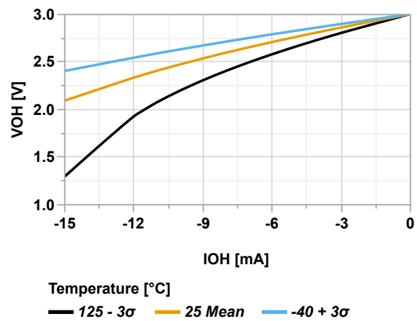
Figure 39-15. Output Pin - Minimum V_{OH} vs. Current, V_{DD} = 5.5V
