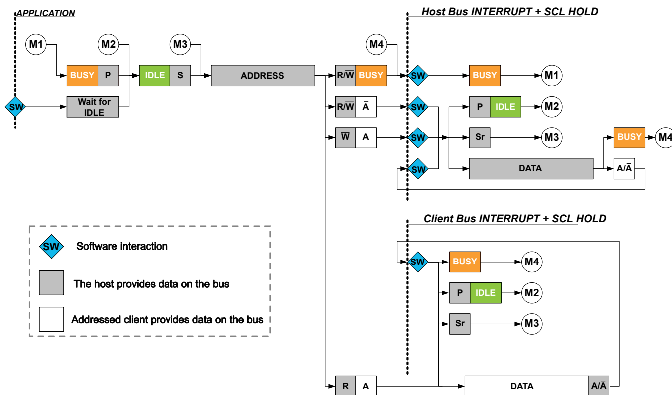
Figure 31-6. I 2 C Host Behavioral Diagram (SCLSM=1)
