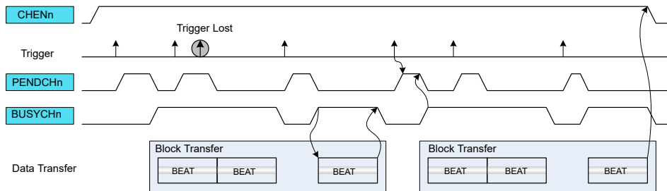
Figure 19-7. Trigger Action and Transfers
