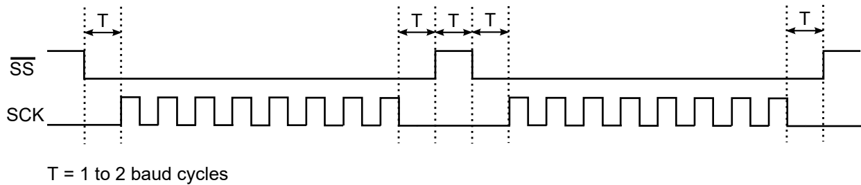
Figure 30-7. Hardware Controlled \overline{SS}
