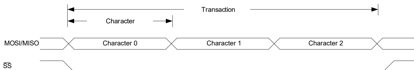
Figure 30-2. SPI Transaction Format
