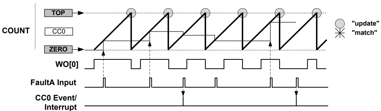
Figure 23-30. Capture Action "DERIVO"
