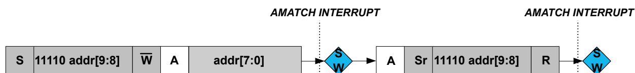
Figure 31-11. 10-bit Addressing
