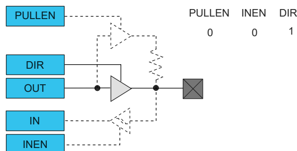
Figure 27-5. I/O Configuration - Totem Pole Output With Disabled Input
