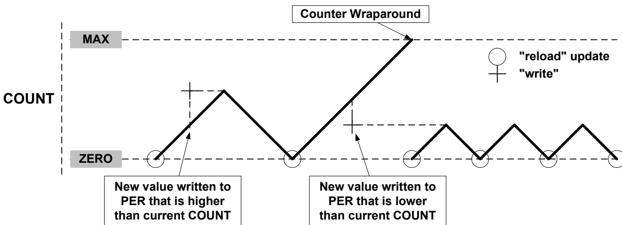
Figure 23-13. Unbuffered Dual-Slope Operation
