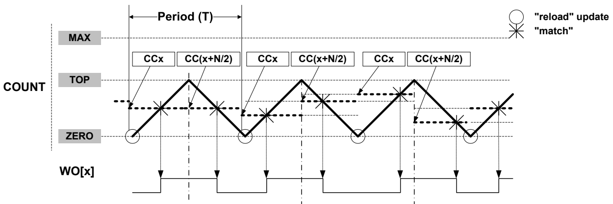
Figure 23-9. Dual-Slope Critical Pulse Width Modulation (N=CC_NUM)
