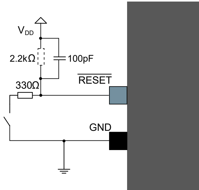
Figure 41-6. External Reset Circuit Schematic (EFT Immunity Enhancement) (2)
