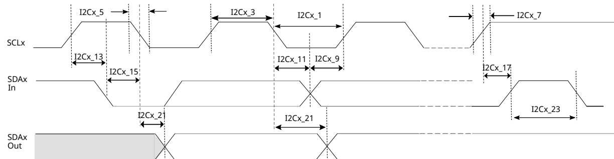
Figure 38-7. I 2 C Bus Data Host Mode Timing Diagrams
