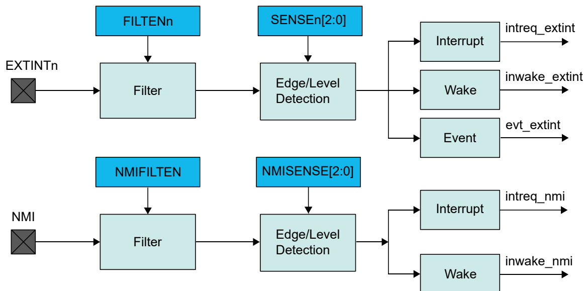
Figure 25-1. EIC Block Diagram
