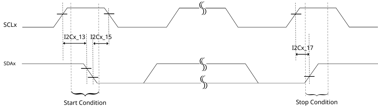
Figure 37-9. I 2 C Bus Data Client Mode Timing Diagrams
