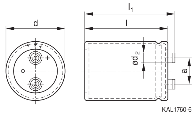
Ring clip/clamp mounting
