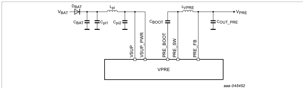
Figure 18. Input topology: direct VSUP connection
