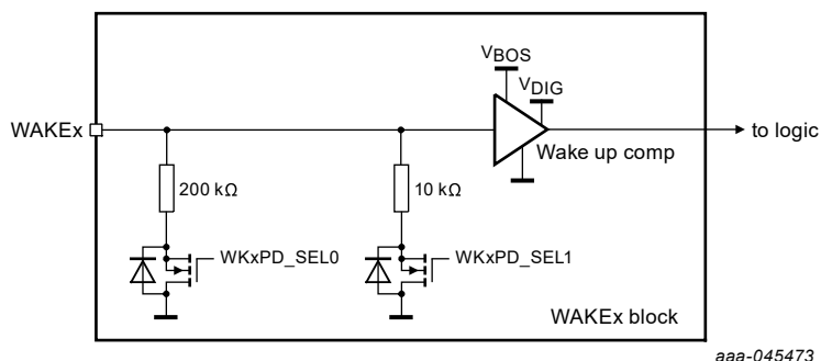
Figure 39. WAKEx pin block diagram
