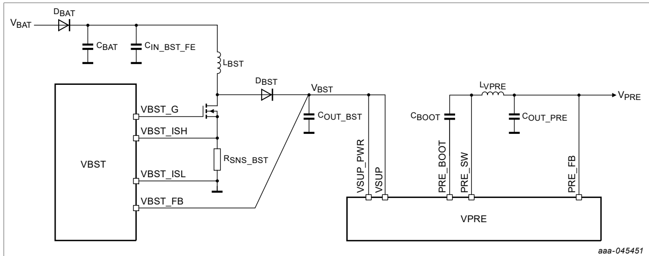
Figure 17. Input topology: front-end boost controller
