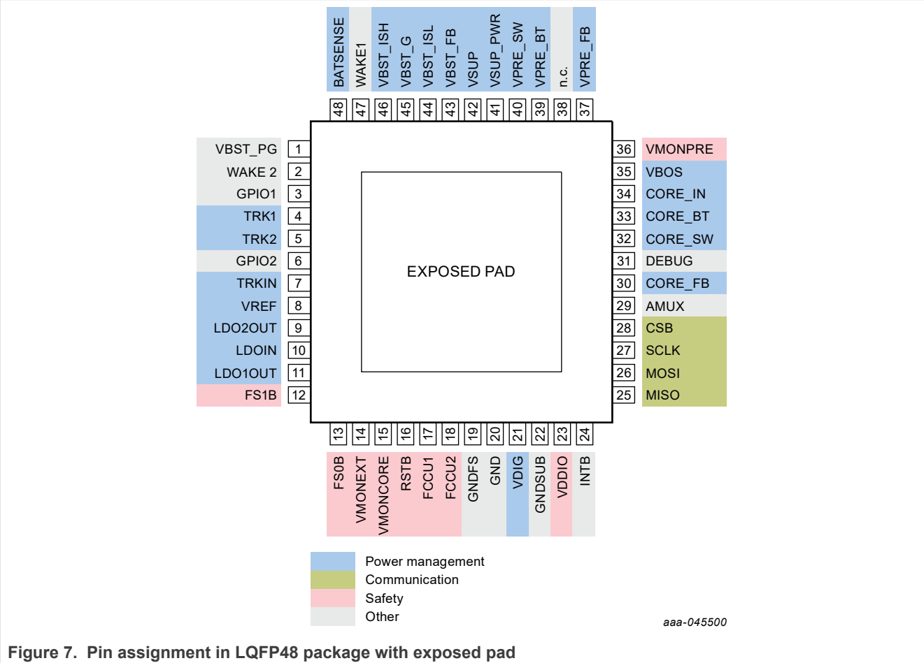
Figure 7. Pin assignment in LQFP48 package with exposed pad
