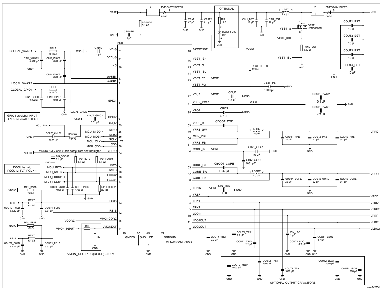
Figure 54. Application schematic in front-end configuration for F_{PRE} = 450 kHz
