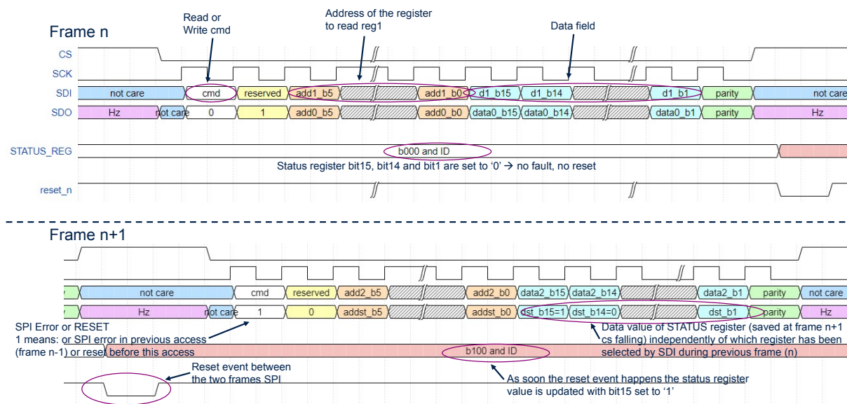
Figure 32. Access after RESET scenario
