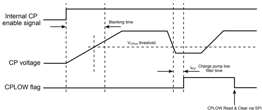
Figure 13. CPLOW flag
