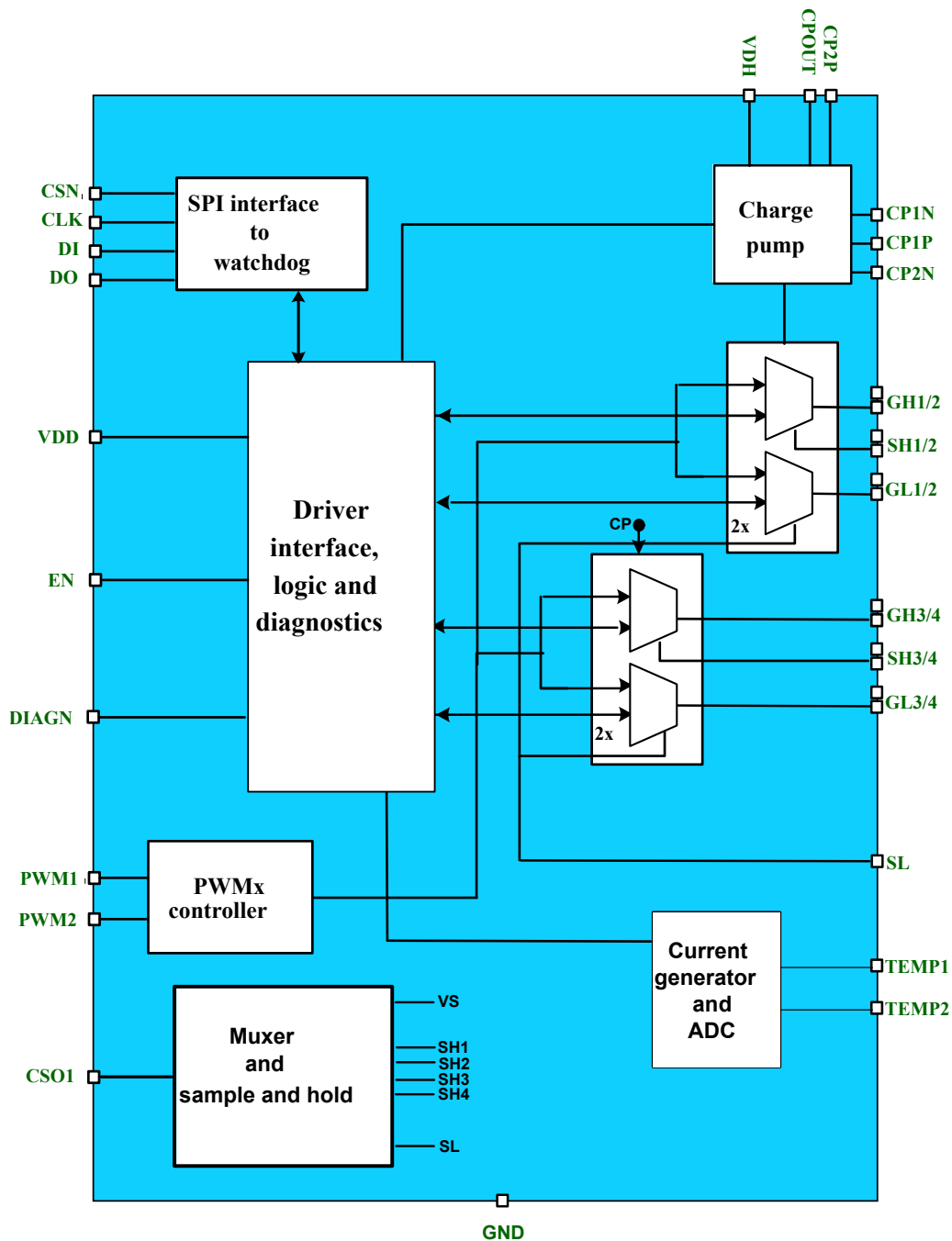
Figure 1. STDRIVE141 block diagram
