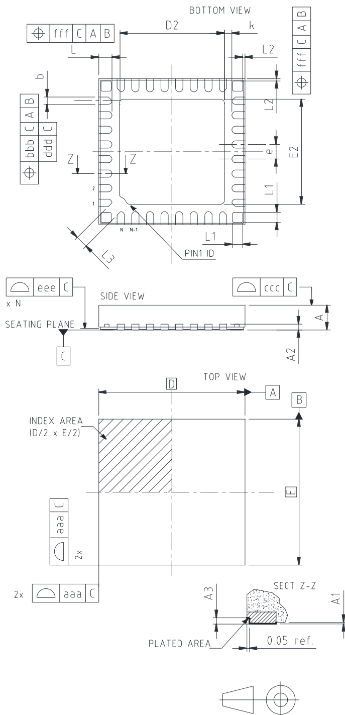
Figure 40. VFQFN32L (5x6x0.9 mm exp. pad down) package outline
