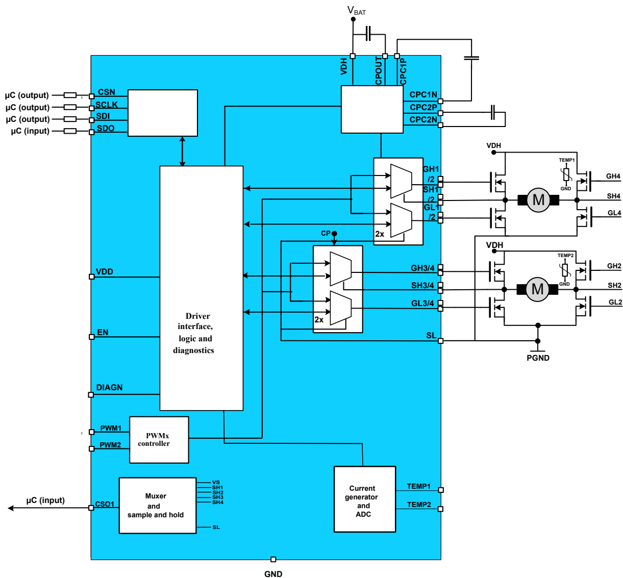
Figure 39. Driving 2 DC motors simultaneously with not sequentially gate drivers (STDRIVE141)
