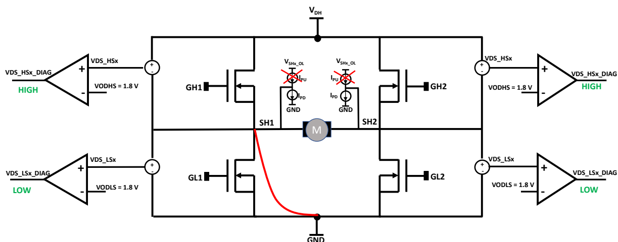
Figure 22. Short circuit to GND
