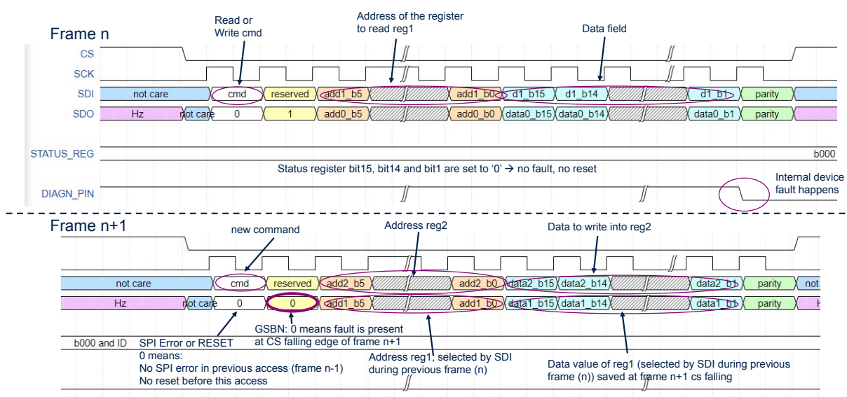
Figure 34. Access while an internal fault happens scenario
