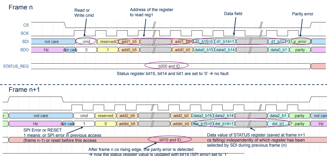
Figure 31. Write or read with SPI error scenario
