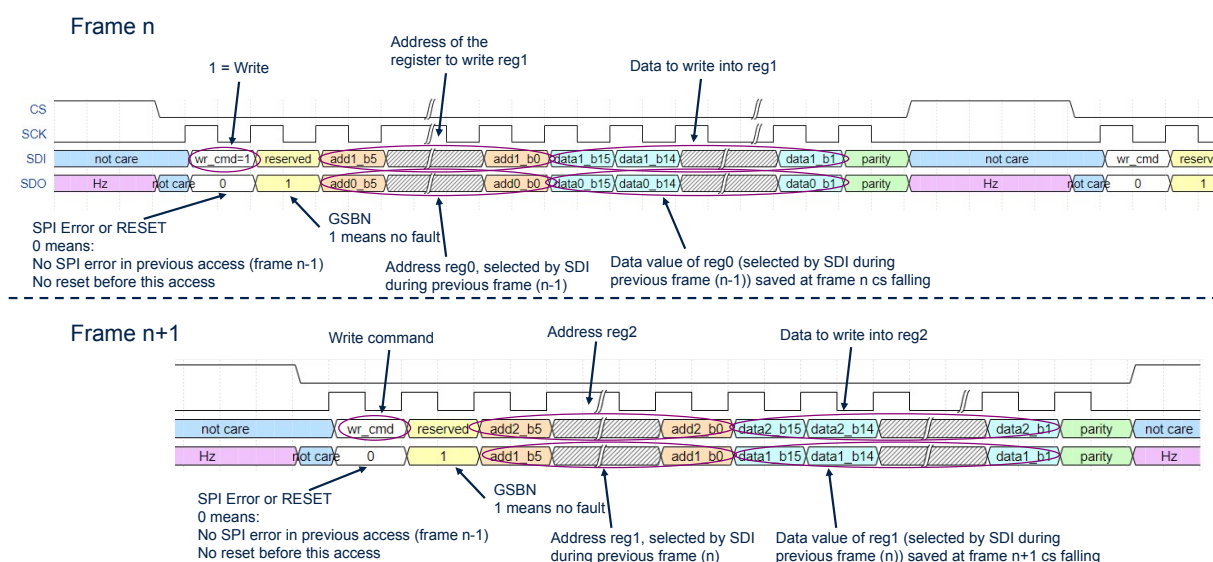
Figure 28. Write access scenario
