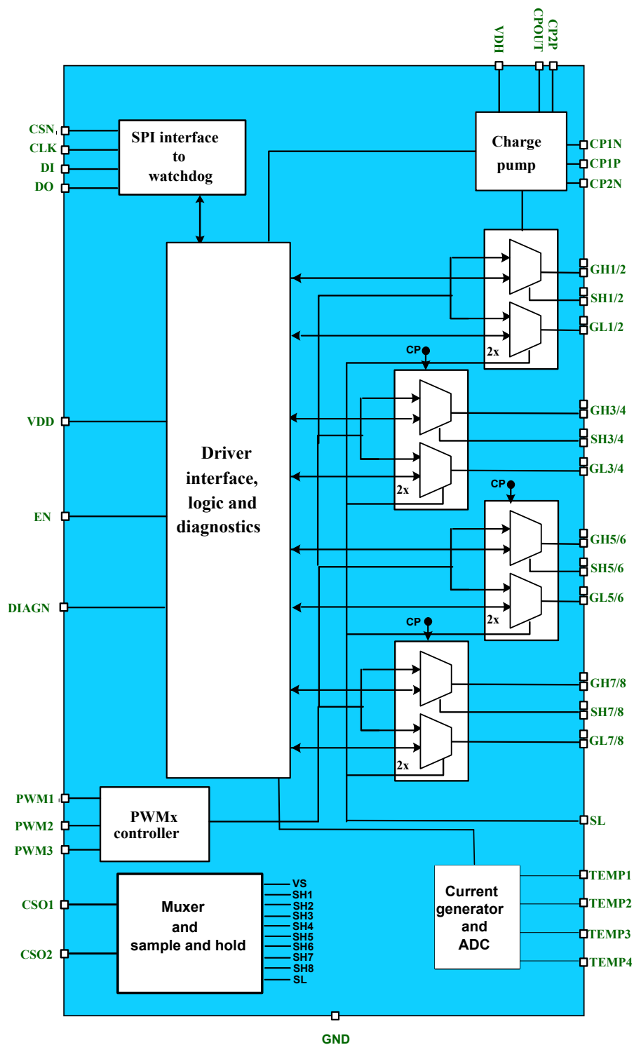
Figure 1. Block diagram
