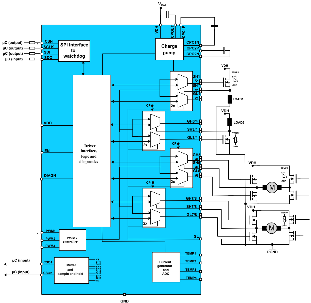
Figure 36. Driving 2 DC motors + 2 additional independent loads simultaneously
