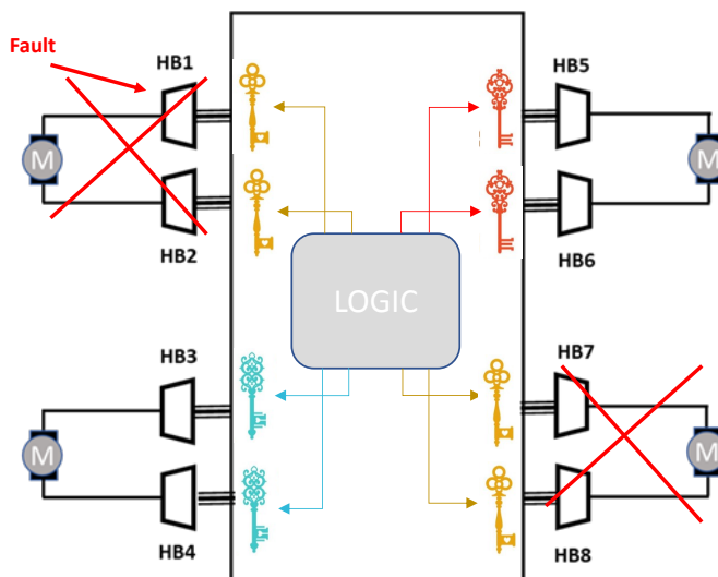
Figure 7. Example of fault on HB1
