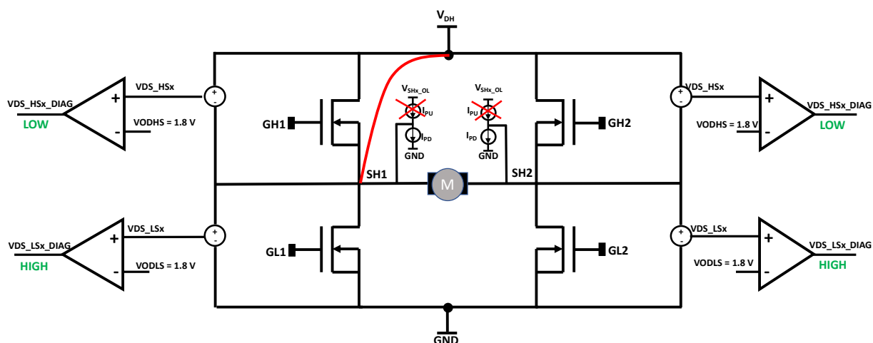
Figure 21. Short circuit to V_{DH}
