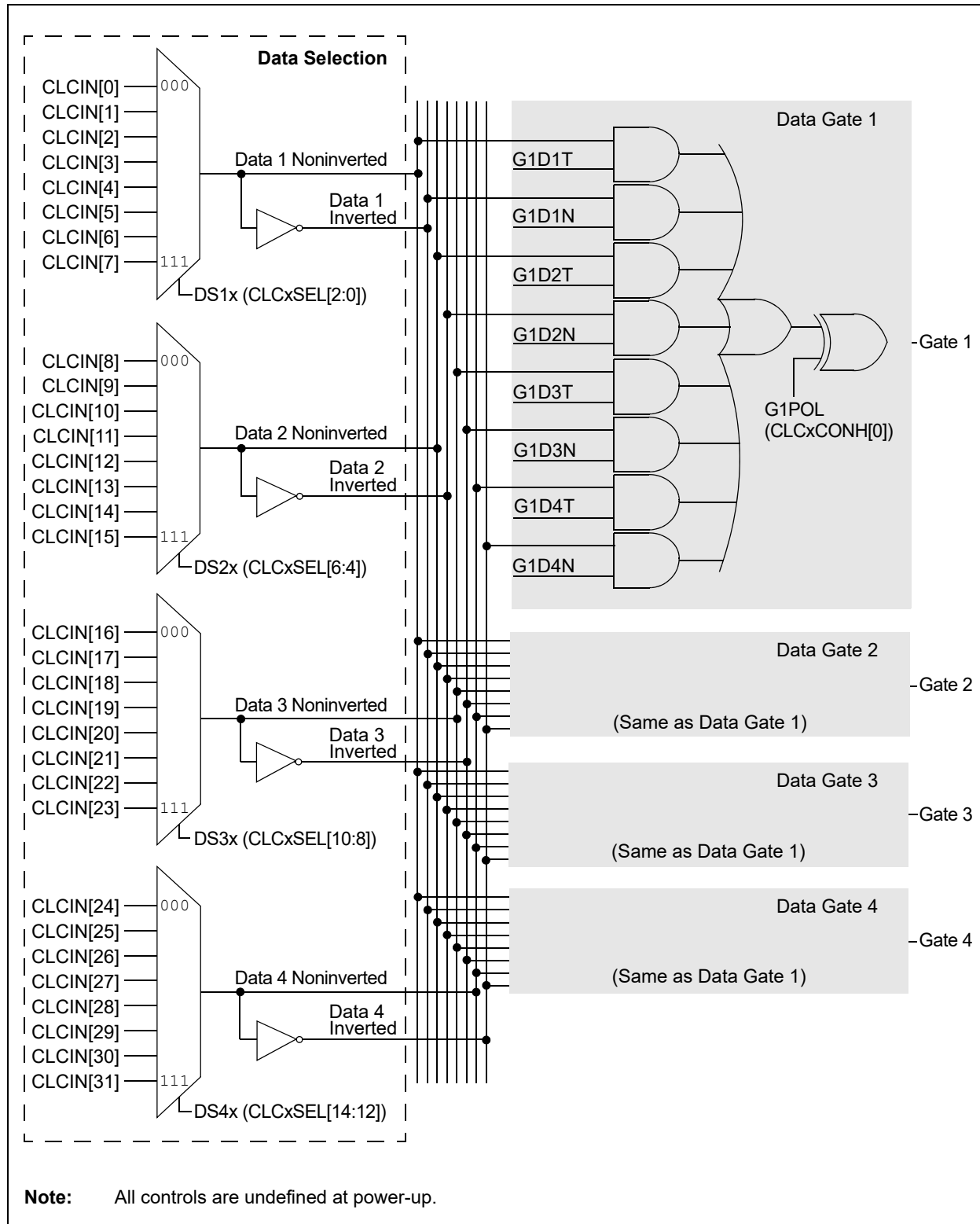
FIGURE 24-3: CLCx INPUT SOURCE SELECTION DIAGRAM
