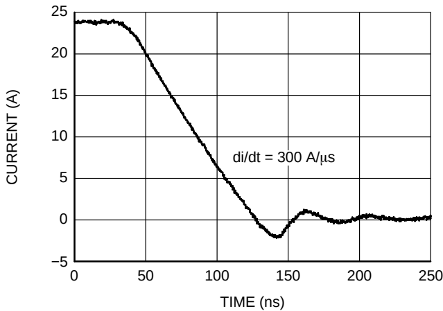
Figure 14. FDMS0308AS SyncFET Body Diode Reverse Recovery Characteristic
