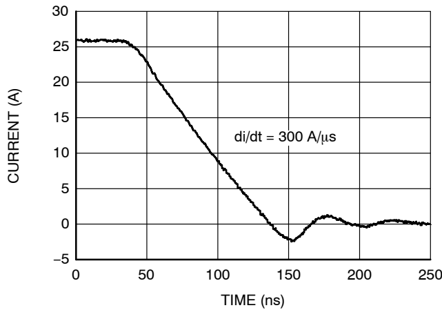
Figure 14. FDMS8023S SyncFET Body Diode Reverse Recovery Characteristic
