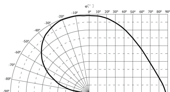
Radiation Characteristics
