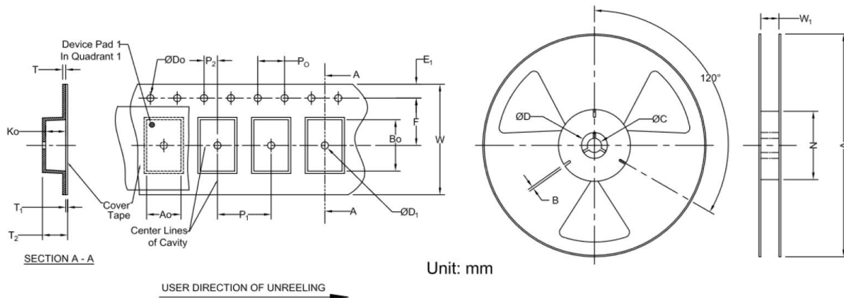
Carrier Tape Specifications (mm)
