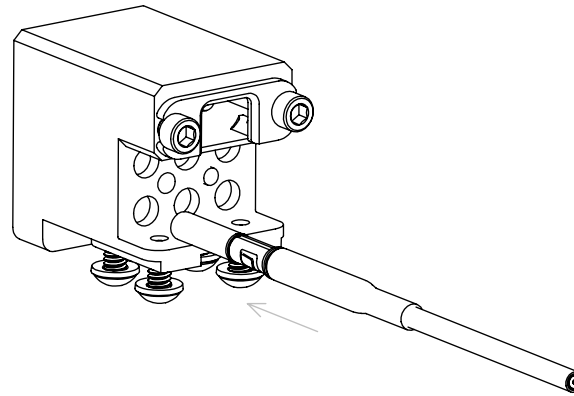
CONTACT INSERTION - STEP 1 ALIGN MALE (SOCKET) CONTACT WITH REAR RF PORT
