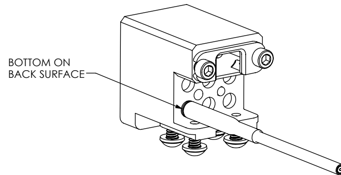
CONTACT INSERTION - STEP 1 ALIGN MALE (SOCKET) CONTACT WITH REAR RF PORT
