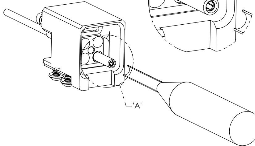
CONTACT REMOVAL - STEP 2 INSERT REMOVAL TOOL IN GAP BETWEEN CONTACT AND HOUSING. INSERT UNTIL BOTTOMED.
