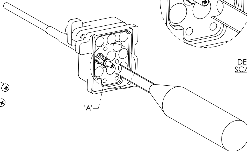
CONTACT REMOVAL - STEP 2 INSERT REMOVAL TOOL IN GAP BETWEEN CONTACT AND HOUSING. INSERT UNTIL BOTTOMED.
