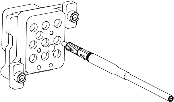
CONTACT INSERTION - STEP 1 ALIGN FEMALE (PIN) CONTACT WITH REAR RF PORT
