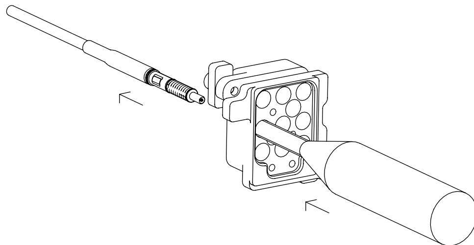
CONTACT REMOVAL - STEP 3 WITH REMOVAL TOOL INSERTED FULLY, GENTLY PULL ON CONTACT CABLE UNTIL REMOVED.
