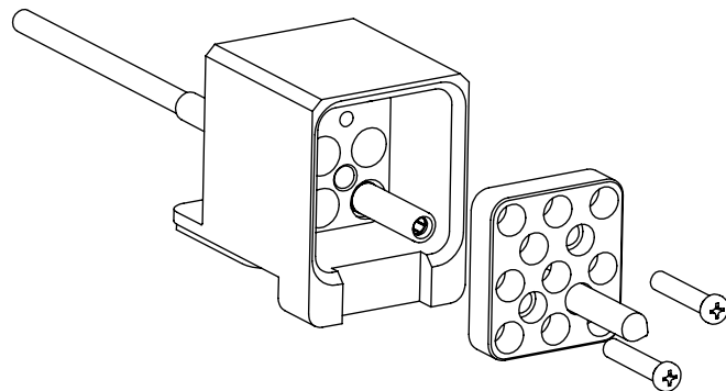
CONTACT REMOVAL - STEP 1 REMOVE FRONT PLATE AND SCREWS USING PH000 DRIVER.
