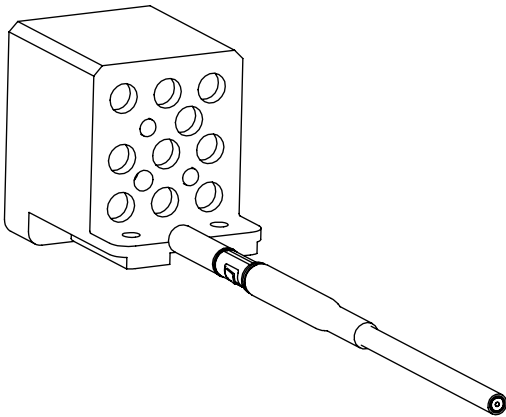
CONTACT INSERTION - STEP 1 ALIGN MALE (SOCKET) CONTACT WITH REAR RF PORT.
