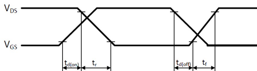
Figure 1-20. Switching Waveform
