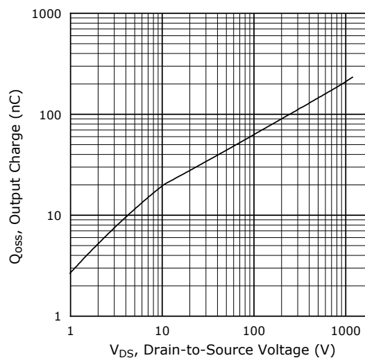
Figure 1-12. Q_{oss} vs. Drain-to-Source Voltage
