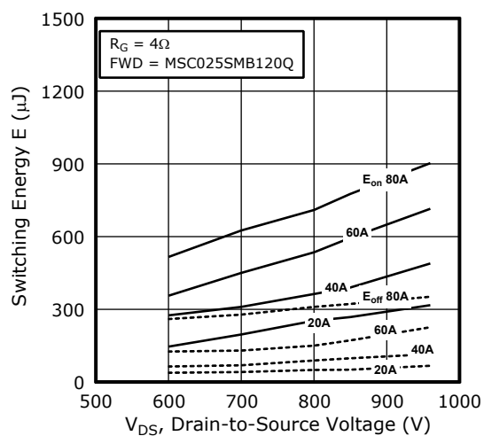
Figure 1-15. Switching Energy vs. V_{DS} & I_D
