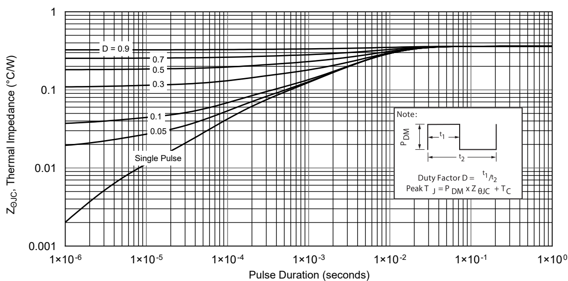
Figure 1-19. Maximum Transient Thermal Impedance
