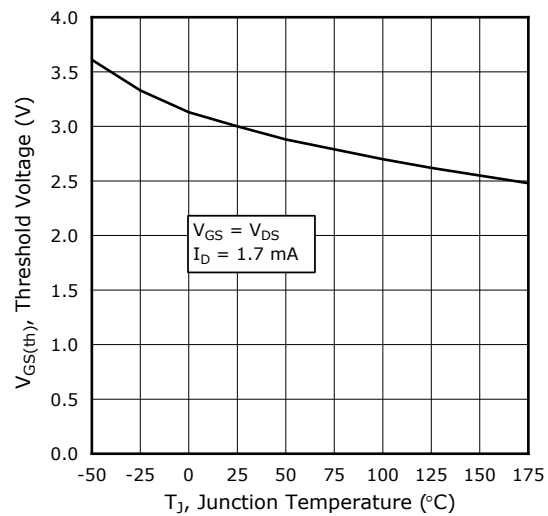
Figure 1-8. Threshold Voltage vs. Junction Temperature
