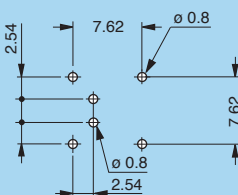
P11 - EPG-EXG (0B/1B.302) Solder mount
