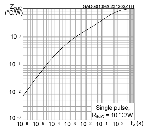
Figure 17. Maximum transient thermal impedance
