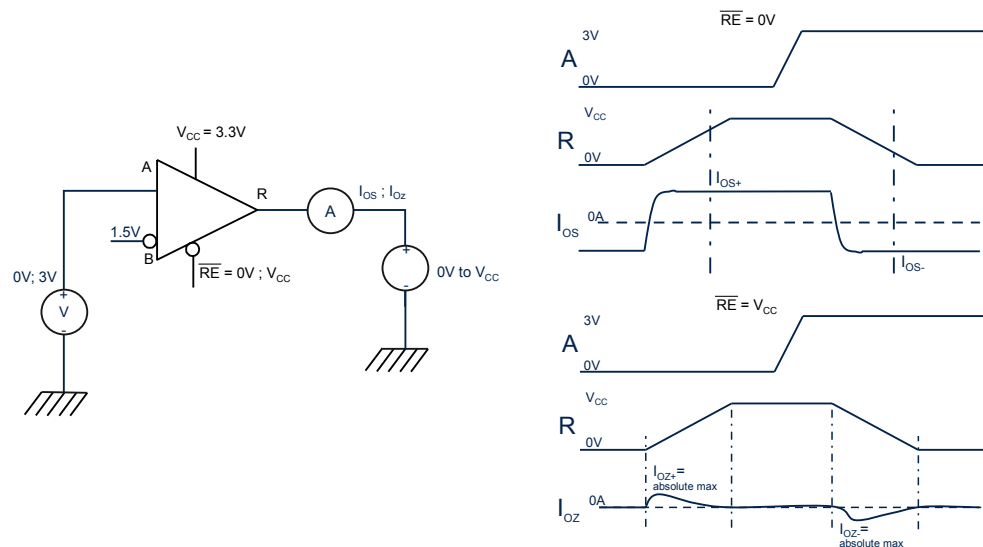
Figure 11. Receiver output current
