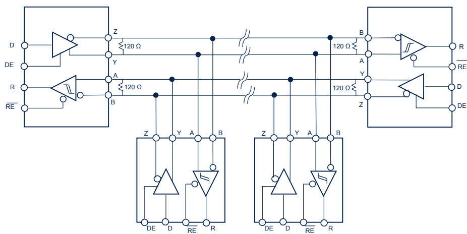
Figure 14. Typical full-duplex RS485 network
