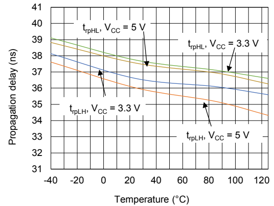
Figure 32. Receiver propagation delay vs. temperature, with C_L = 20\text{ pF}
