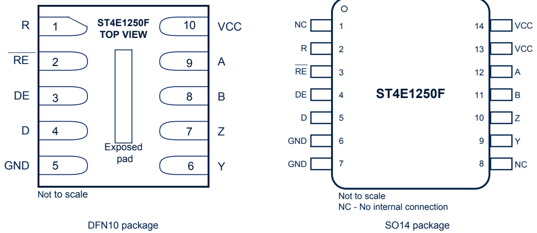
Figure 1. Pin connections
