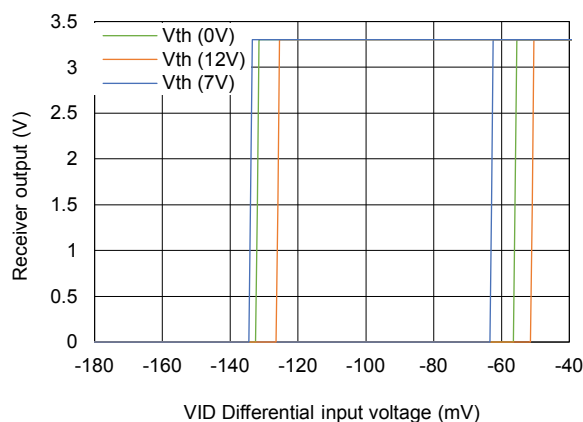
Figure 20. Receiver output vs. input @ V_{CC} = 3.3\text{ V}
