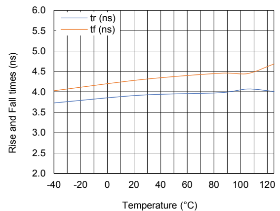
Figure 28. Driver rise and fall times vs. temperature @ V CC = 3.3 V
