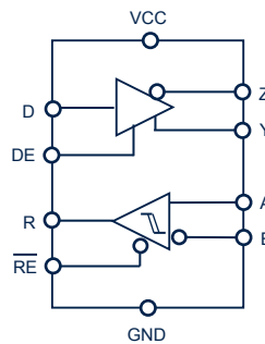
Figure 35. Block diagram
