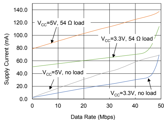
Figure 22. Supply current vs. data rate
