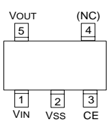
SOT-25 (SOT-23-5) [TOP VIEW]
