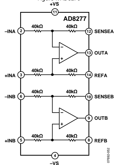
Figure 2. AD8277
